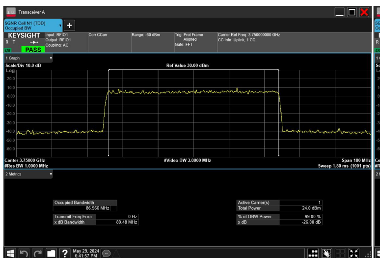
90MHz_30kHz_3750MHz_DFT-s-OFDM 16 QAM_RB243@0
