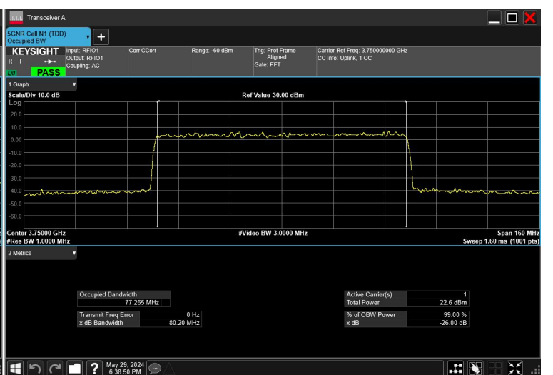
80MHz_30kHz_3750MHz_CP-OFDM 64 QAM_RB17@0
