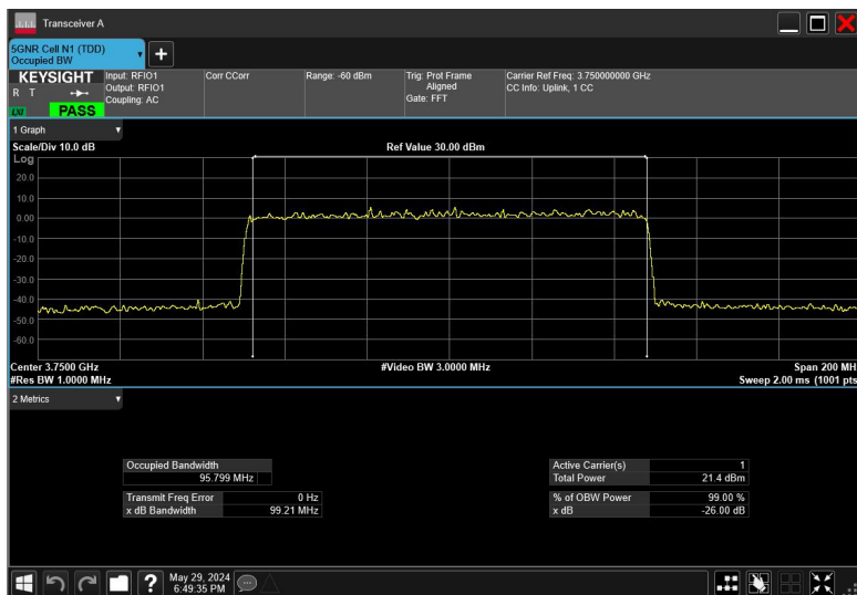
100MHz_30kHz_3750MHz_DFT-s-OFDM 256 QAM_RB270@0
