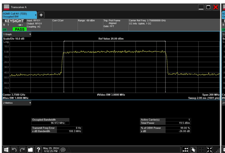
100MHz_30kHz_3750MHz_CP-OFDM 256 QAM_RB273@0
