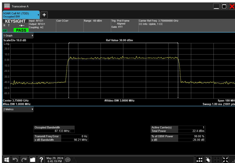
90MHz_30kHz_3750MHz_CP-OFDM 64 QAM_RB245@0
