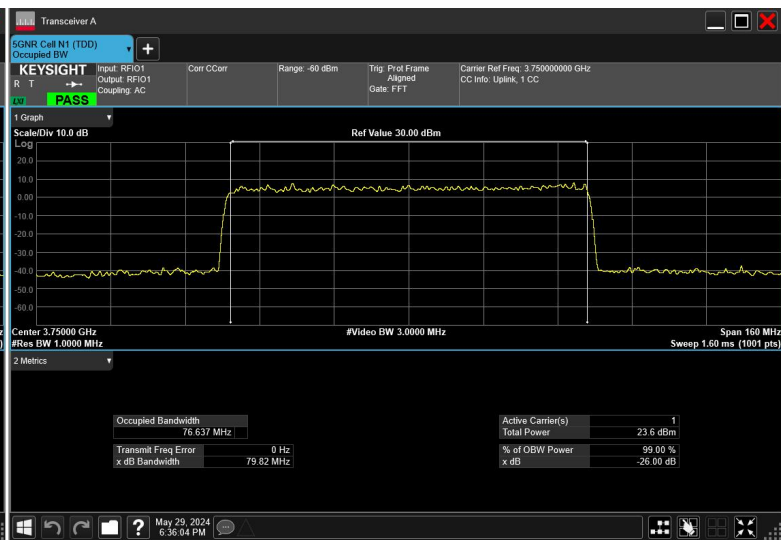
80MHz_30kHz_3750MHz_DFT-s-OFDM 64 QAM_RB216@0
