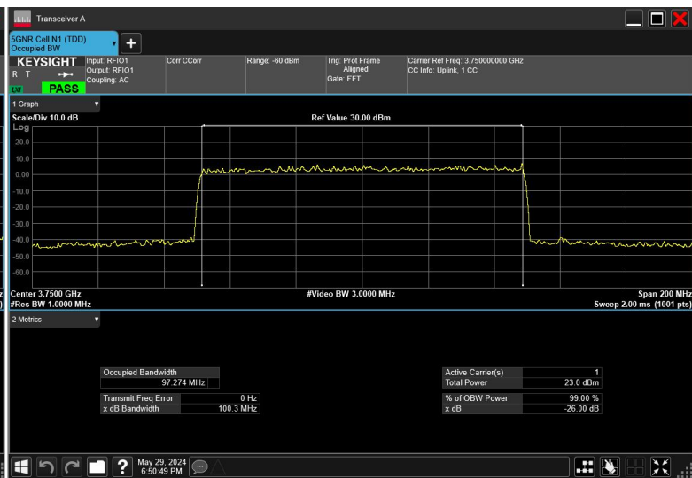
100MHz_30kHz_3750MHz_CP-OFDM 16 QAM_RB273@0
