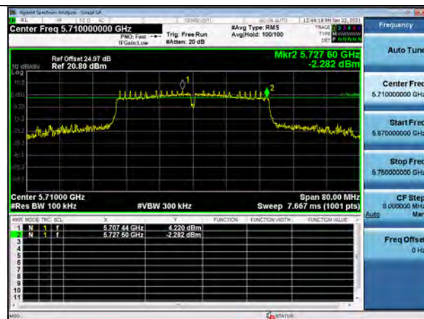
802.11ac_VHT40 CH.142
