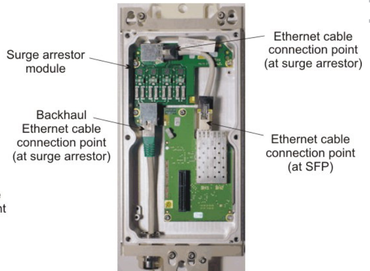
Electrical Backhaul Ethernet cable connection (with surge arrestor module)
