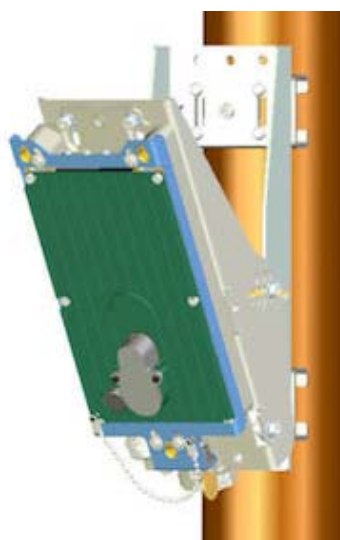
Figure 3-2 9764 Metro Dock pole mount using screws
