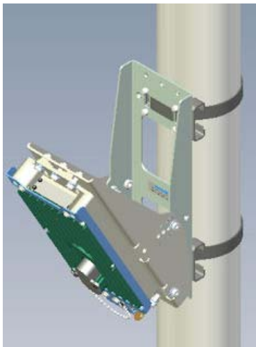
Pole mount - with tilt
