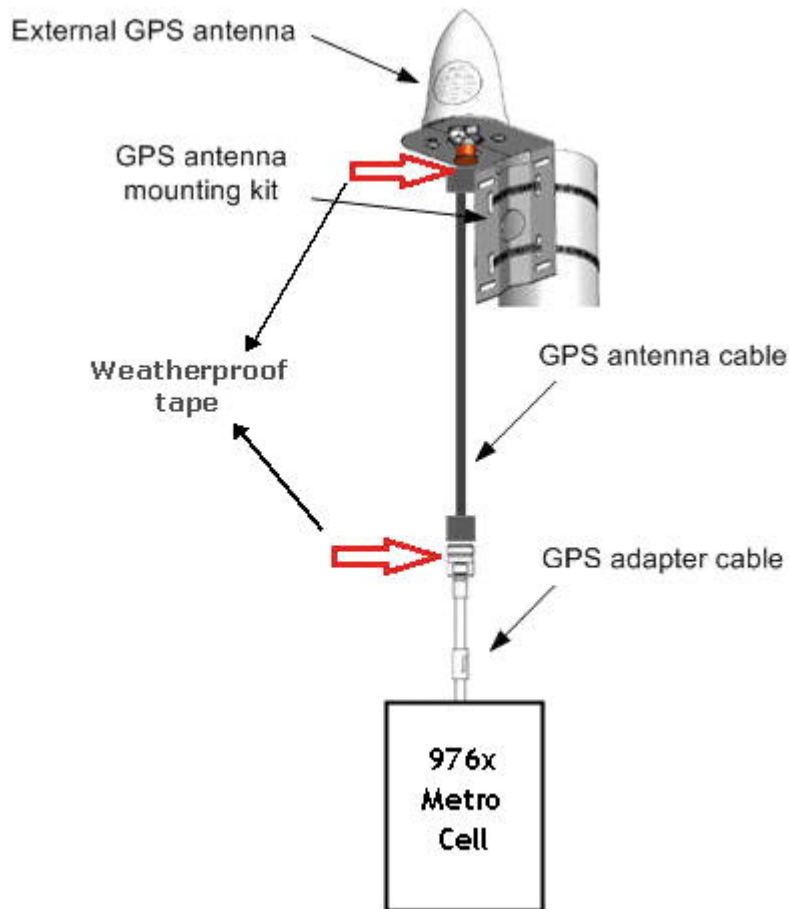
Figure 4-7 Weatherproof tape placement for external GPS antenna
