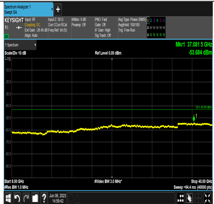
Band48-20MHz-256QAM-56640-E-TM3.1A-30~3530
