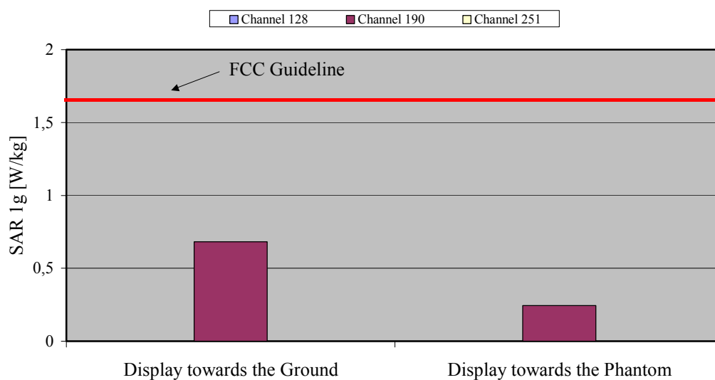
Fig. 11: The measured SAR values in body-worn configuration for GSM 850 for the Alcatel One Touch 331a, with 1.5 cm distance between mobile and phantom, in comparison to the FCC exposure limit.
