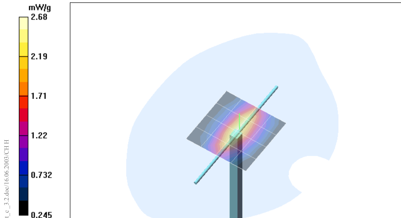
Fig. 15: Validation measurement 850 MHz body (October 07, 2003), coarse grid. Ambient Temperature: 20.8° C, Liquid Temperature: 20.3° C.
