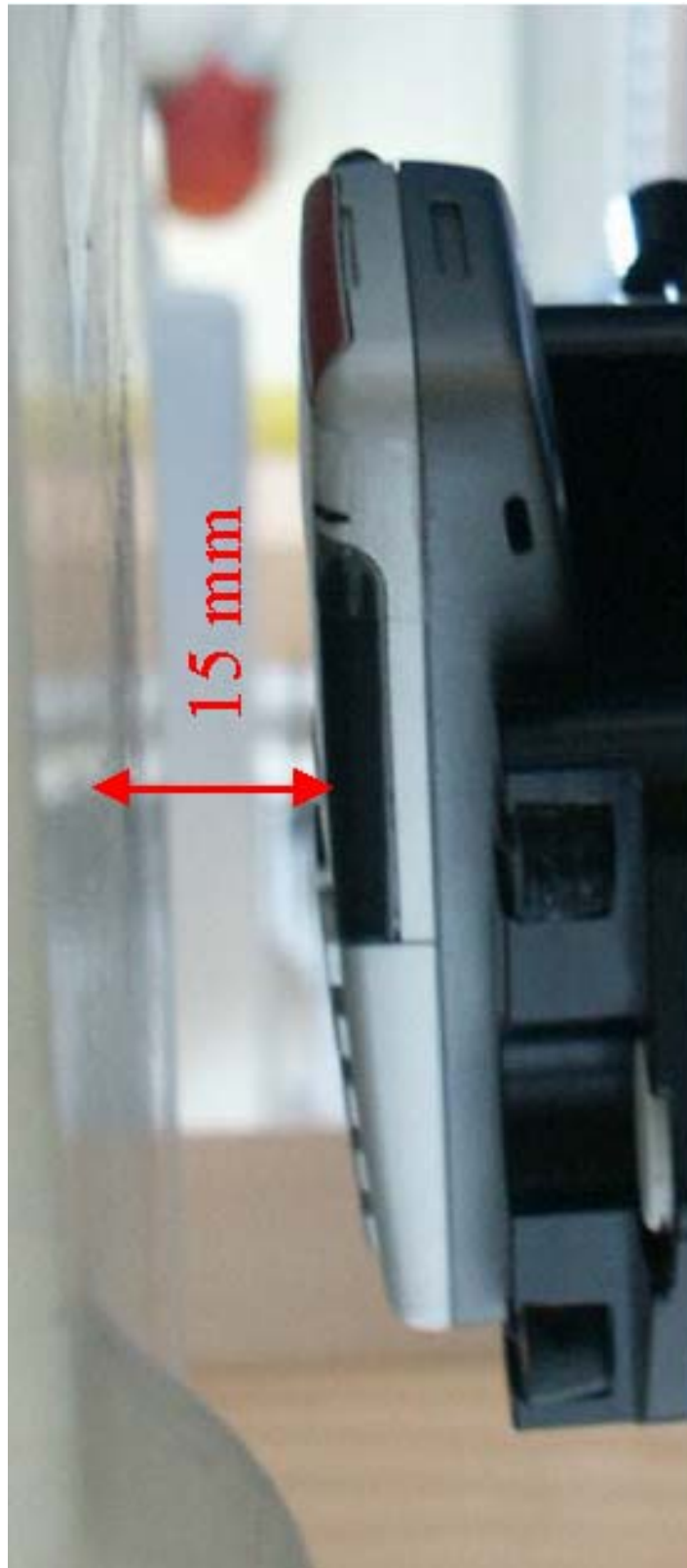
Fig. 30: Body worn configuration, with 1.5 cm distance between mobile and phantom, display towards the phantom
