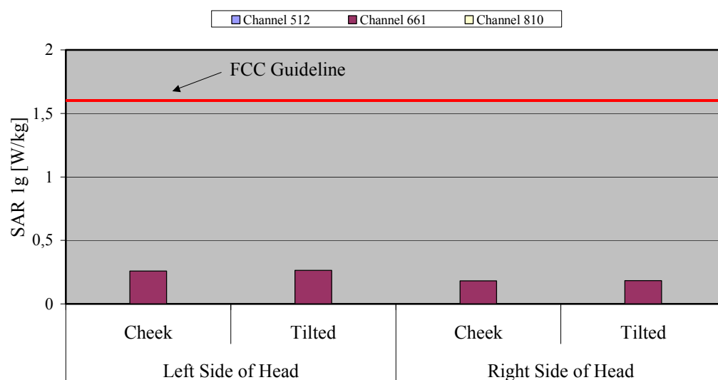
Fig. 9: The measured head phantom SAR values for the Alcatel One Touch 331a for PCS 1900 in comparison to the FCC exposure limit.
