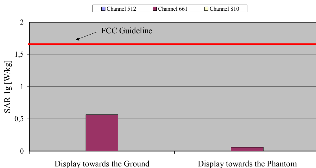
Fig. 13: The measured SAR values in body-worn configuration for the Alcatel One Touch 331a for PCS 1900, with 1.5 cm distance between mobile and phantom, in comparison to the FCC exposure limit.
