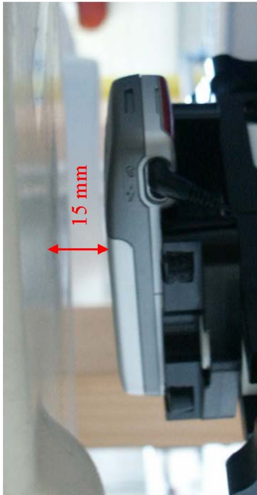
Fig. 29: Body worn configuration, with 1.5 cm distance between mobile and phantom, display towards the ground
