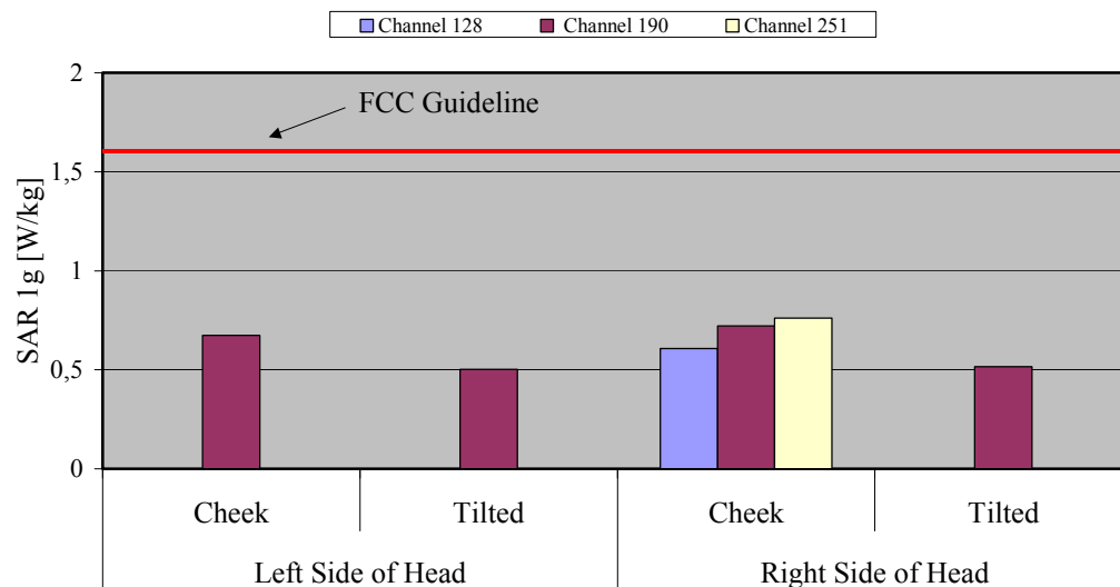
Fig. 8: The measured head phantom SAR values for the Alcatel One Touch 331a for GSM 850 in comparison to the FCC exposure limit.
