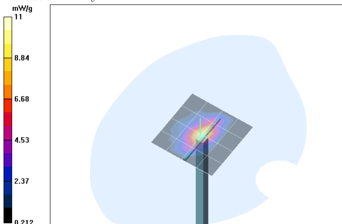
Fig. 16: Validation measurement 1900 MHz Head (October 09, 2003), coarse grid. Ambient Temperature: 20.8° C, Liquid Temperature: 20.4° C.
