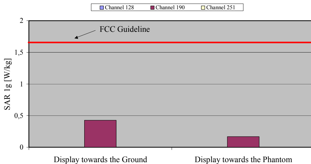
Fig. 10: The measured SAR values in body-worn configuration for the Alcatel One Touch 331a, with belt clip and headset, in comparison to the FCC exposure limit.
