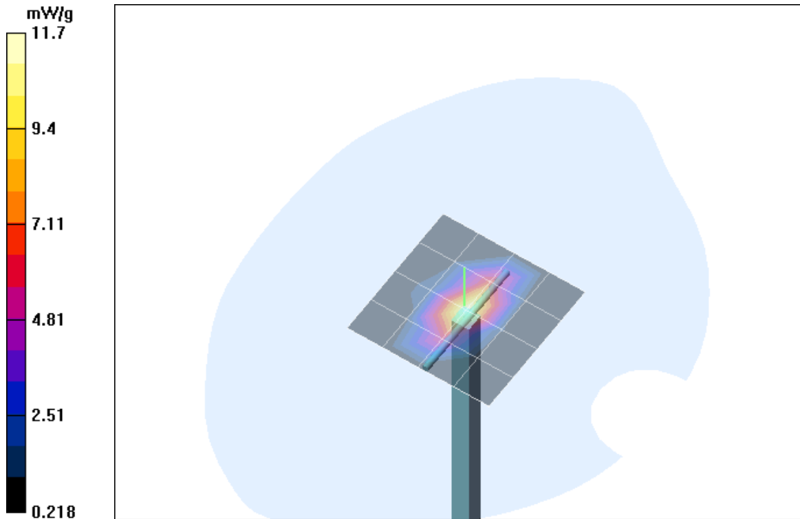
Fig. 17: Validation measurement 1900 MHz body (October 08, 2003), coarse grid. Ambient Temperature: 20.8° C, Liquid Temperature: 20.7° C.
