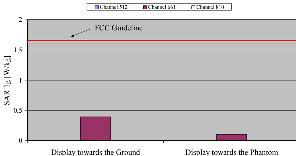
Fig. 12: The measured SAR values in body-worn configuration for the Alcatel One Touch 331a for PCS 1900, with belt clip and headset, in comparison to the FCC exposure limit.
