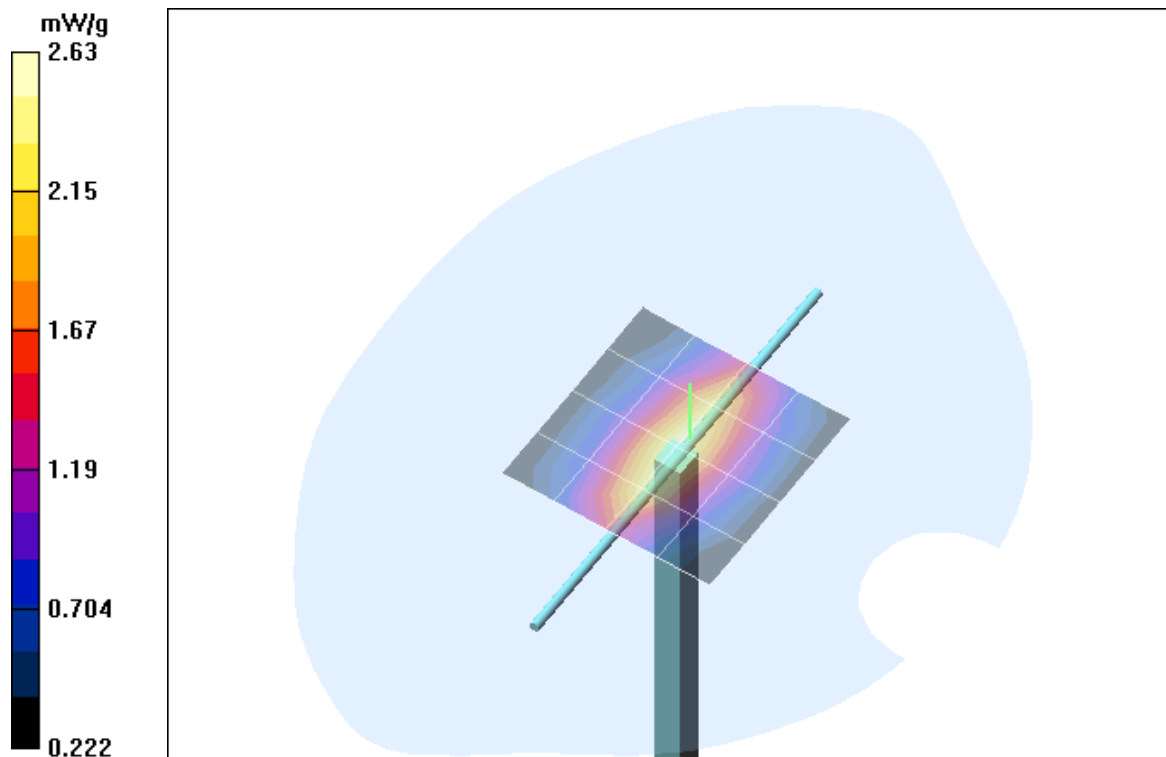
Fig. 14: Validation measurement 850 MHz Head (October 06, 2003), coarse grid. Ambient Temperature: 20.6° C, Liquid Temperature: 19.9° C.
