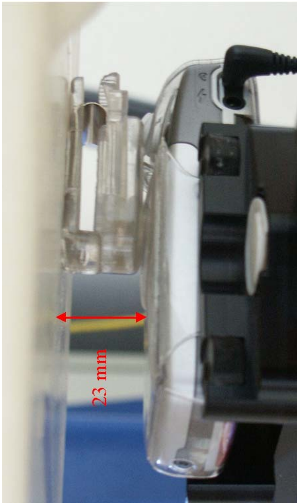
Fig. 27: Body worn configuration, belt clip with headset, display towards the ground.
