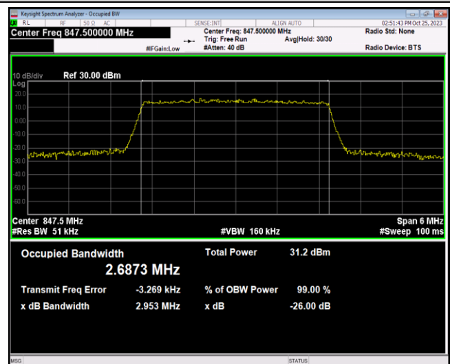
Band5-3MHz-16QAM-20525-15RB#0
