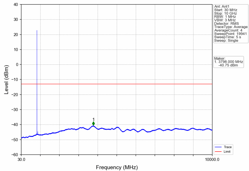
Band5_1.4MHz_16QAM_HCH_848.3MHz_RB_1_0_NTNV
