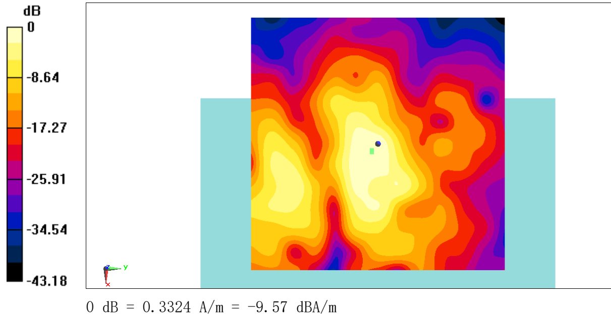
Fig B.5 T-Coil WiFi-5G
