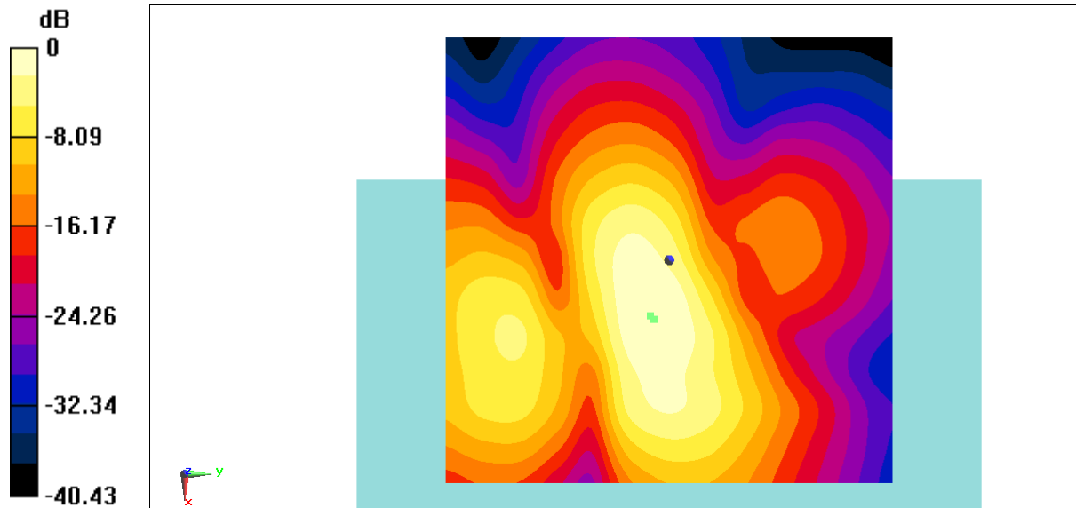
Fig B.3 T-Coil LTE B41
