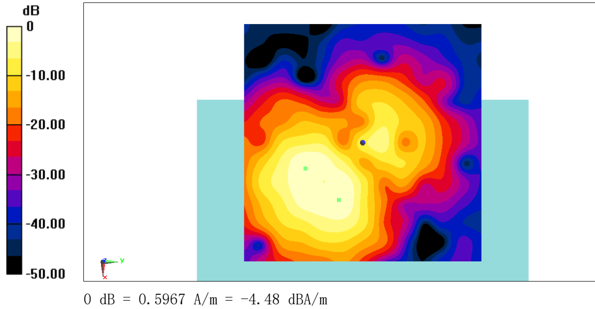
Fig B.6 T-Coil WiFi-5G
