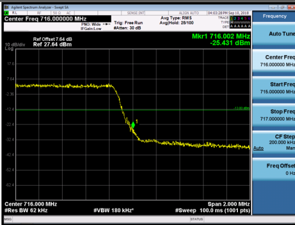
HCH_QPSK_15RB#0
