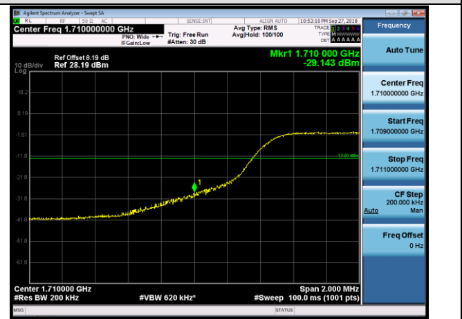
LCH_16QAM_50RB#0
