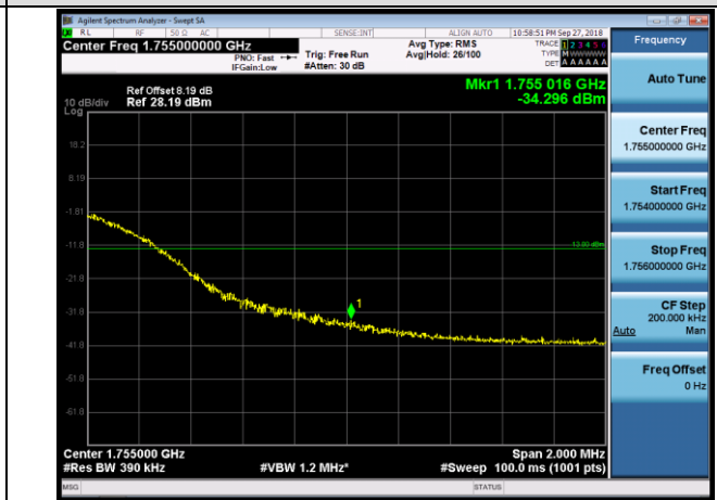
HCH_16QAM_100RB#0
