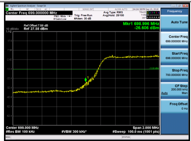
LCH_16QAM_25RB#0
