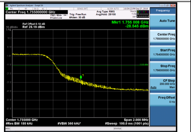
HCH_16QAM_50RB#0
