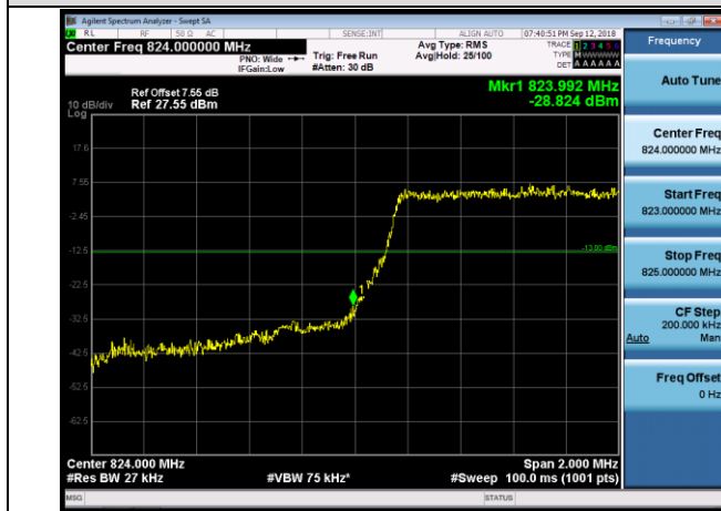
LCH_QPSK_6RB#0
