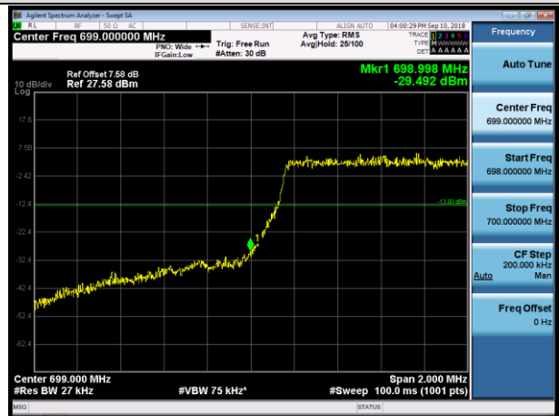
LCH_16QAM_6RB#0
