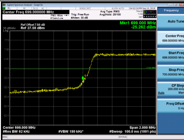
LCH_QPSK_15RB#0
