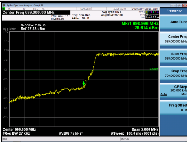
LCH_QPSK_6RB#0
