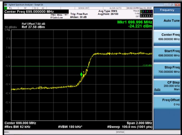
LCH_16QAM_15RB#0
