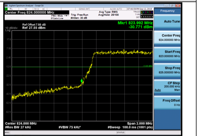
LCH_16QAM_6RB#0
