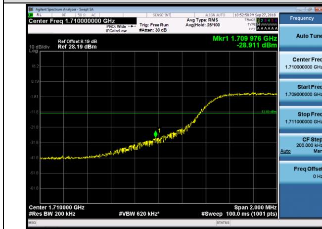
LCH_QPSK_50RB#0
