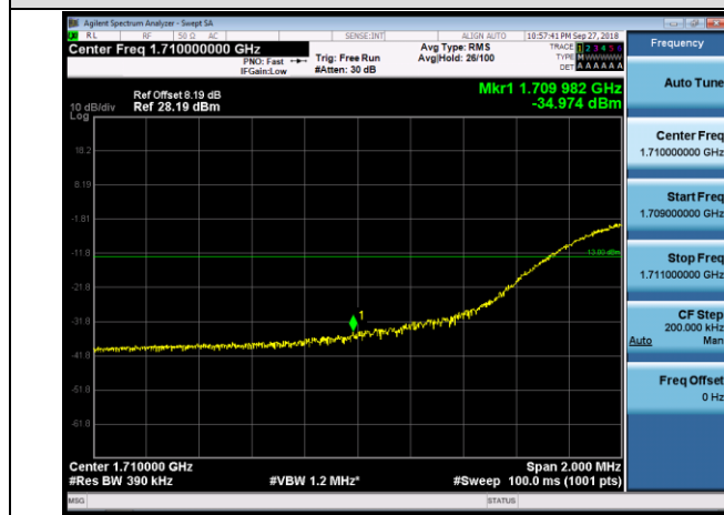
LCH_QPSK_100RB#0
