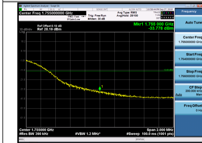
HCH_QPSK_100RB#0
