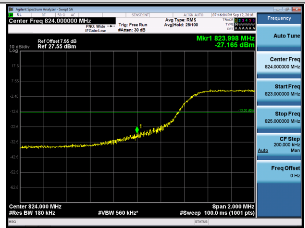
LCH_16QAM_50RB#0
