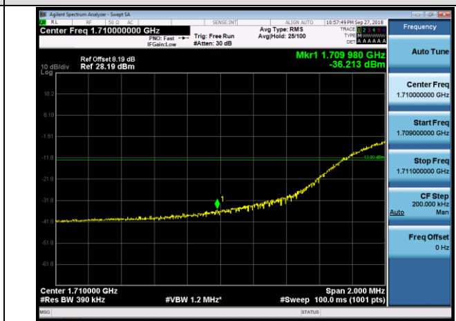
LCH_16QAM_100RB#0
