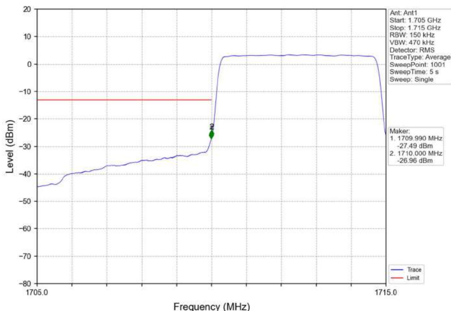
Band4_5MHz_16QAM_LCH_1712.5MHz_RB_25_0_NTNV
