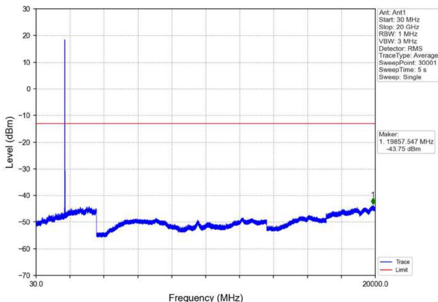
Band4_10MHz_16QAM_MCH_1732.5MHz_RB_1_0_NTNV
