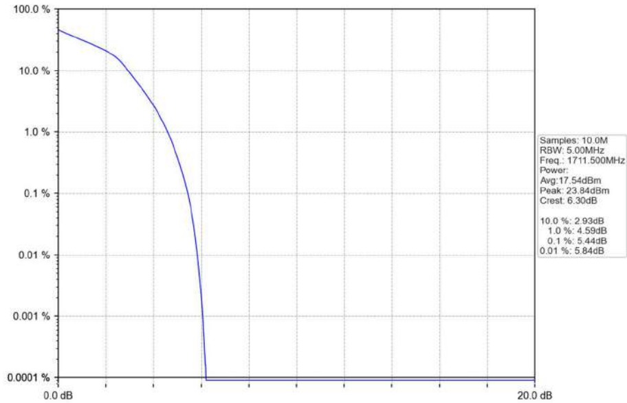
Band4_3MHz_16QAM_LCH_1711.5MHz_RB_15_0_NTNV
