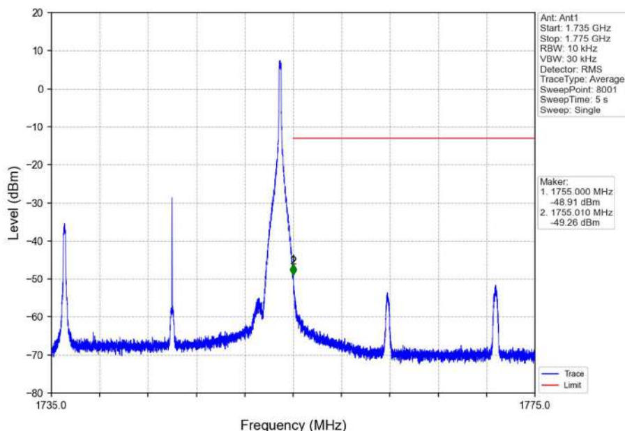
Band4_20MHz_16QAM_HCH_1745MHz_RB_1_99_NTNV
