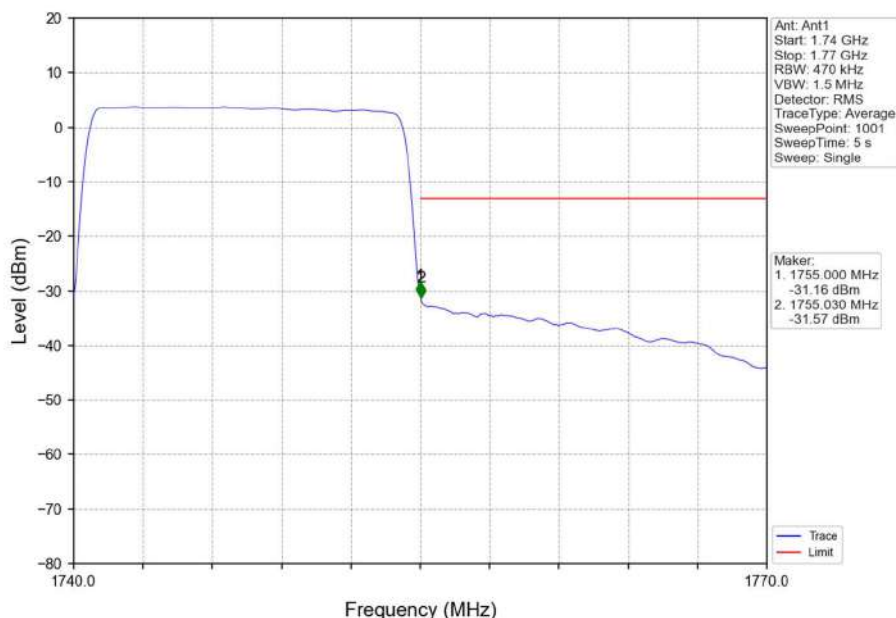
Band4_15MHz_16QAM_HCH_1747.5MHz_RB_75_0_NTNV
