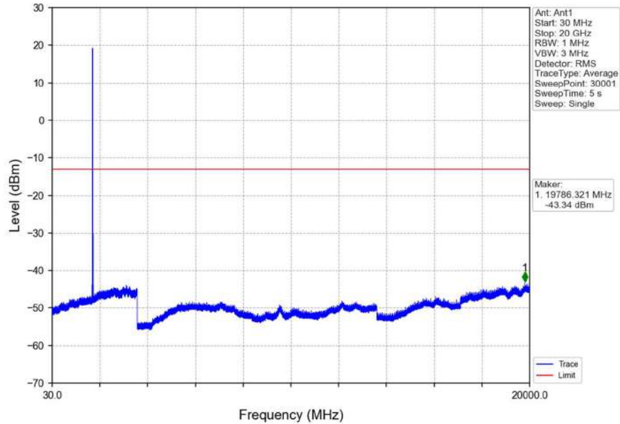
Band4_10MHz_QPSK_MCH_1732.5MHz_RB_1_0_NTNV
