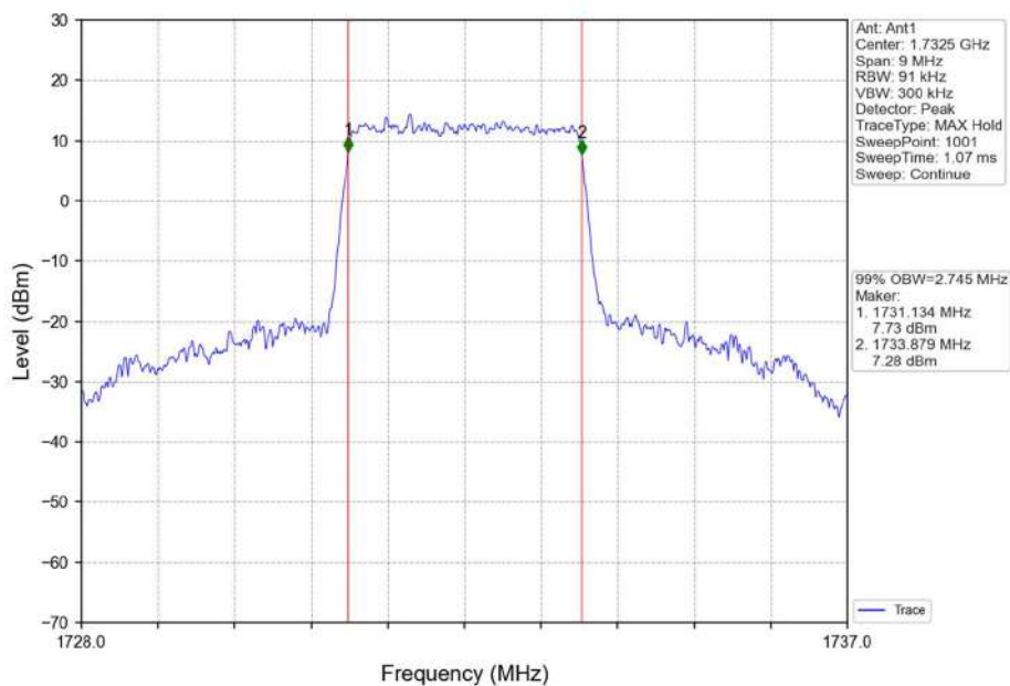
Band4_3MHz_16QAM_MCH_1732.5MHz_RB_15_0_NTNV
