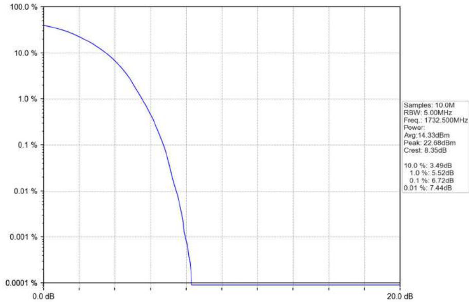
Band4_15MHz_QPSK_MCH_1732.5MHz_RB_75_0_NTNV
