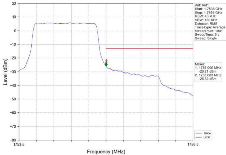
Band4_1.4MHz_QPSK_HCH_1754.3MHz_RB_6_0_NTNV
