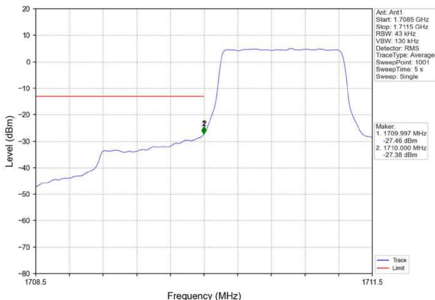
Band4_1.4MHz_QPSK_LCH_1710.7MHz_RB_6_0_NTNV
