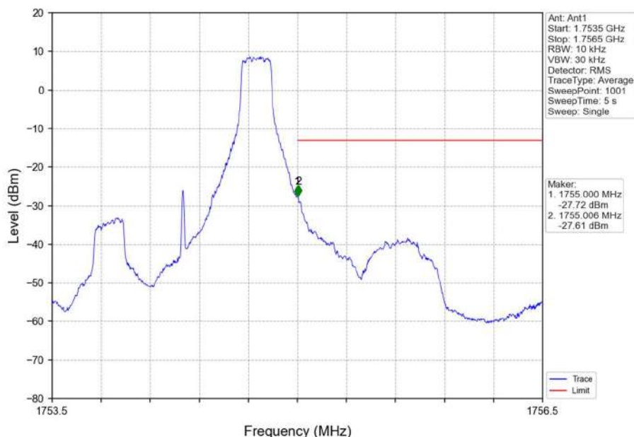
Band4_1.4MHz_QPSK_HCH_1754.3MHz_RB_1_5_NTNV
