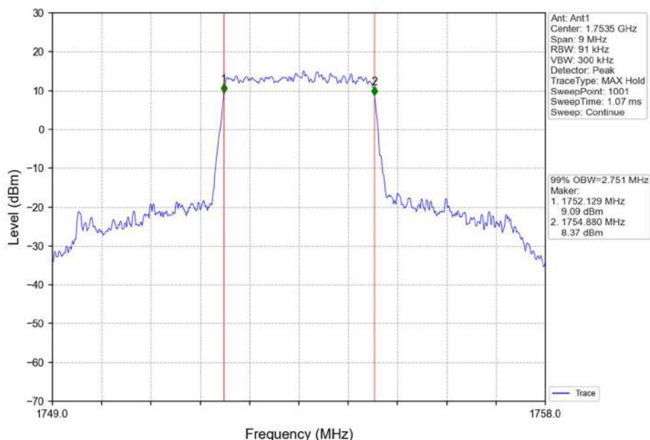
Band4_3MHz_QPSK_HCH_1753.5MHz_RB_15_0_NTNV
