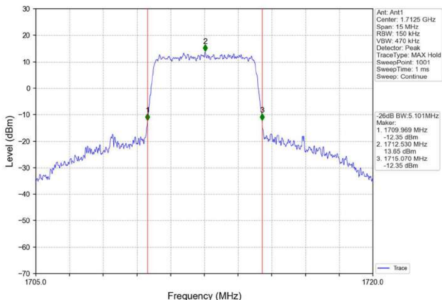
Band4_5MHz_16QAM_LCH_1712.5MHz_RB_25_0_NTNV
