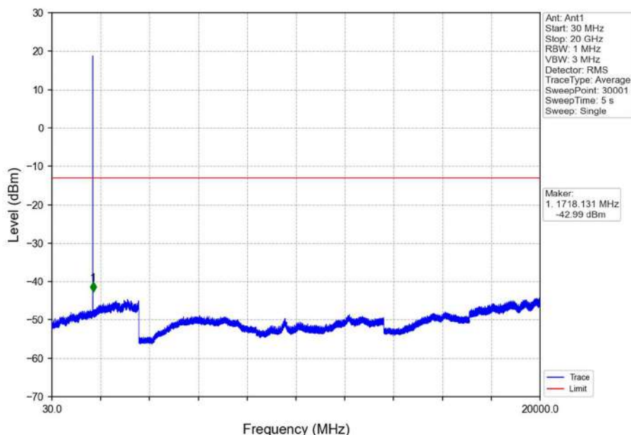
Band4_1.4MHz_QPSK_LCH_1710.7MHz_RB_1_0_NTNV
