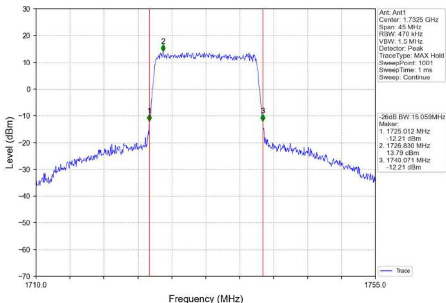
Band4_15MHz_16QAM_MCH_1732.5MHz_RB_75_0_NTNV
