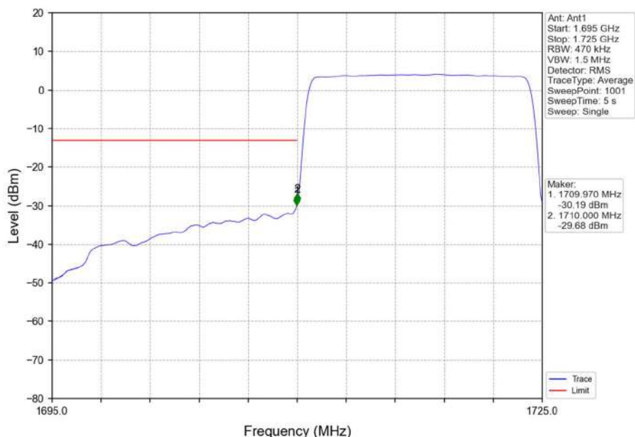
Band4_15MHz_QPSK_LCH_1717.5MHz_RB_75_0_NTNV
