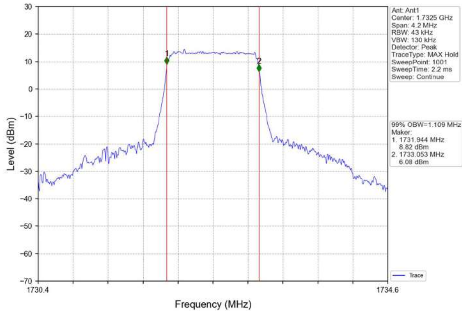
Band4_1.4MHz_16QAM_MCH_1732.5MHz_RB_6_0_NTNV
