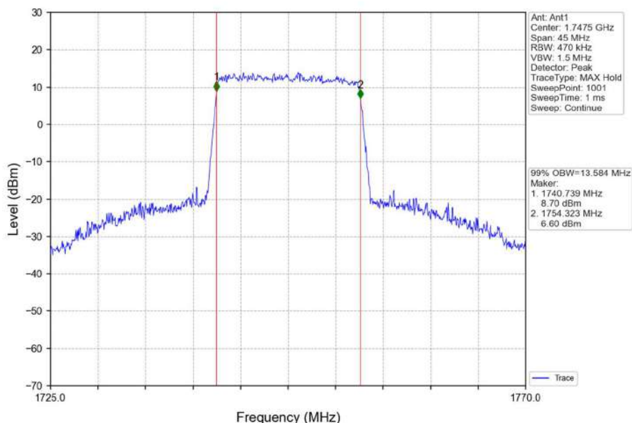
Band4_15MHz_16QAM_HCH_1747.5MHz_RB_75_0_NTNV
