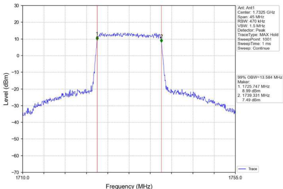
Band4_15MHz_16QAM_MCH_1732.5MHz_RB_75_0_NTNV
