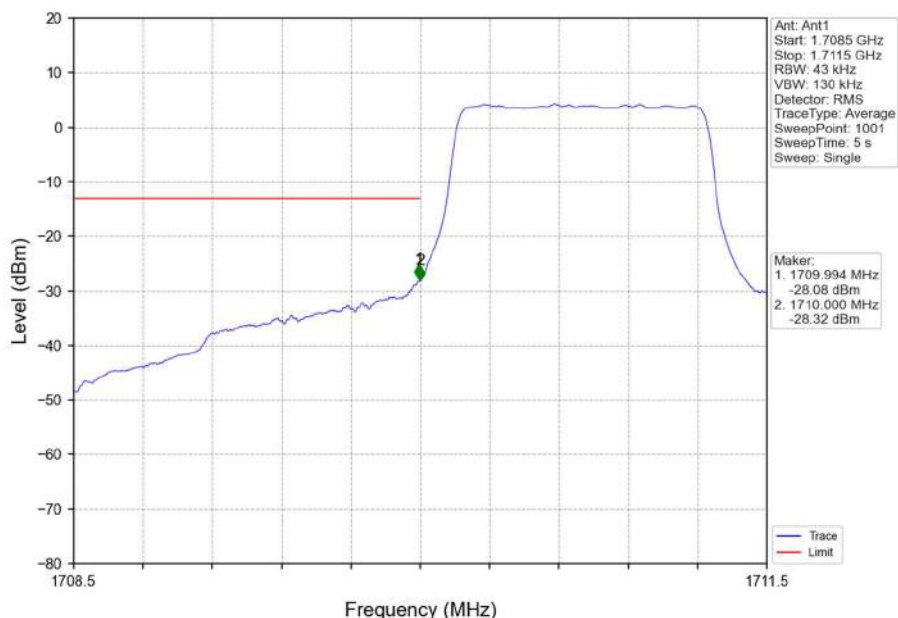
Band4_1.4MHz_16QAM_LCH_1710.7MHz_RB_6_0_NTNV
