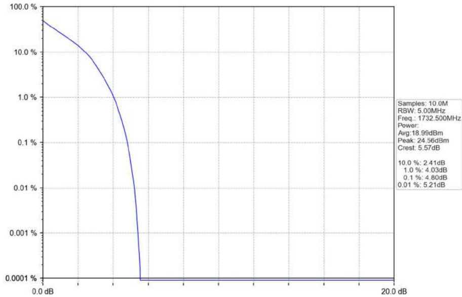
Band4_3MHz_QPSK_MCH_1732.5MHz_RB_15_0_NTNV
