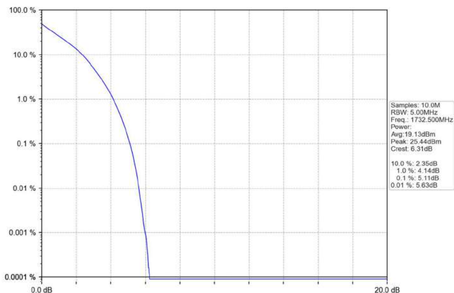
Band4_5MHz_QPSK_MCH_1732.5MHz_RB_25_0_NTNV
