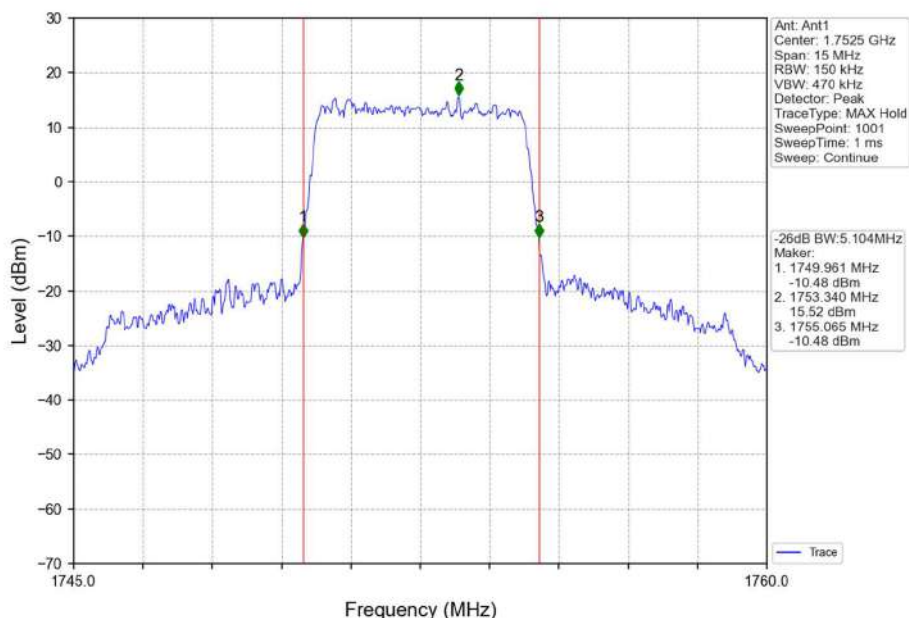
Band4_5MHz_QPSK_HCH_1752.5MHz_RB_25_0_NTNV
