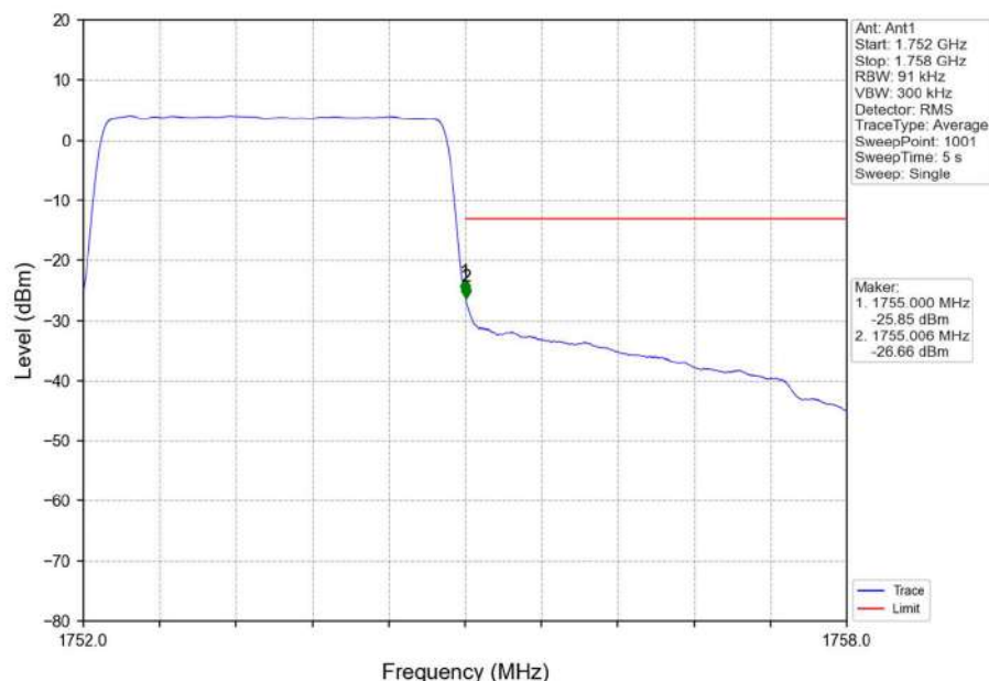
Band4_3MHz_16QAM_HCH_1753.5MHz_RB_15_0_NTNV
