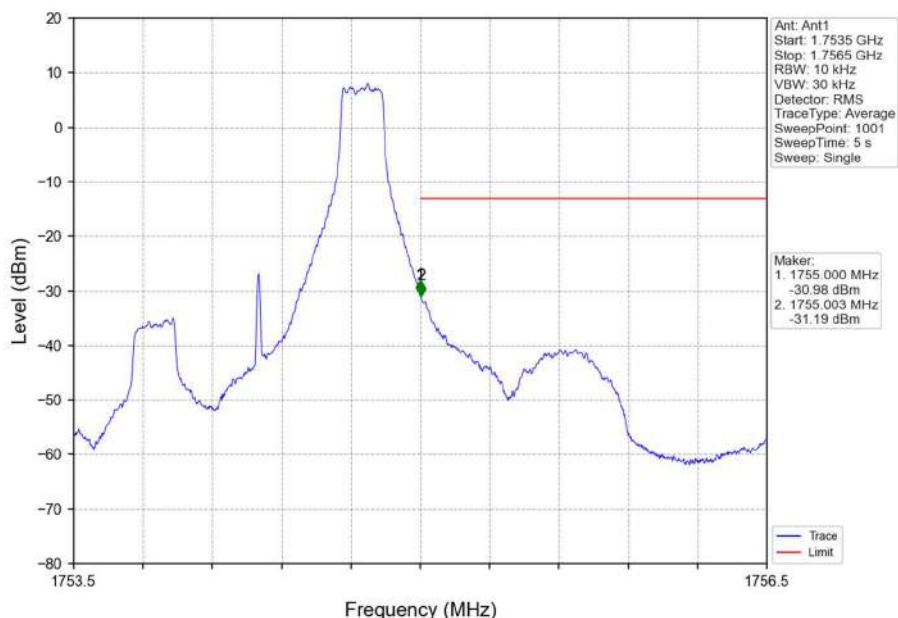
Band4_1.4MHz_16QAM_HCH_1754.3MHz_RB_1_5_NTNV
