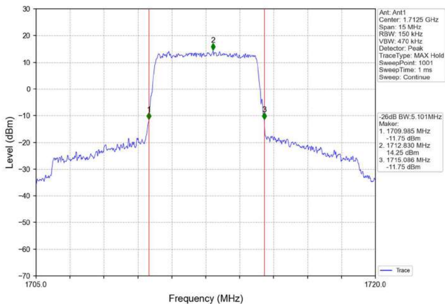
Band4_5MHz_QPSK_LCH_1712.5MHz_RB_25_0_NTNV
