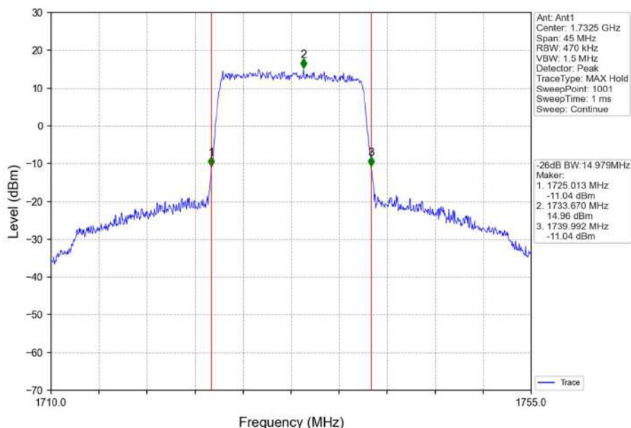
Band4_15MHz_QPSK_MCH_1732.5MHz_RB_75_0_NTNV
