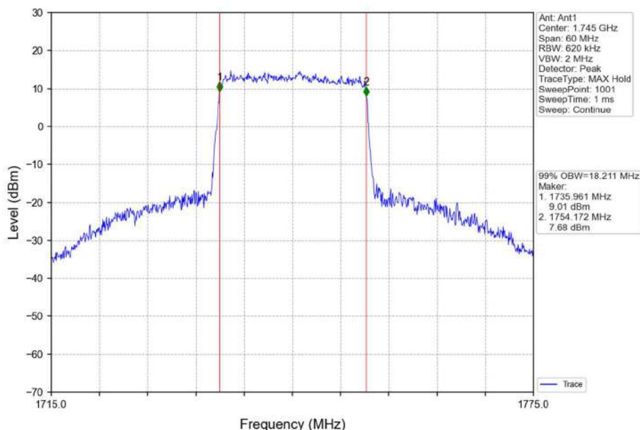
Band4_20MHz_16QAM_HCH_1745MHz_RB_100_0_NTNV
