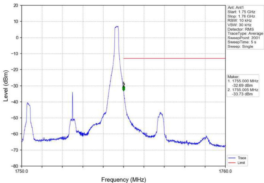
Band4_5MHz_16QAM_HCH_1752.5MHz_RB_1_24_NTNV
