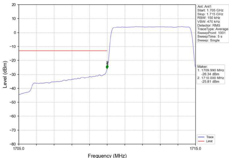
Band4_5MHz_QPSK_LCH_1712.5MHz_RB_25_0_NTNV
