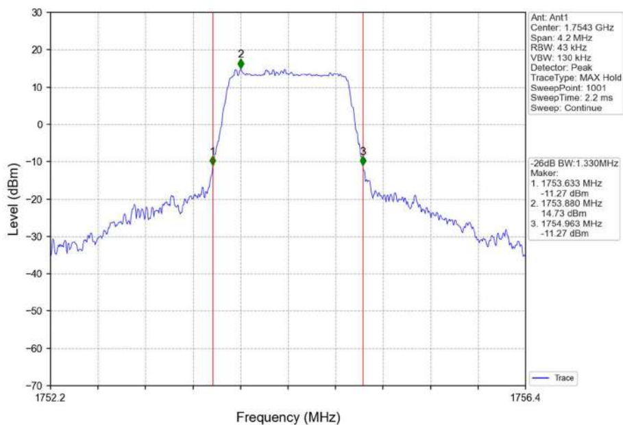
Band4_1.4MHz_16QAM_HCH_1754.3MHz_RB_6_0_NTNV
