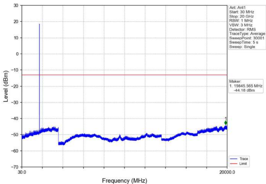
Band4_3MHz_16QAM_HCH_1753.5MHz_RB_1_0_NTNV
