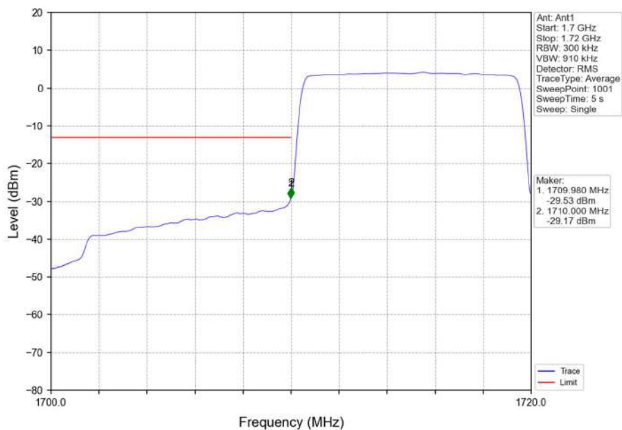
Band4_10MHz_QPSK_LCH_1715MHz_RB_50_0_NTNV
