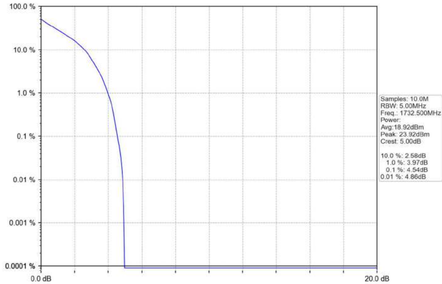
Band4_1.4MHz_QPSK_MCH_1732.5MHz_RB_6_0_NTNV
