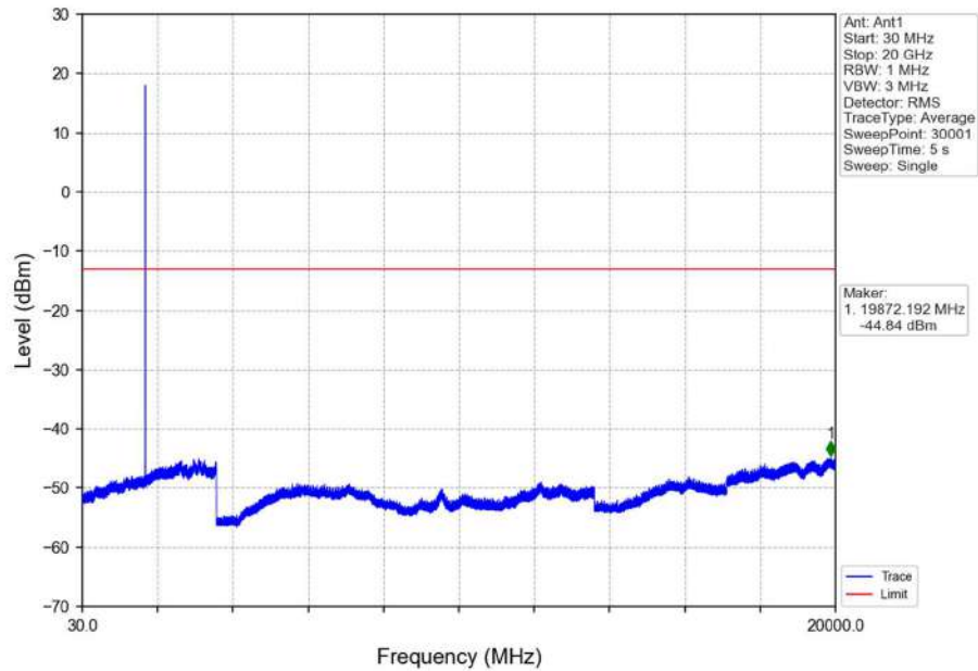
Band4_1.4MHz_16QAM_LCH_1710.7MHz_RB_1_0_NTNV
