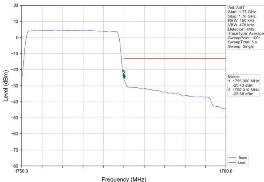
Band4_5MHz_QPSK_HCH_1752.5MHz_RB_25_0_NTNV
