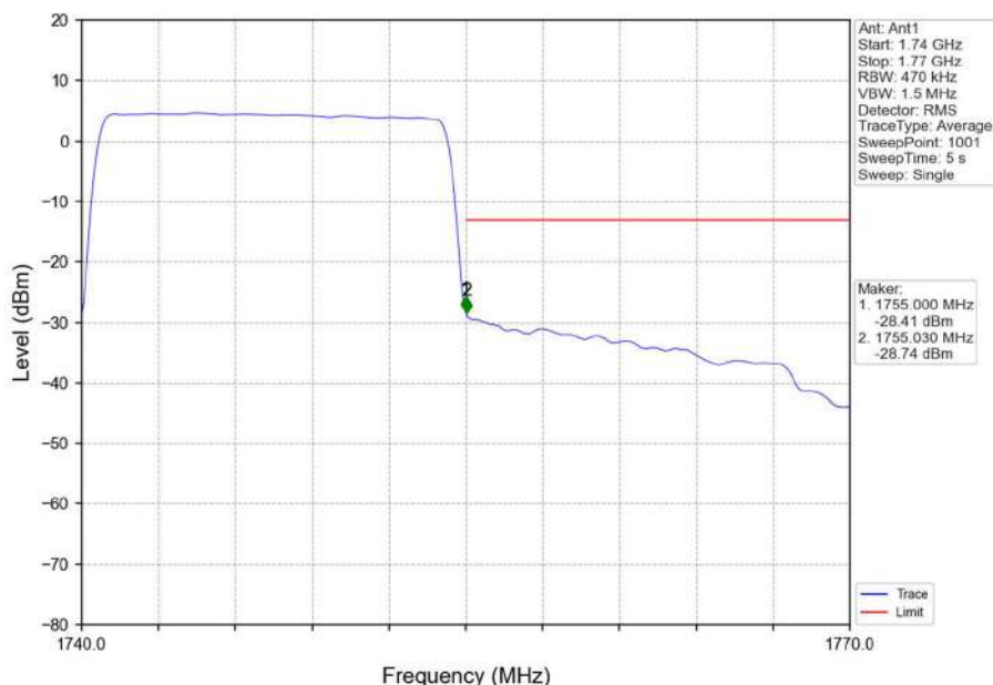
Band4_15MHz_QPSK_HCH_1747.5MHz_RB_75_0_NTNV
