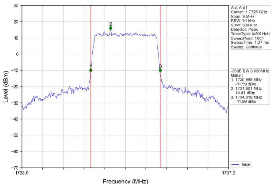
Band4_3MHz_16QAM_MCH_1732.5MHz_RB_15_0_NTNV
