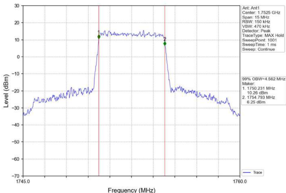
Band4_5MHz_QPSK_HCH_1752.5MHz_RB_25_0_NTNV
