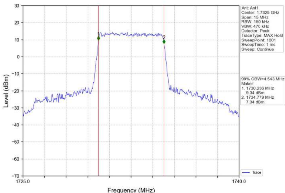
Band4_5MHz_QPSK_MCH_1732.5MHz_RB_25_0_NTNV
