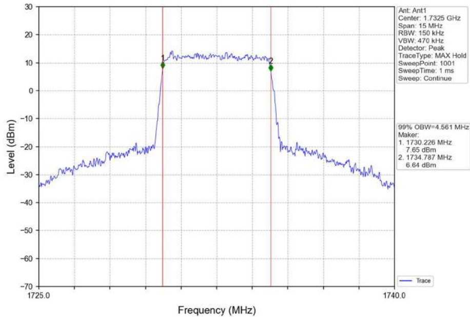
Band4_5MHz_16QAM_MCH_1732.5MHz_RB_25_0_NTNV
