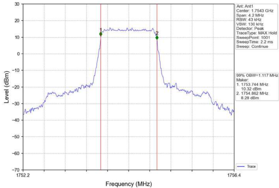
Band4_1.4MHz_QPSK_HCH_1754.3MHz_RB_6_0_NTNV
