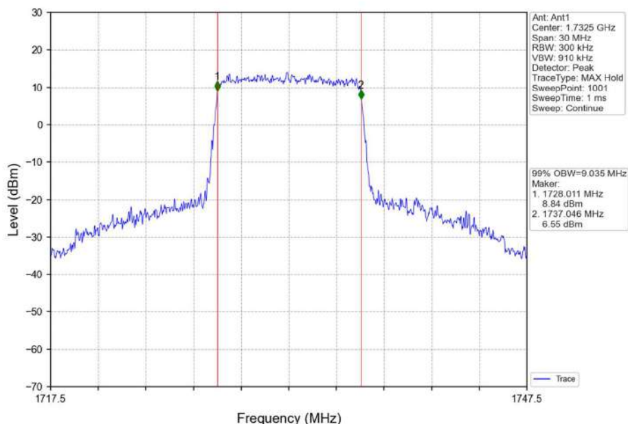
Band4_10MHz_16QAM_MCH_1732.5MHz_RB_50_0_NTNV
