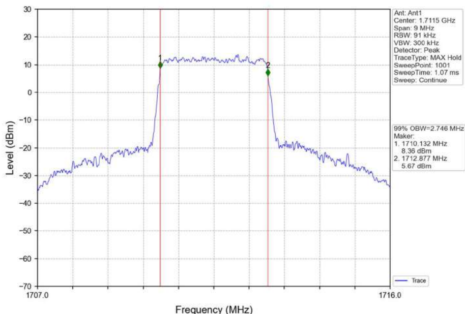
Band4_3MHz_16QAM_LCH_1711.5MHz_RB_15_0_NTNV
