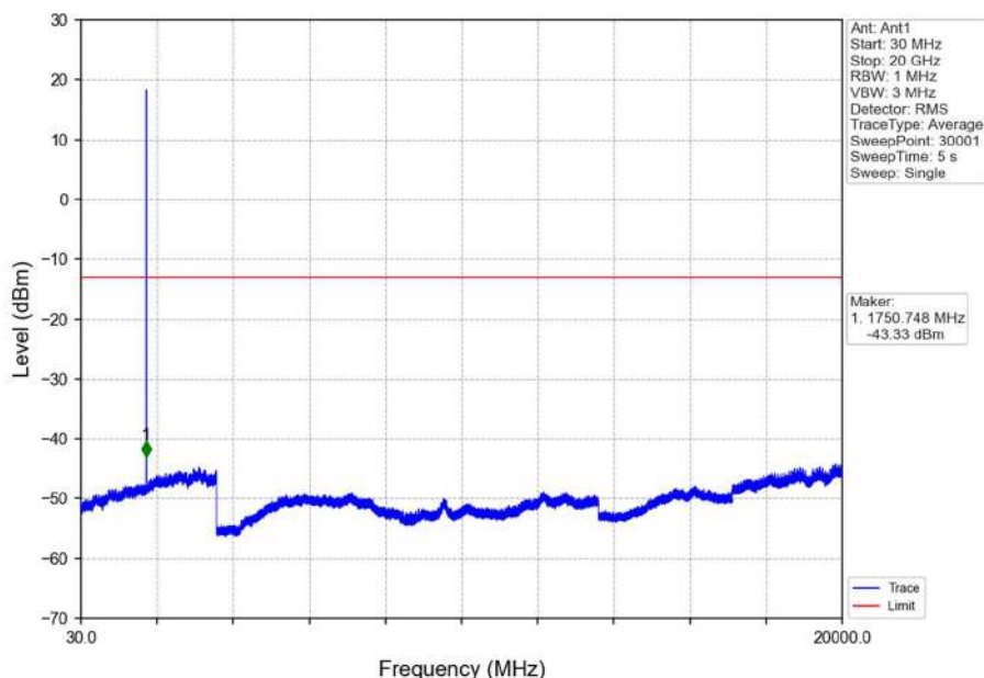
Band4_1.4MHz_16QAM_HCH_1754.3MHz_RB_1_0_NTNV
