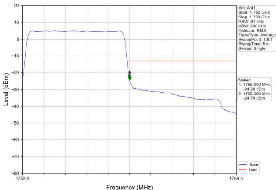
Band4_3MHz_QPSK_HCH_1753.5MHz_RB_15_0_NTNV
