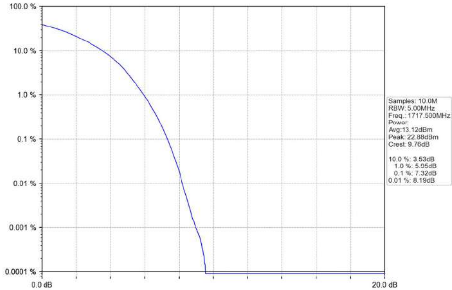
Band4_15MHz_16QAM_LCH_1717.5MHz_RB_75_0_NTNV
