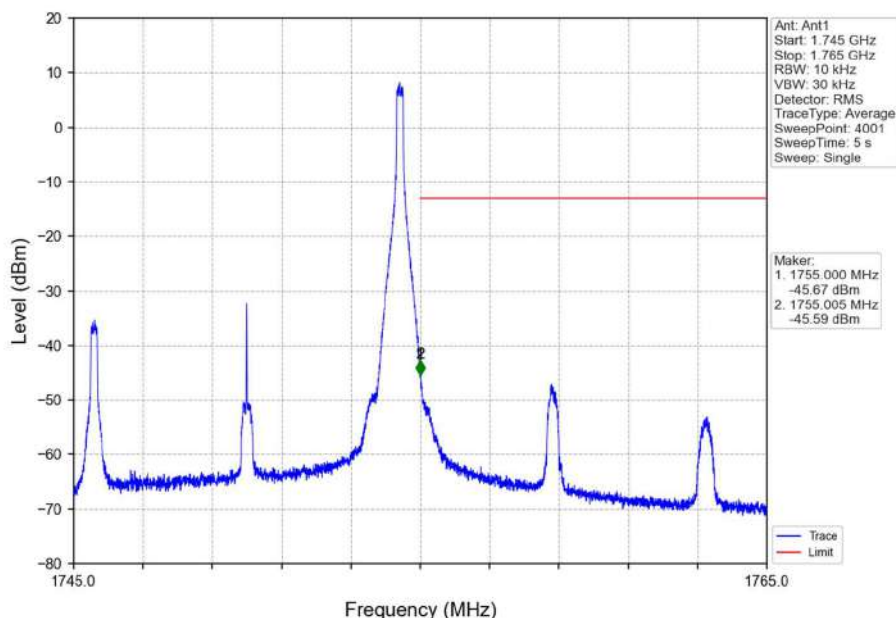
Band4_10MHz_16QAM_HCH_1750MHz_RB_1_49_NTNV
