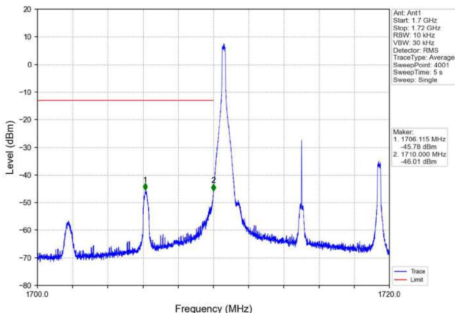
Band4_10MHz_16QAM_LCH_1715MHz_RB_1_0_NTNV
