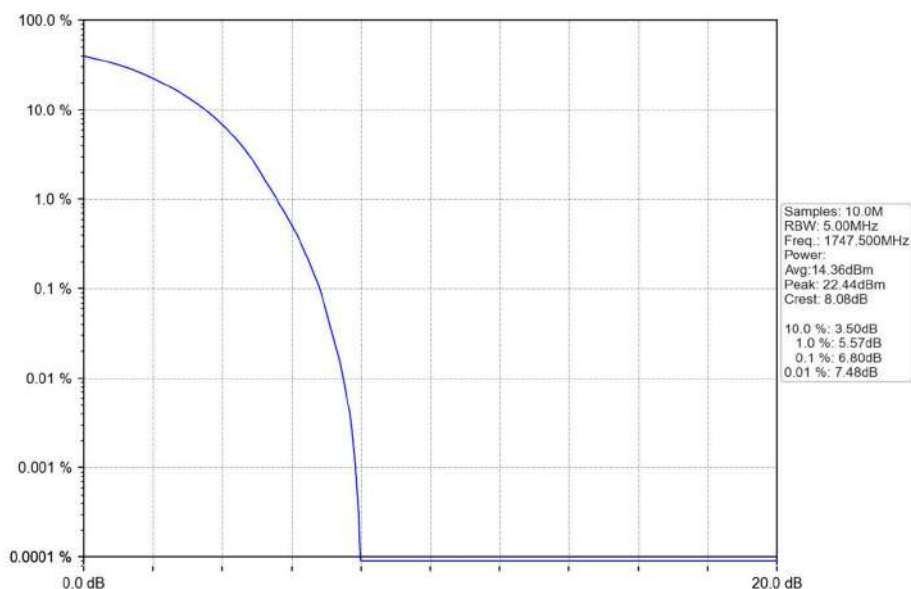
Band4_15MHz_QPSK_HCH_1747.5MHz_RB_75_0_NTNV
