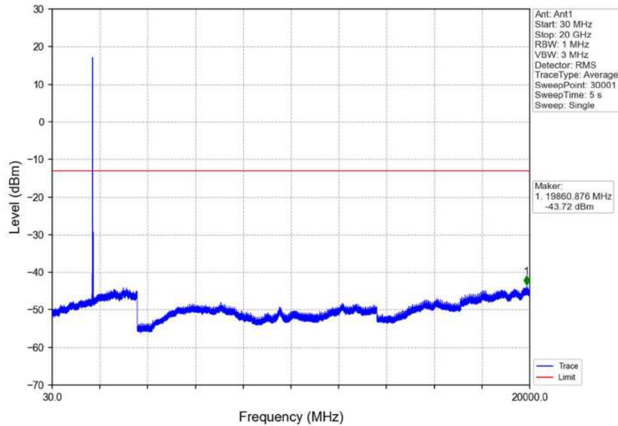
Band4_15MHz_16QAM_MCH_1732.5MHz_RB_1_0_NTNV
