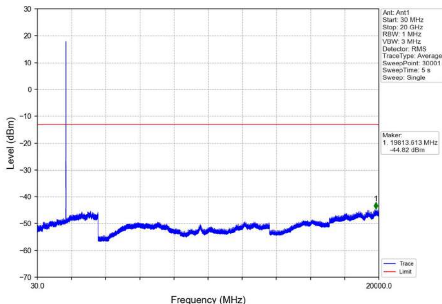
Band4_5MHz_16QAM_LCH_1712.5MHz_RB_1_0_NTNV
