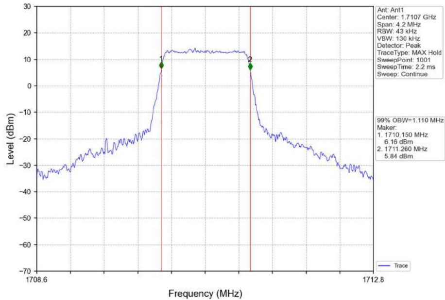
Band4_1.4MHz_16QAM_LCH_1710.7MHz_RB_6_0_NTNV
