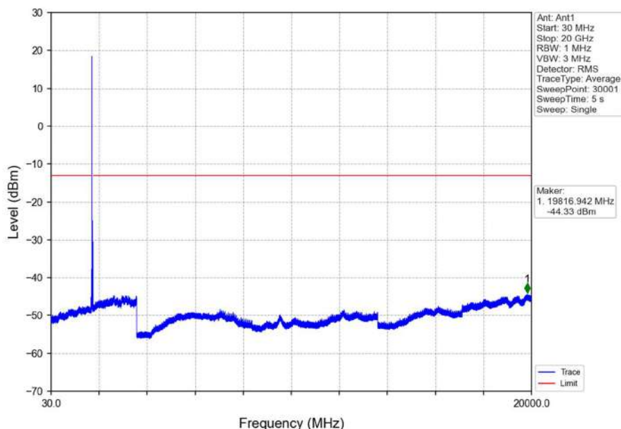
Band4_20MHz_16QAM_HCH_1745MHz_RB_1_0_NTNV
