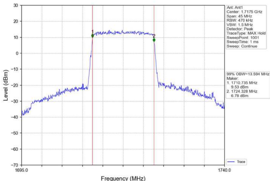
Band4_15MHz_QPSK_LCH_1717.5MHz_RB_75_0_NTNV
