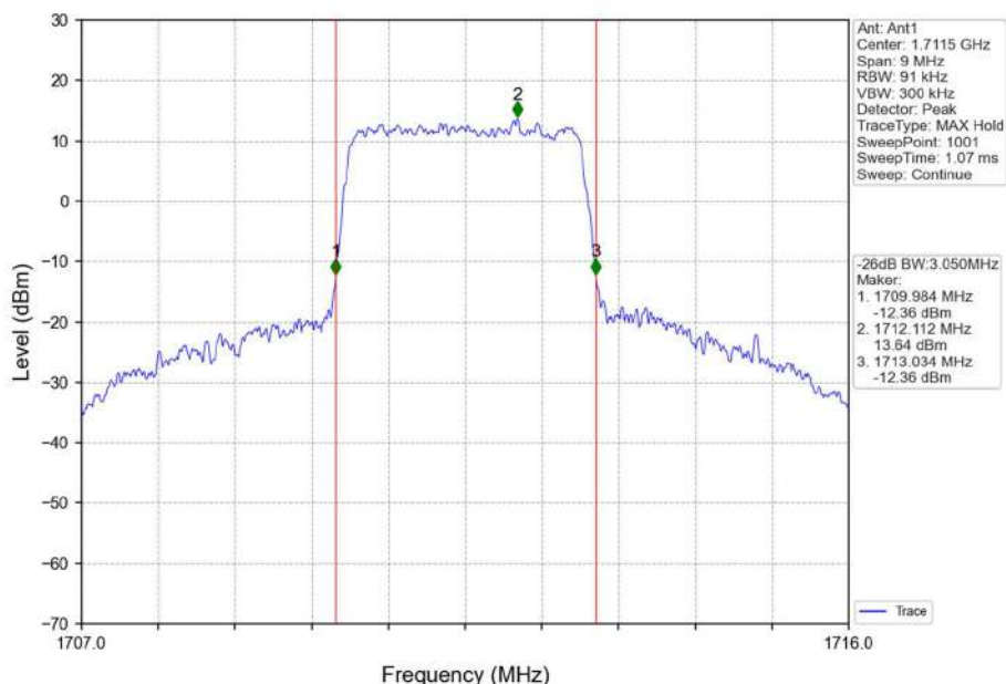
Band4_3MHz_16QAM_LCH_1711.5MHz_RB_15_0_NTNV
