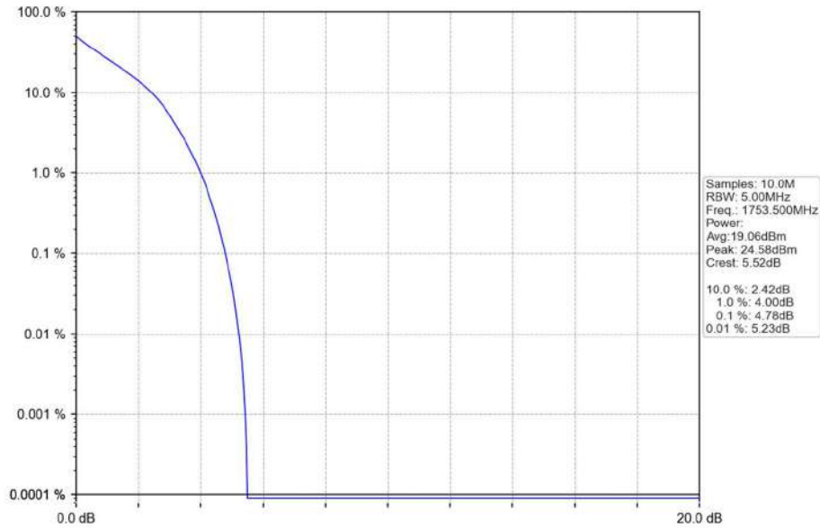
Band4_3MHz_QPSK_HCH_1753.5MHz_RB_15_0_NTNV
