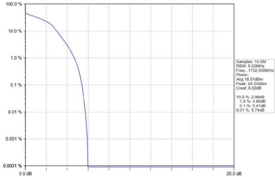
Band4_1.4MHz_16QAM_MCH_1732.5MHz_RB_6_0_NTNV
