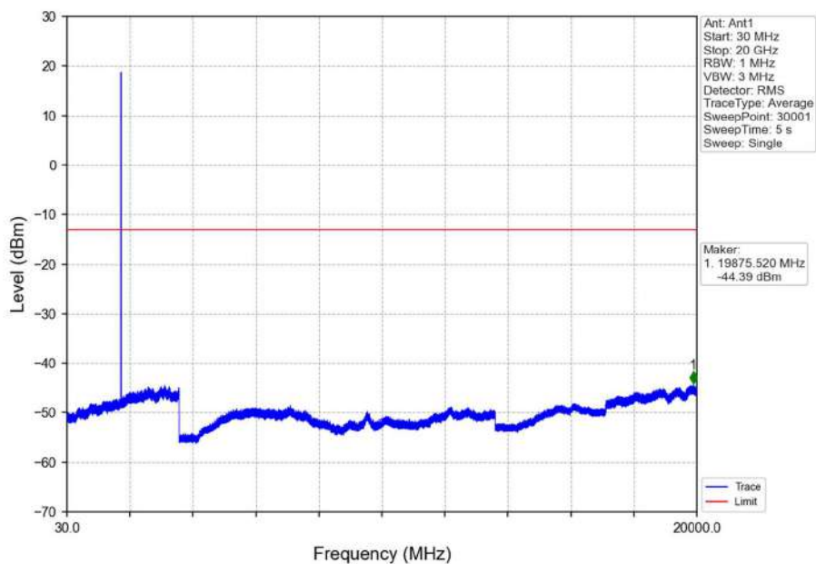
Band4_5MHz_QPSK_HCH_1752.5MHz_RB_1_0_NTNV
