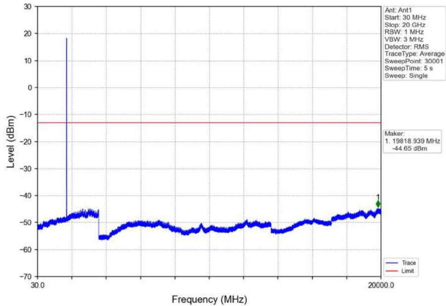
Band4_5MHz_16QAM_MCH_1732.5MHz_RB_1_0_NTNV
