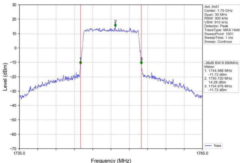
Band4_10MHz_16QAM_HCH_1750MHz_RB_50_0_NTNV
