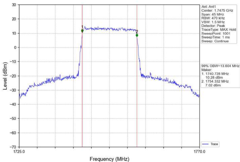
Band4_15MHz_QPSK_HCH_1747.5MHz_RB_75_0_NTNV
