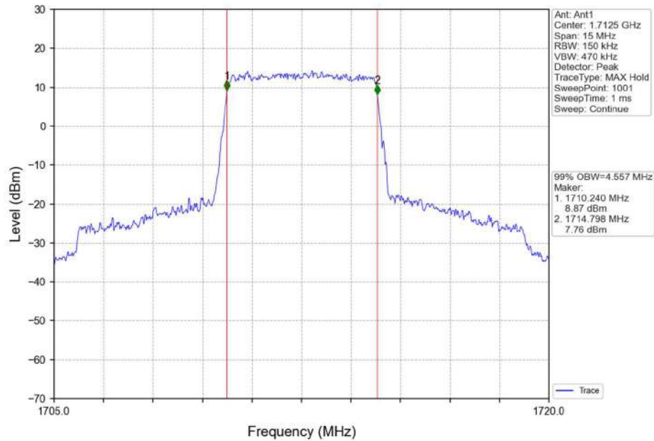
Band4_5MHz_QPSK_LCH_1712.5MHz_RB_25_0_NTNV
