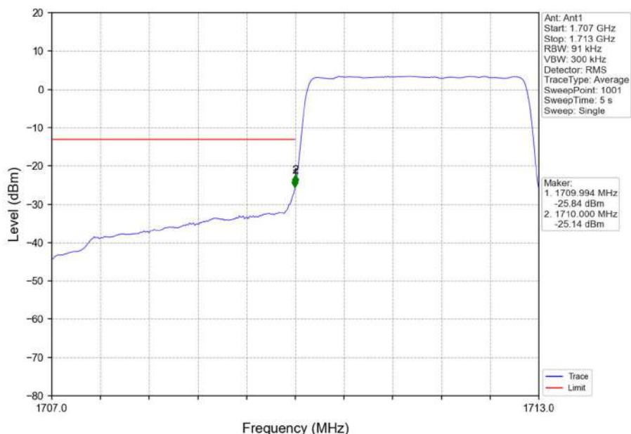
Band4_3MHz_16QAM_LCH_1711.5MHz_RB_15_0_NTNV
