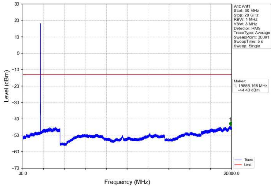
Band4_3MHz_16QAM_MCH_1732.5MHz_RB_1_0_NTNV
