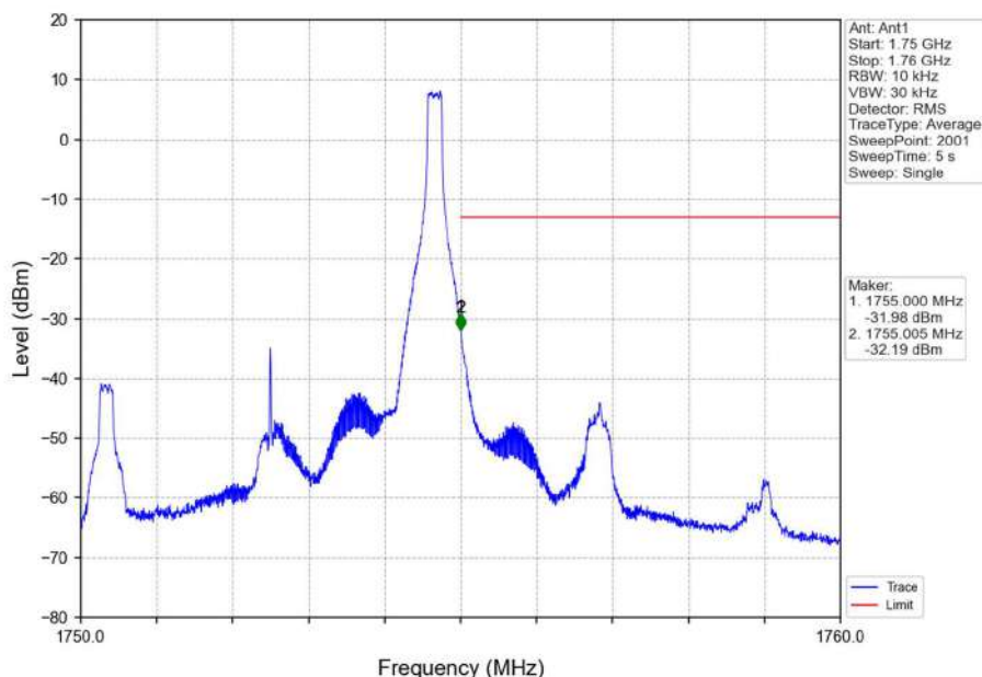
Band4_5MHz_QPSK_HCH_1752.5MHz_RB_1_24_NTNV
