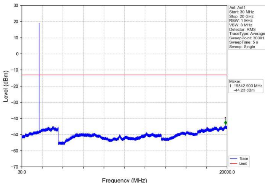
Band4_3MHz_QPSK_MCH_1732.5MHz_RB_1_0_NTNV
