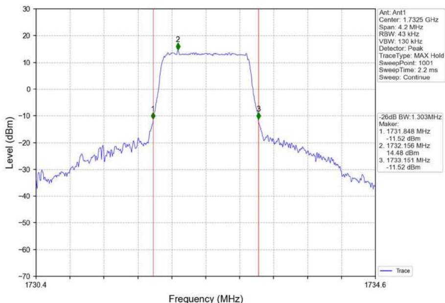
Band4_1.4MHz_16QAM_MCH_1732.5MHz_RB_6_0_NTNV
