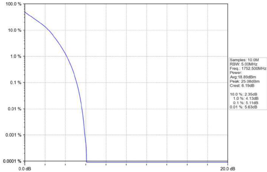
Band4_5MHz_QPSK_HCH_1752.5MHz_RB_25_0_NTNV
