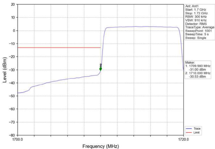
Band4_10MHz_16QAM_LCH_1715MHz_RB_50_0_NTNV
