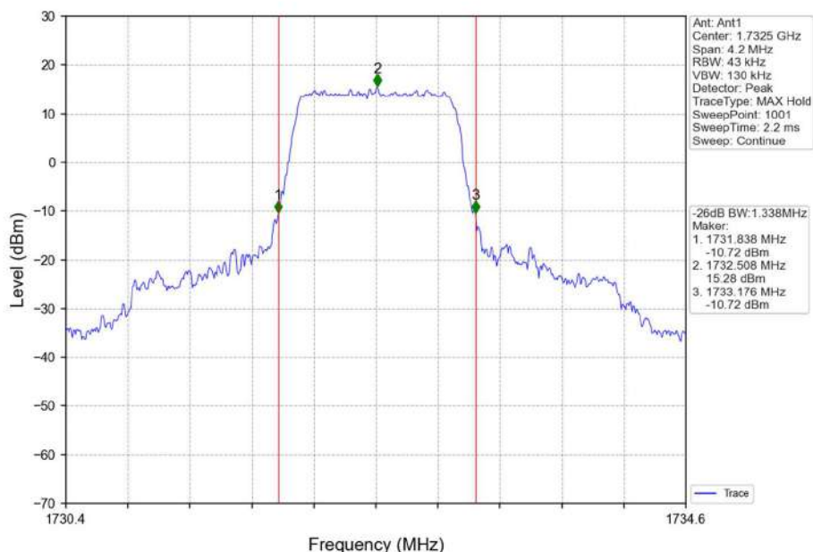
Band4_1.4MHz_QPSK_MCH_1732.5MHz_RB_6_0_NTNV
