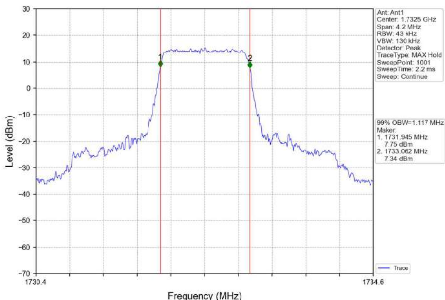
Band4_1.4MHz_QPSK_MCH_1732.5MHz_RB_6_0_NTNV
