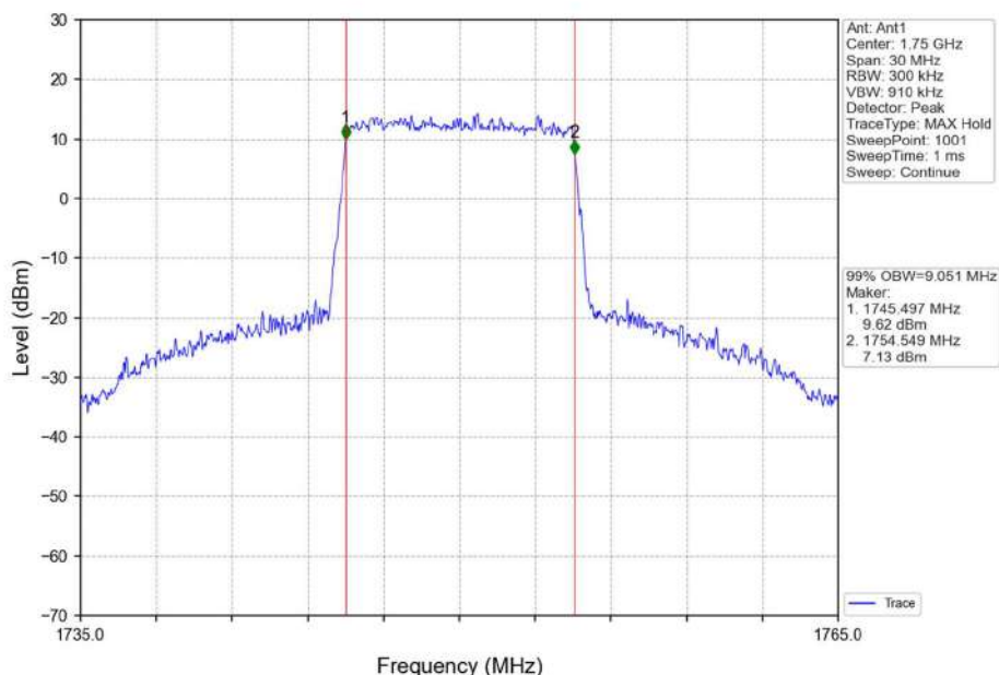
Band4_10MHz_16QAM_HCH_1750MHz_RB_50_0_NTNV
