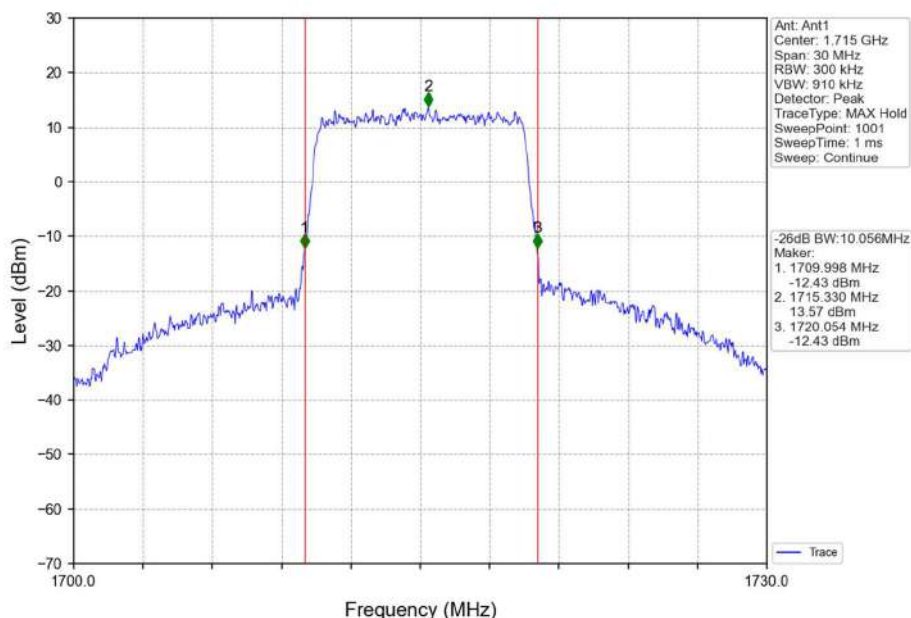
Band4_10MHz_16QAM_LCH_1715MHz_RB_50_0_NTNV
