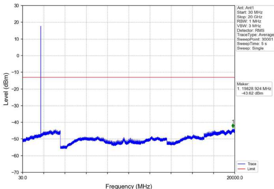
Band4_5MHz_16QAM_HCH_1752.5MHz_RB_1_0_NTNV
