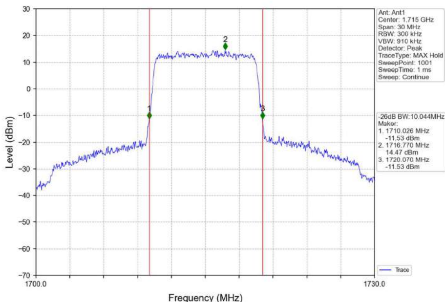
Band4_10MHz_QPSK_LCH_1715MHz_RB_50_0_NTNV
