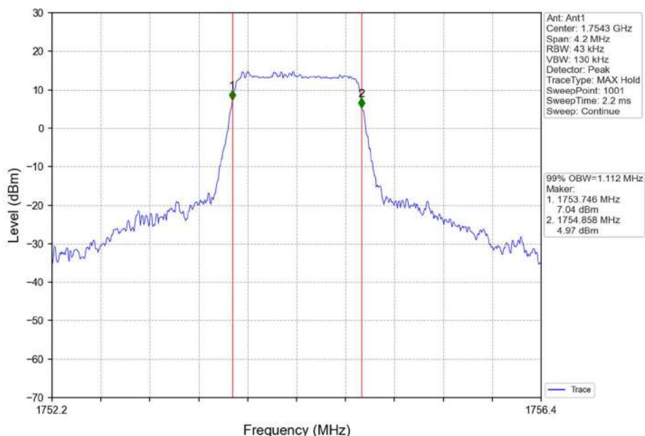
Band4_1.4MHz_16QAM_HCH_1754.3MHz_RB_6_0_NTNV
