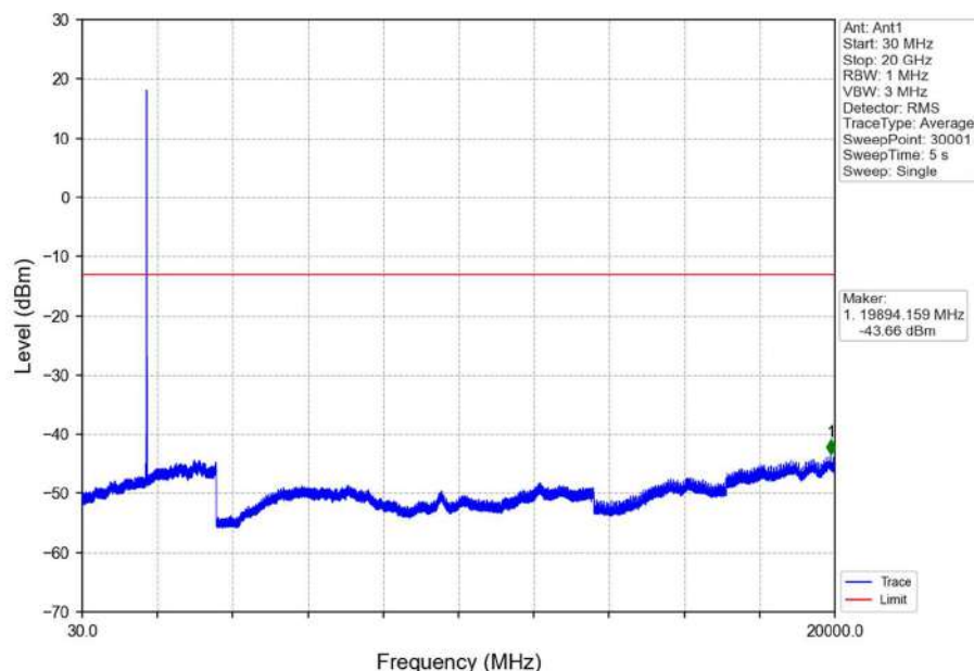
Band4_10MHz_16QAM_HCH_1750MHz_RB_1_0_NTNV
