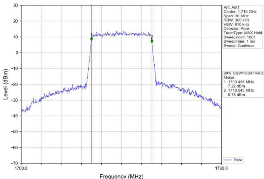
Band4_10MHz_16QAM_LCH_1715MHz_RB_50_0_NTNV
