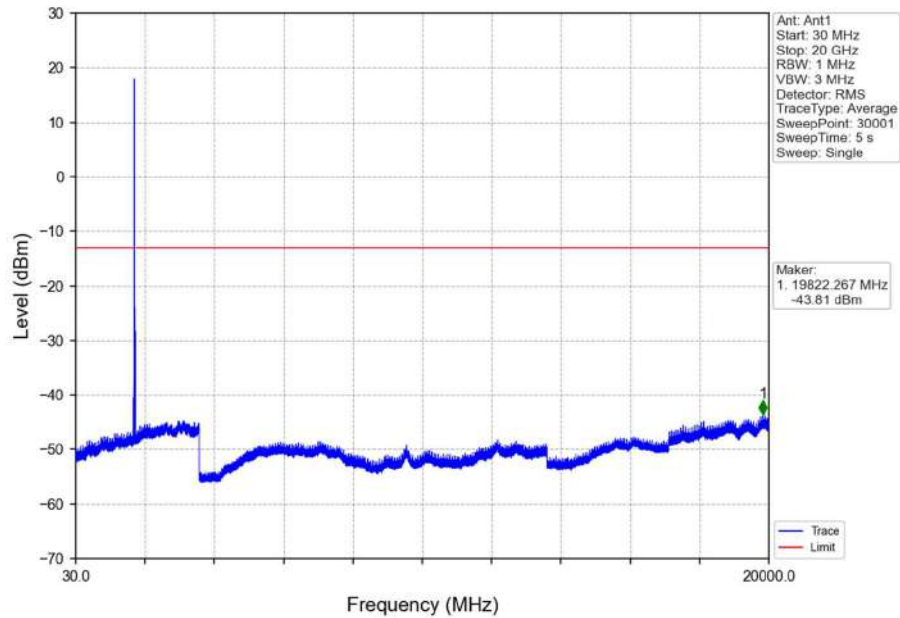
Band4_20MHz_16QAM_MCH_1732.5MHz_RB_1_0_NTNV
