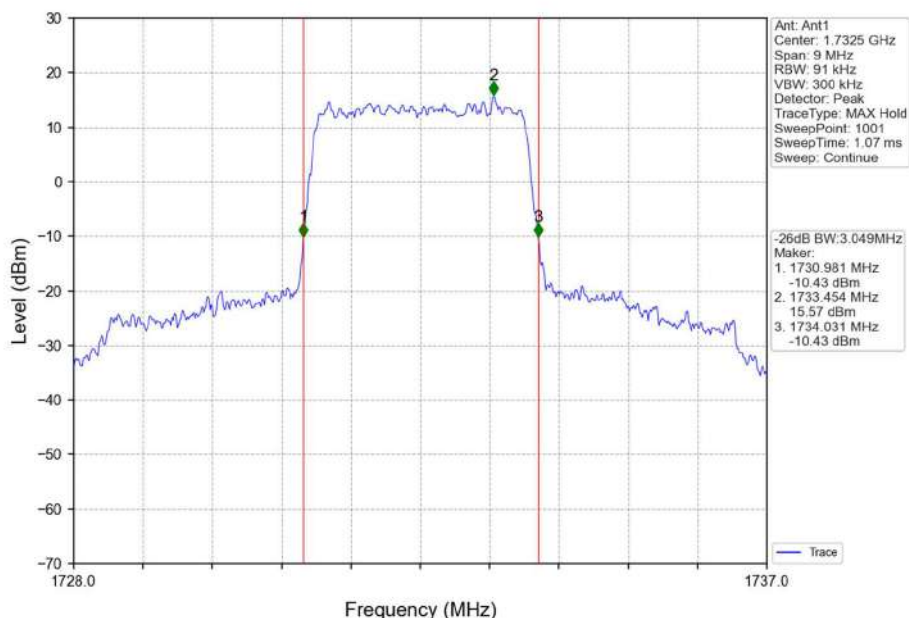
Band4_3MHz_QPSK_MCH_1732.5MHz_RB_15_0_NTNV
