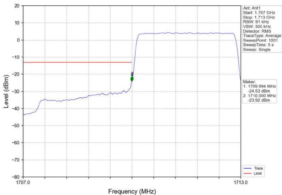
Band4_3MHz_QPSK_LCH_1711.5MHz_RB_15_0_NTNV
