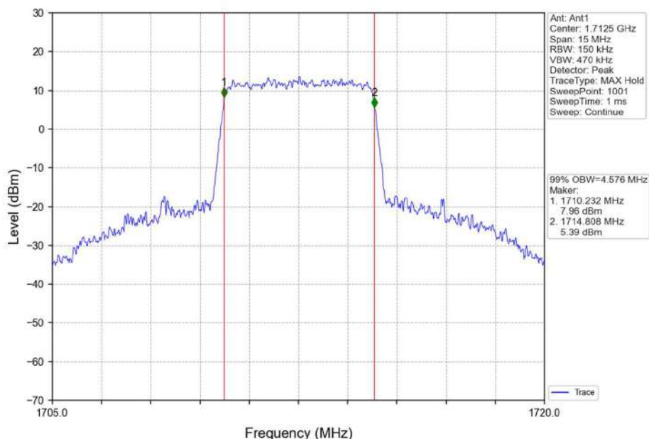
Band4_5MHz_16QAM_LCH_1712.5MHz_RB_25_0_NTNV
