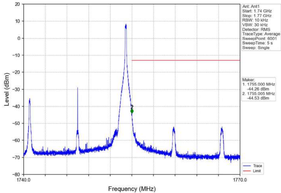
Band4_15MHz_16QAM_HCH_1747.5MHz_RB_1_74_NTNV
