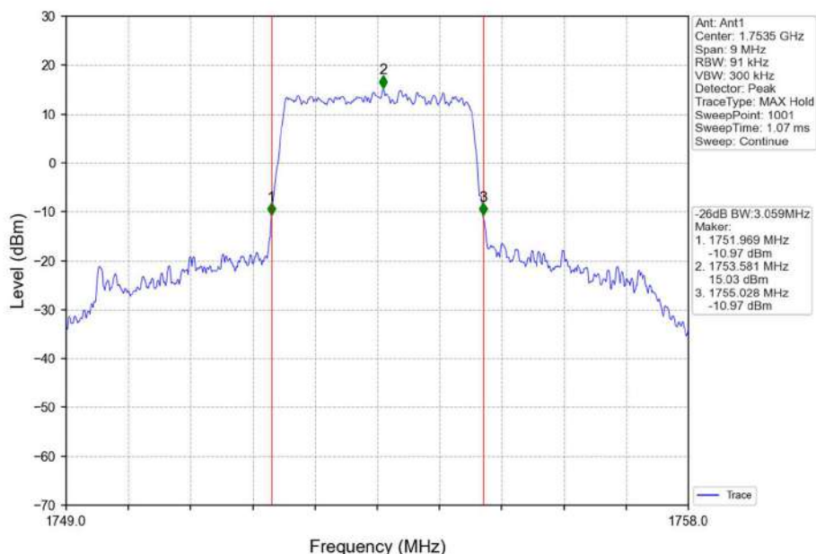
Band4_3MHz_QPSK_HCH_1753.5MHz_RB_15_0_NTNV
