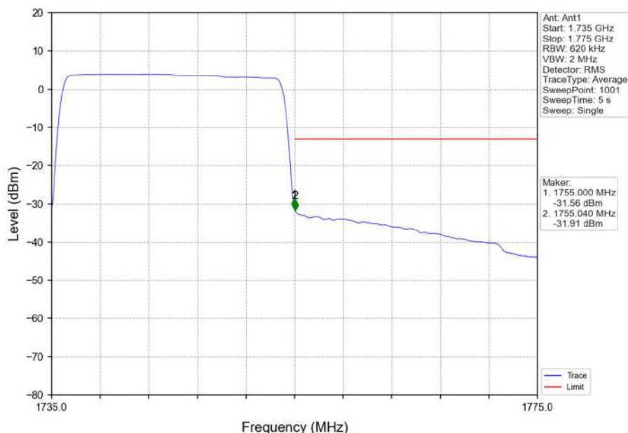
Band4_20MHz_16QAM_HCH_1745MHz_RB_100_0_NTNV
