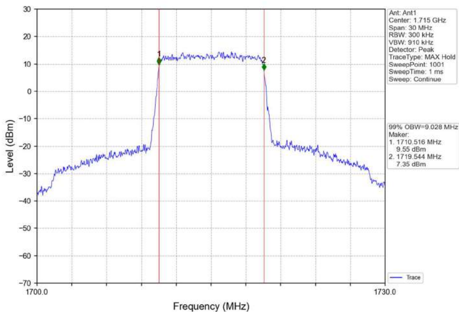
Band4_10MHz_QPSK_LCH_1715MHz_RB_50_0_NTNV
