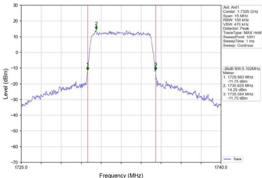
Band4_5MHz_16QAM_MCH_1732.5MHz_RB_25_0_NTNV
