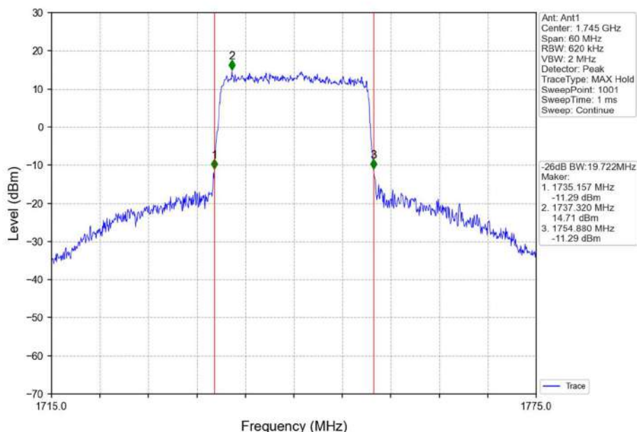
Band4_20MHz_16QAM_HCH_1745MHz_RB_100_0_NTNV
