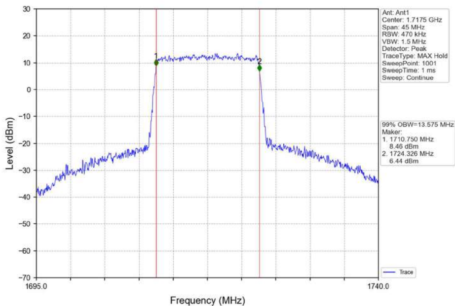
Band4_15MHz_16QAM_LCH_1717.5MHz_RB_75_0_NTNV
