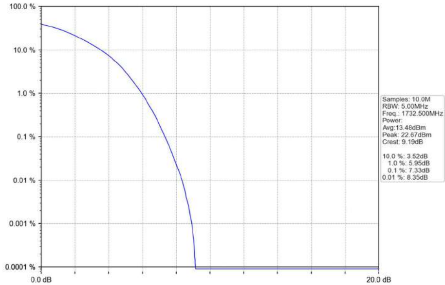
Band4_15MHz_16QAM_MCH_1732.5MHz_RB_75_0_NTNV
