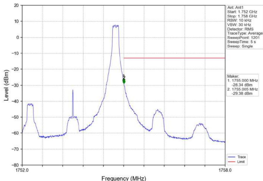
Band4_3MHz_16QAM_HCH_1753.5MHz_RB_1_14_NTNV
