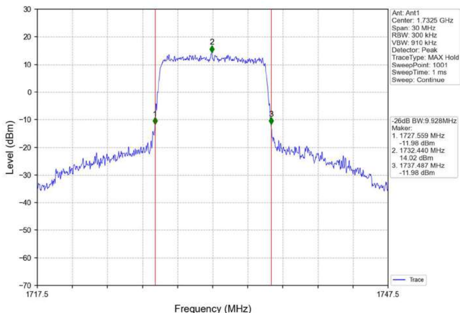
Band4_10MHz_16QAM_MCH_1732.5MHz_RB_50_0_NTNV
