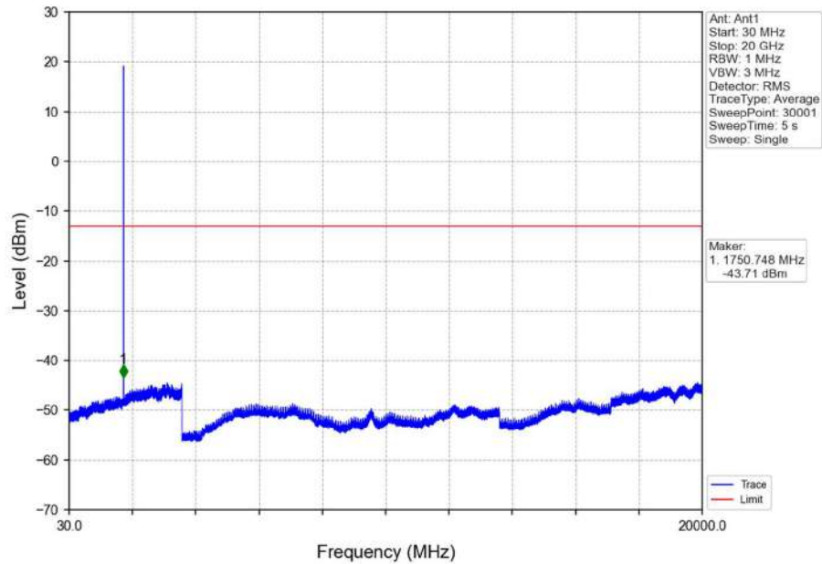
Band4_1.4MHz_QPSK_HCH_1754.3MHz_RB_1_0_NTNV
