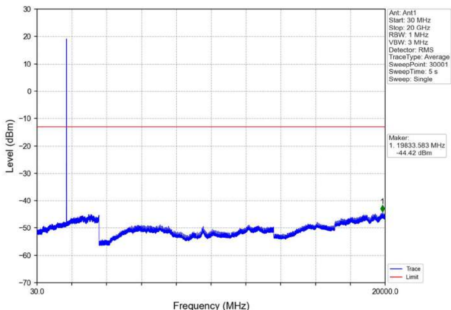
Band4_5MHz_QPSK_MCH_1732.5MHz_RB_1_0_NTNV
