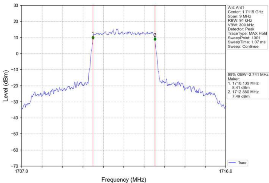
Band4_3MHz_QPSK_LCH_1711.5MHz_RB_15_0_NTNV
