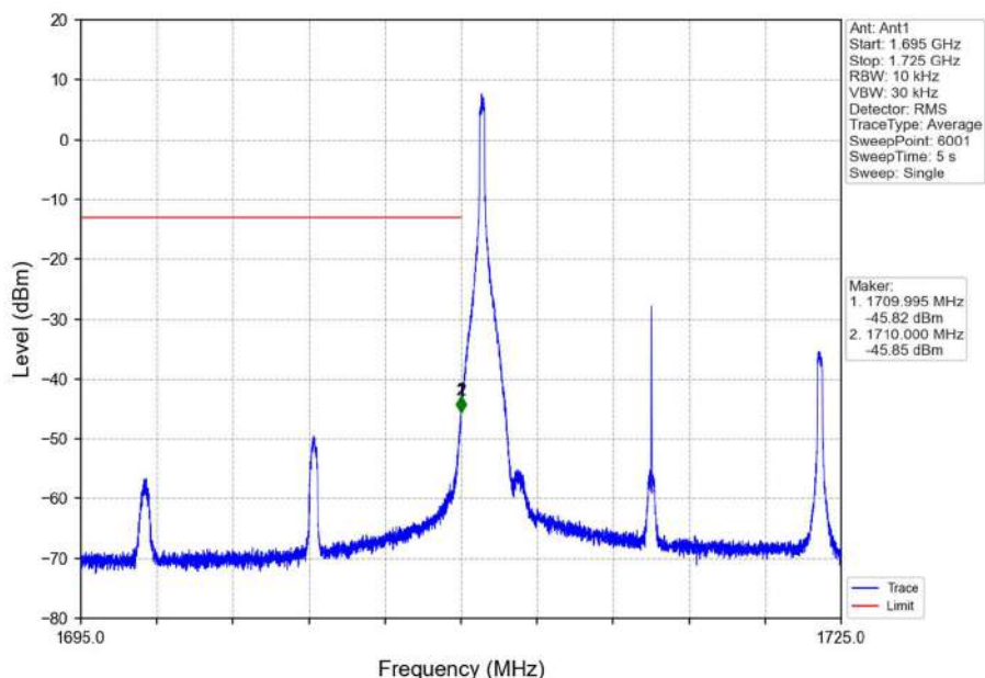
Band4_15MHz_16QAM_LCH_1717.5MHz_RB_1_0_NTNV
