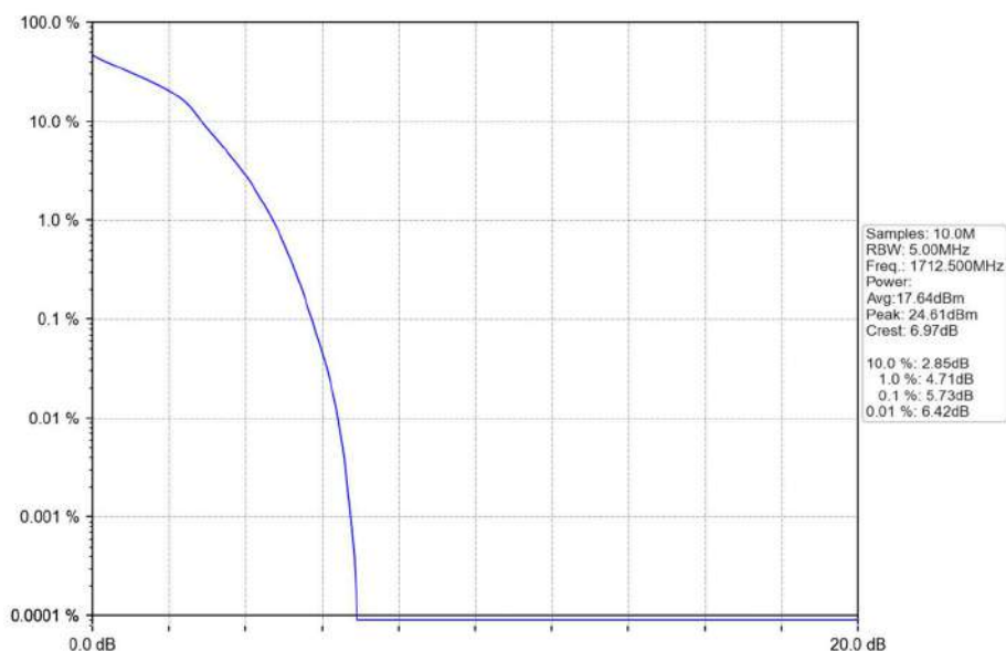
Band4_5MHz_16QAM_LCH_1712.5MHz_RB_25_0_NTNV
