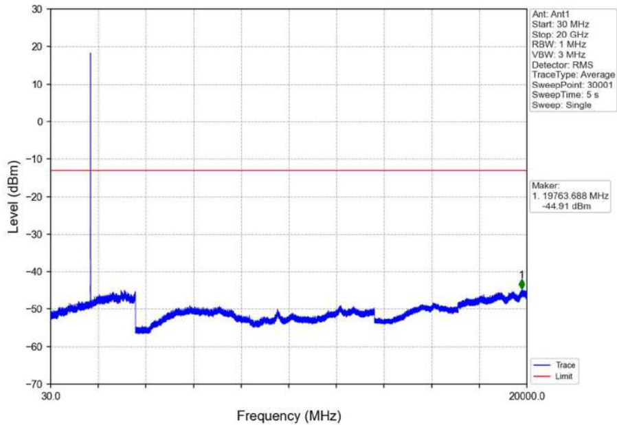
Band4_3MHz_16QAM_LCH_1711.5MHz_RB_1_0_NTNV
