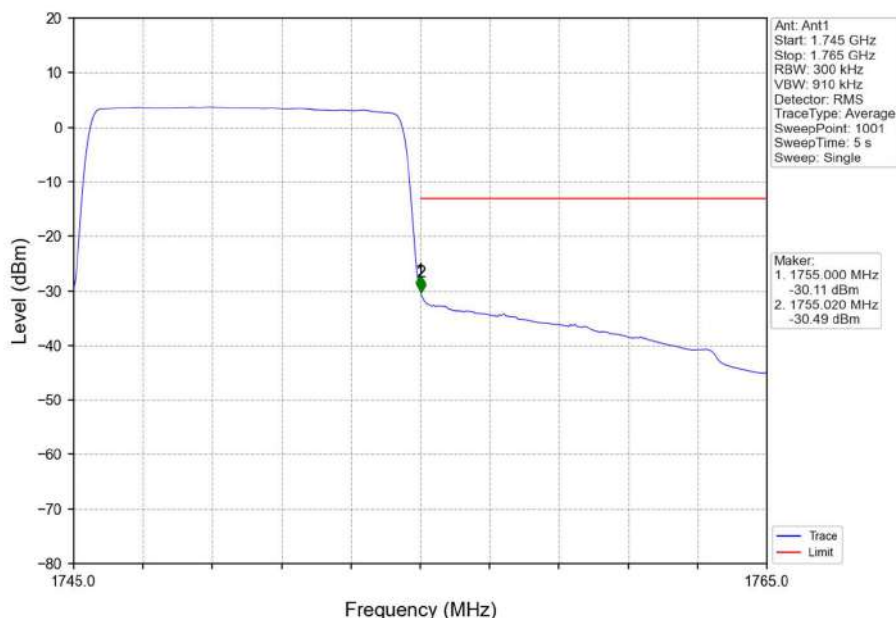
Band4_10MHz_16QAM_HCH_1750MHz_RB_50_0_NTNV
