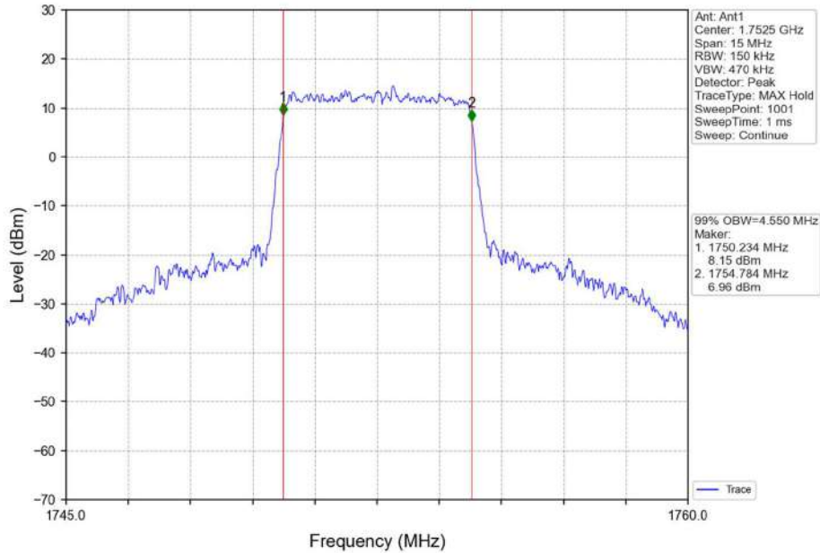
Band4_5MHz_16QAM_HCH_1752.5MHz_RB_25_0_NTNV
