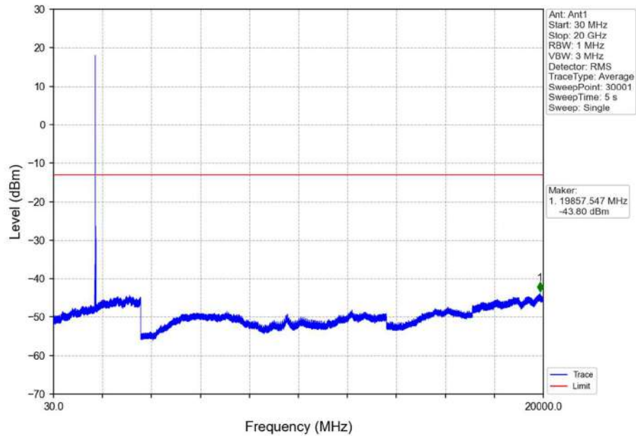
Band4_15MHz_16QAM_HCH_1747.5MHz_RB_1_0_NTNV
