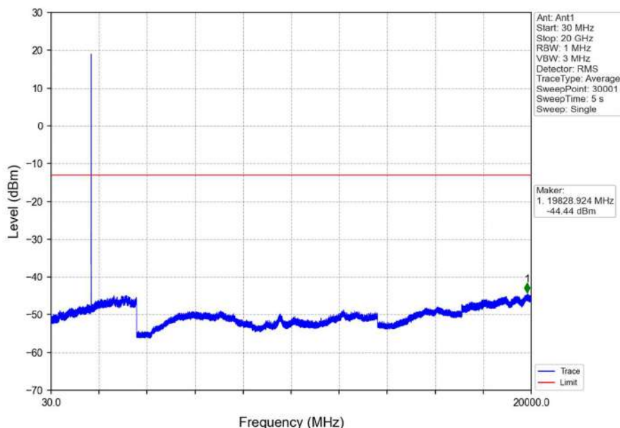
Band4_3MHz_QPSK_LCH_1711.5MHz_RB_1_0_NTNV
