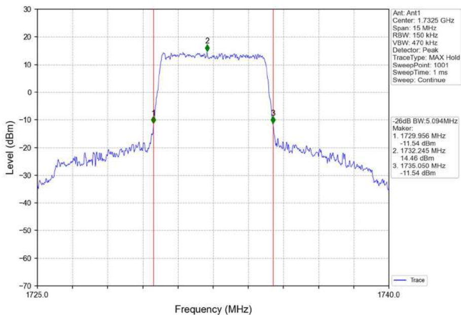
Band4_5MHz_QPSK_MCH_1732.5MHz_RB_25_0_NTNV
