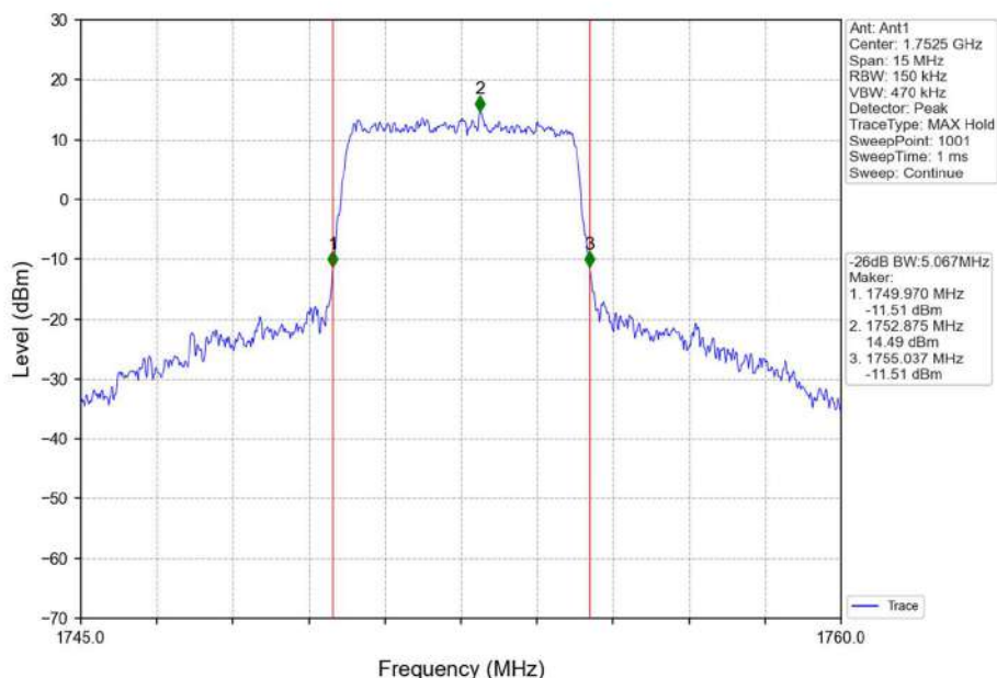
Band4_5MHz_16QAM_HCH_1752.5MHz_RB_25_0_NTNV
