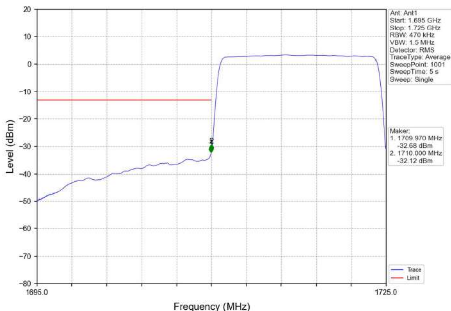
Band4_15MHz_16QAM_LCH_1717.5MHz_RB_75_0_NTNV
