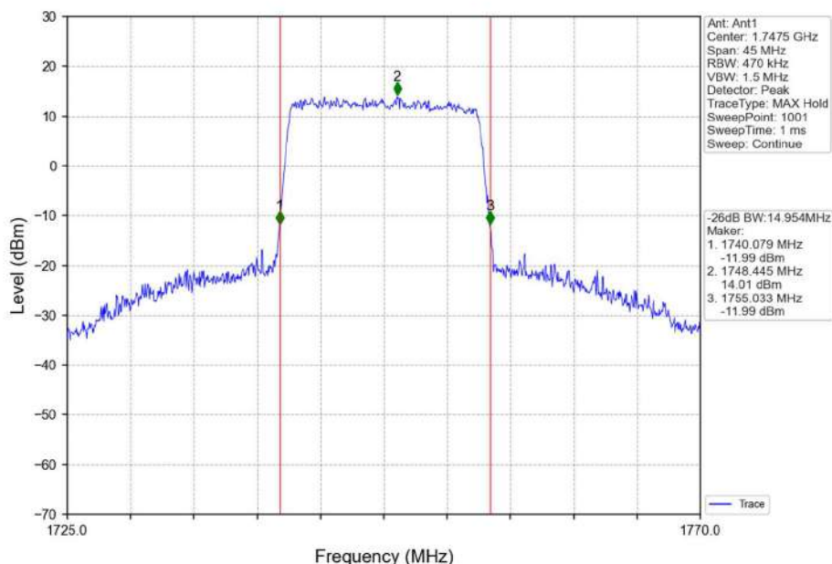
Band4_15MHz_16QAM_HCH_1747.5MHz_RB_75_0_NTNV
