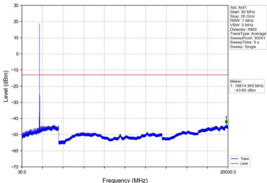
Band4_15MHz_QPSK_HCH_1747.5MHz_RB_1_0_NTNV
