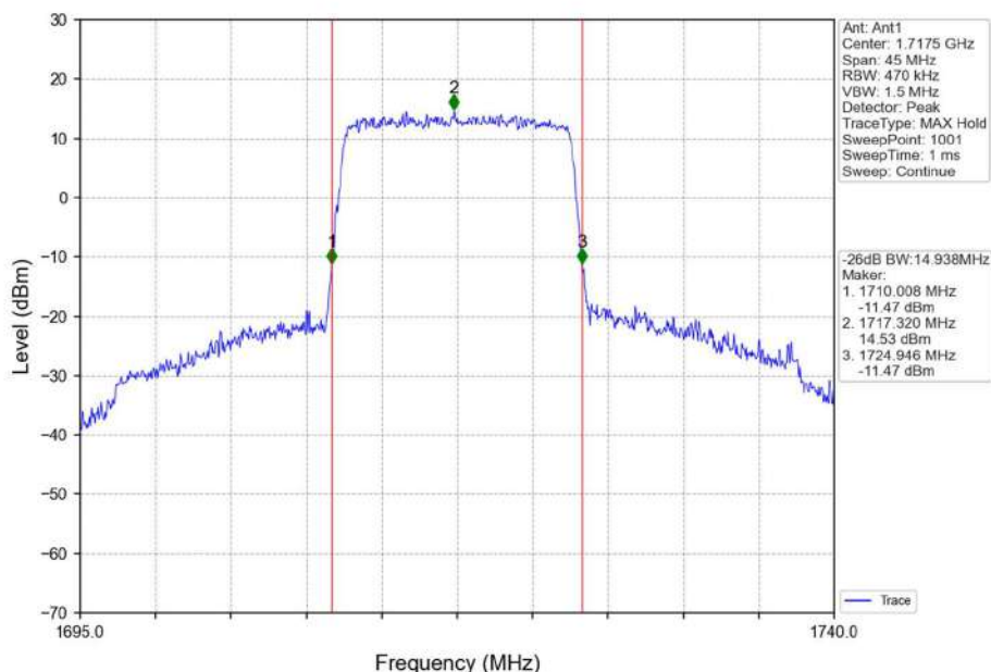
Band4_15MHz_QPSK_LCH_1717.5MHz_RB_75_0_NTNV
