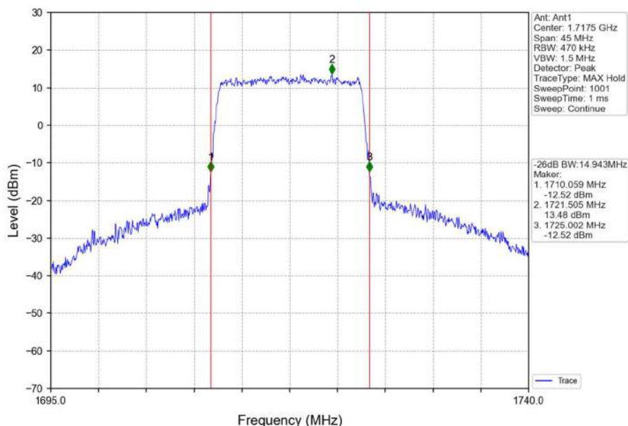
Band4_15MHz_16QAM_LCH_1717.5MHz_RB_75_0_NTNV
