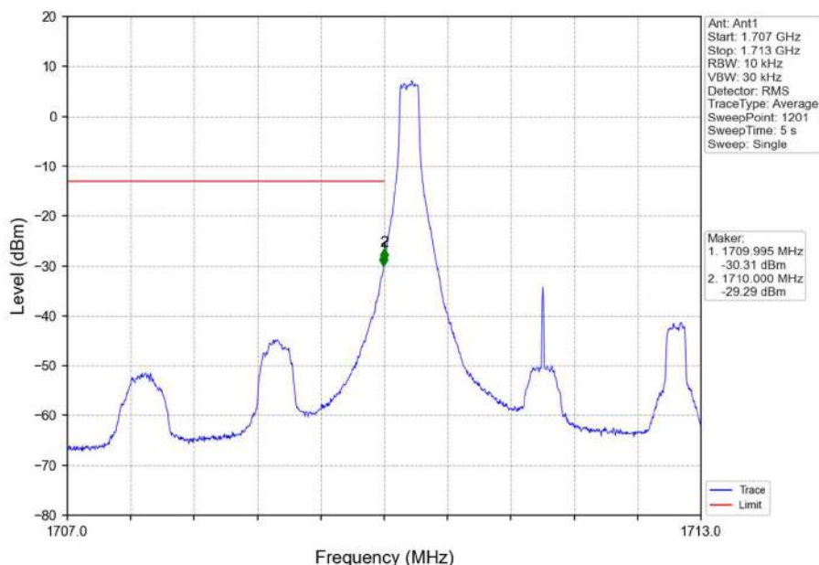
Band4_3MHz_16QAM_LCH_1711.5MHz_RB_1_0_NTNV
