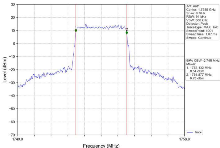
Band4_3MHz_16QAM_HCH_1753.5MHz_RB_15_0_NTNV
