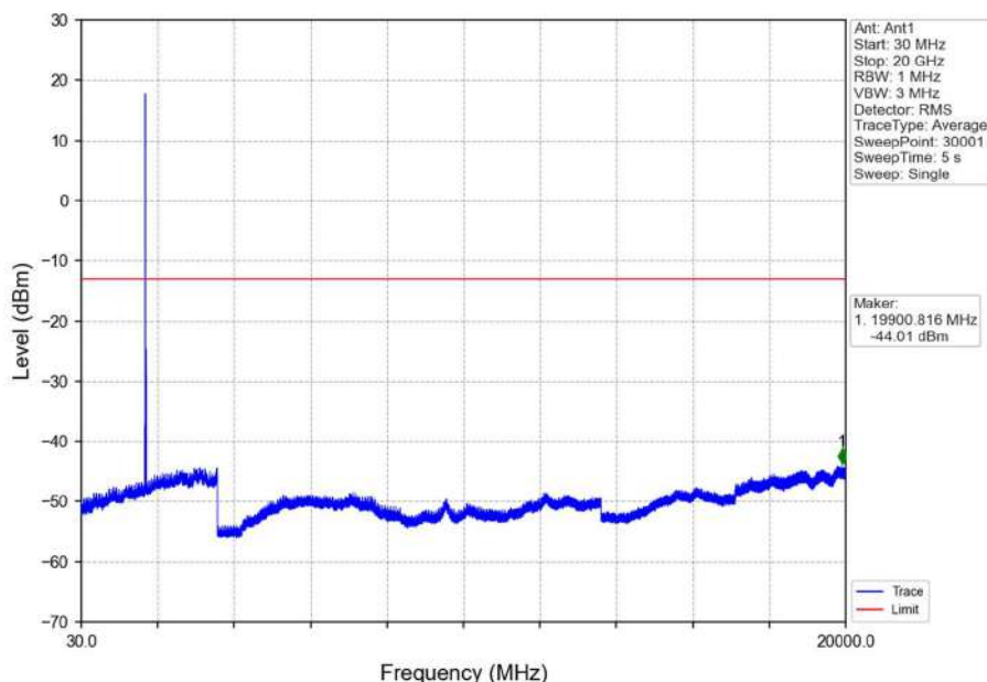
Band4_15MHz_16QAM_LCH_1717.5MHz_RB_1_0_NTNV
