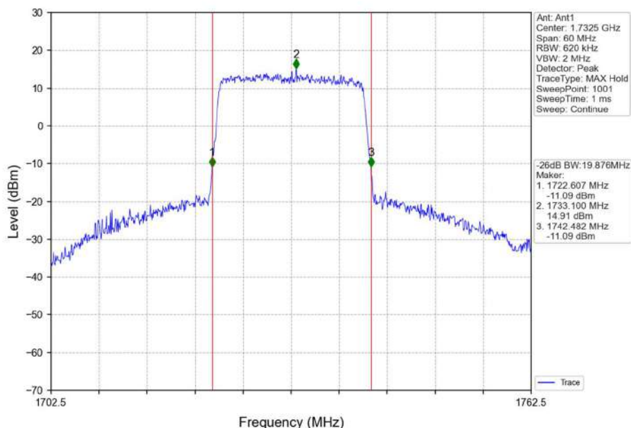
Band4_20MHz_16QAM_MCH_1732.5MHz_RB_100_0_NTNV
