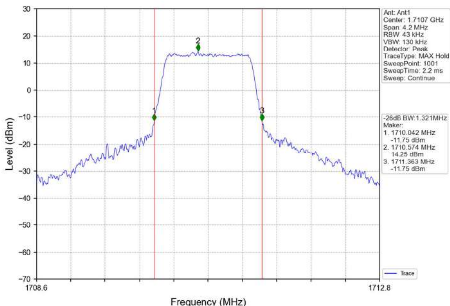
Band4_1.4MHz_16QAM_LCH_1710.7MHz_RB_6_0_NTNV
