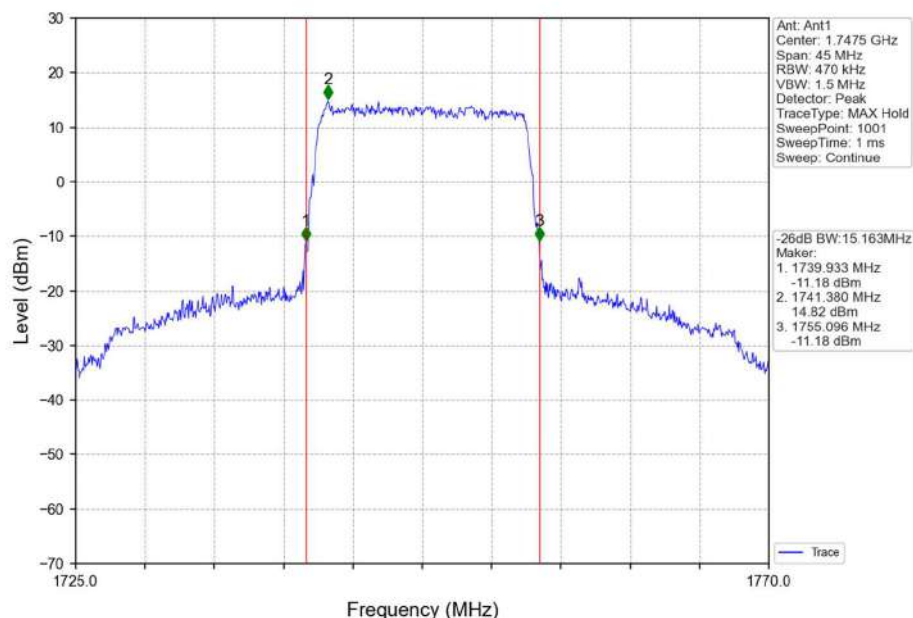
Band4_15MHz_QPSK_HCH_1747.5MHz_RB_75_0_NTNV
