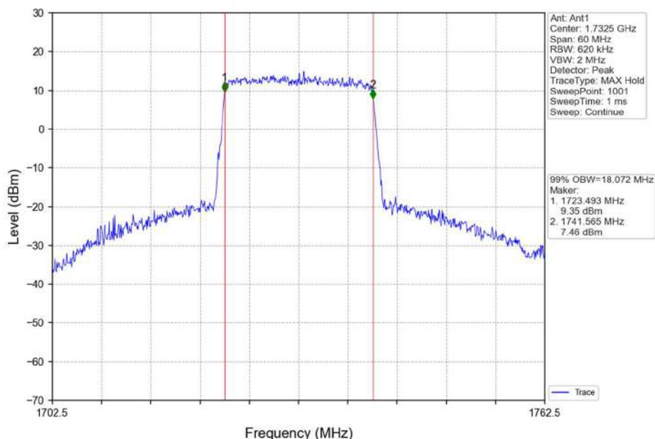
Band4_20MHz_16QAM_MCH_1732.5MHz_RB_100_0_NTNV
