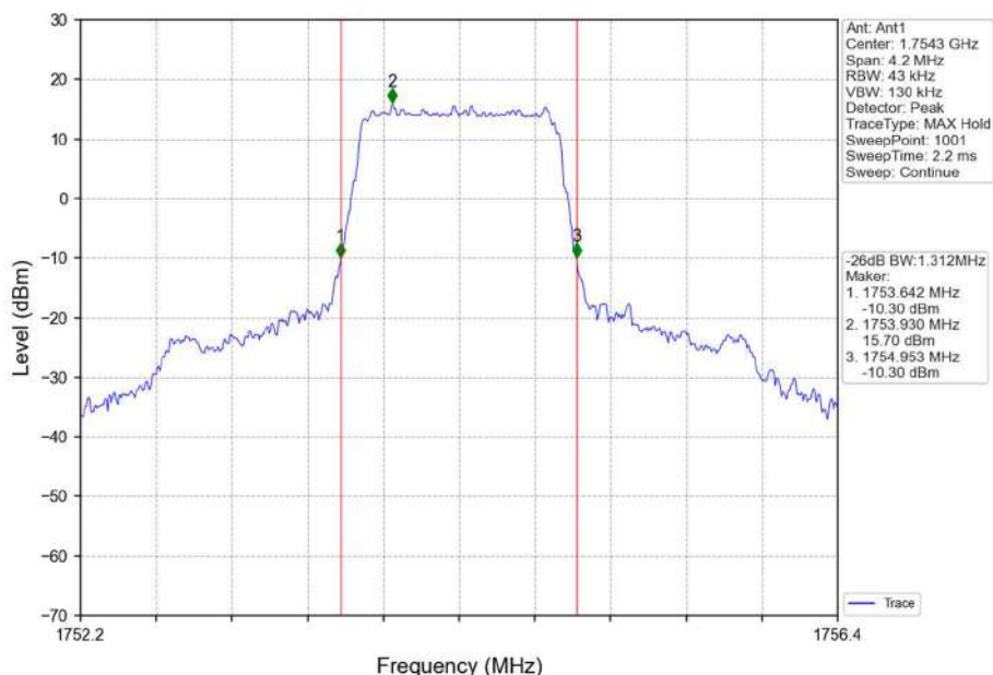
Band4_1.4MHz_QPSK_HCH_1754.3MHz_RB_6_0_NTNV
