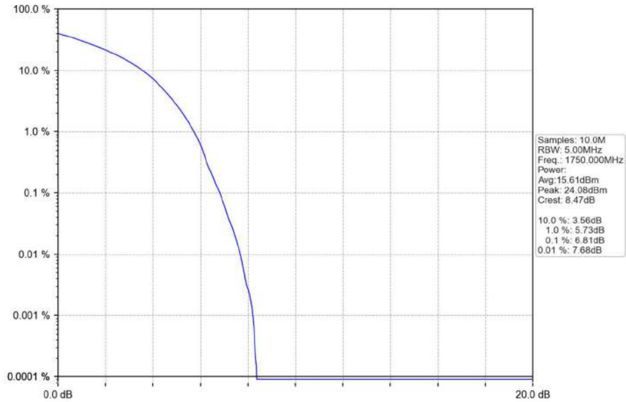
Band4_10MHz_16QAM_HCH_1750MHz_RB_50_0_NTNV
