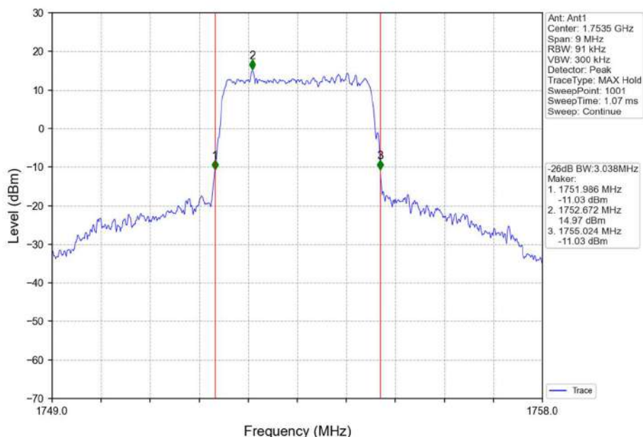
Band4_3MHz_16QAM_HCH_1753.5MHz_RB_15_0_NTNV
