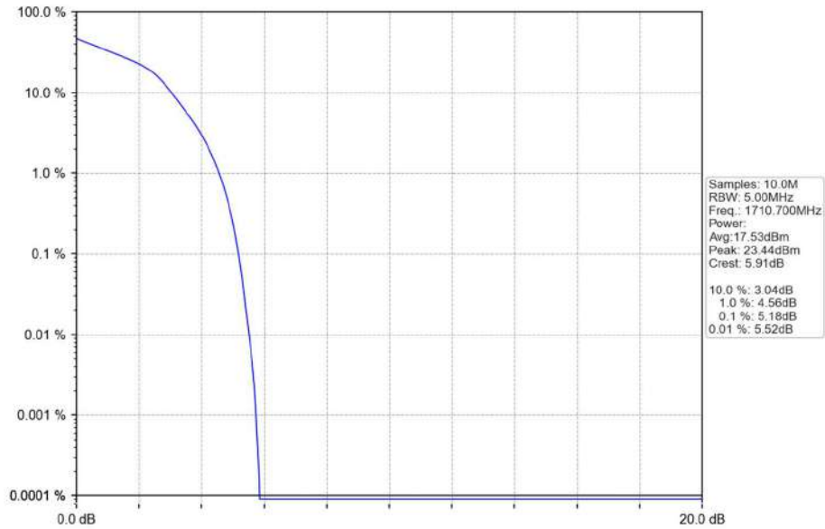
Band4_1.4MHz_16QAM_LCH_1710.7MHz_RB_6_0_NTNV
