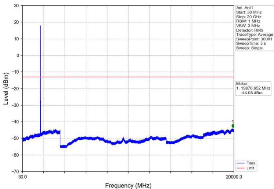
Band4_15MHz_QPSK_MCH_1732.5MHz_RB_1_0_NTNV
