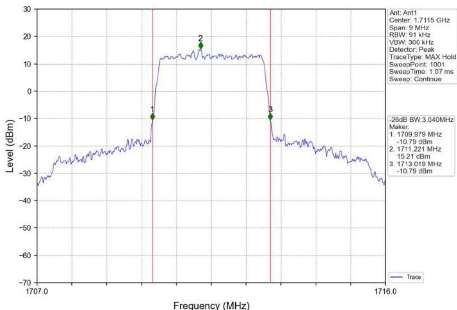
Band4_3MHz_QPSK_LCH_1711.5MHz_RB_15_0_NTNV
