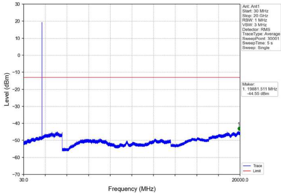
Band4_1.4MHz_QPSK_MCH_1732.5MHz_RB_1_0_NTNV
