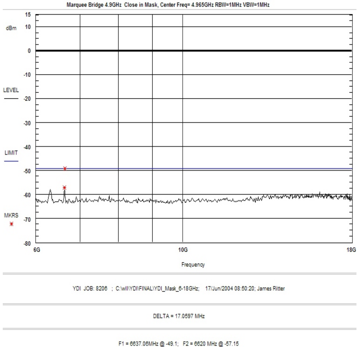
Figure 8. Spurious Emissions, 6G – 18GHz
