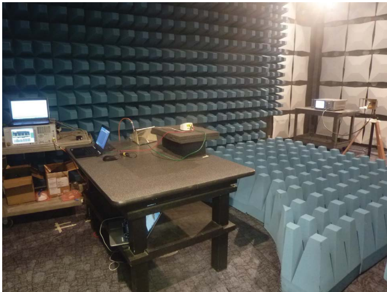
Figure 22: DFS Test Setup Photo for Master – Radiated Method – View 2
