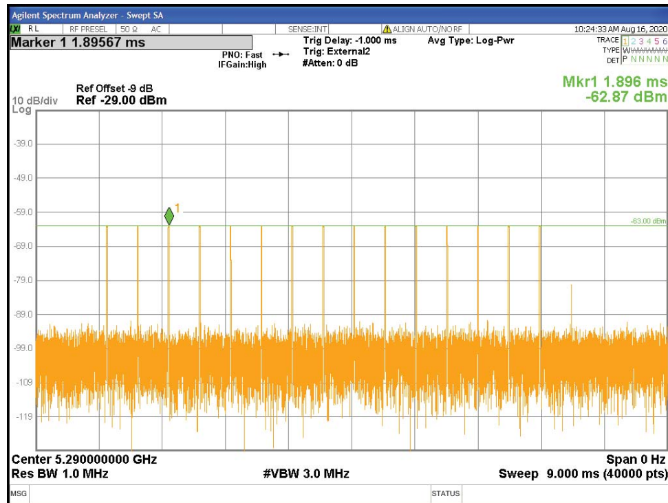
Figure 6: Radar Type 4 DFS Detection Threshold Level at 5290 MHz
