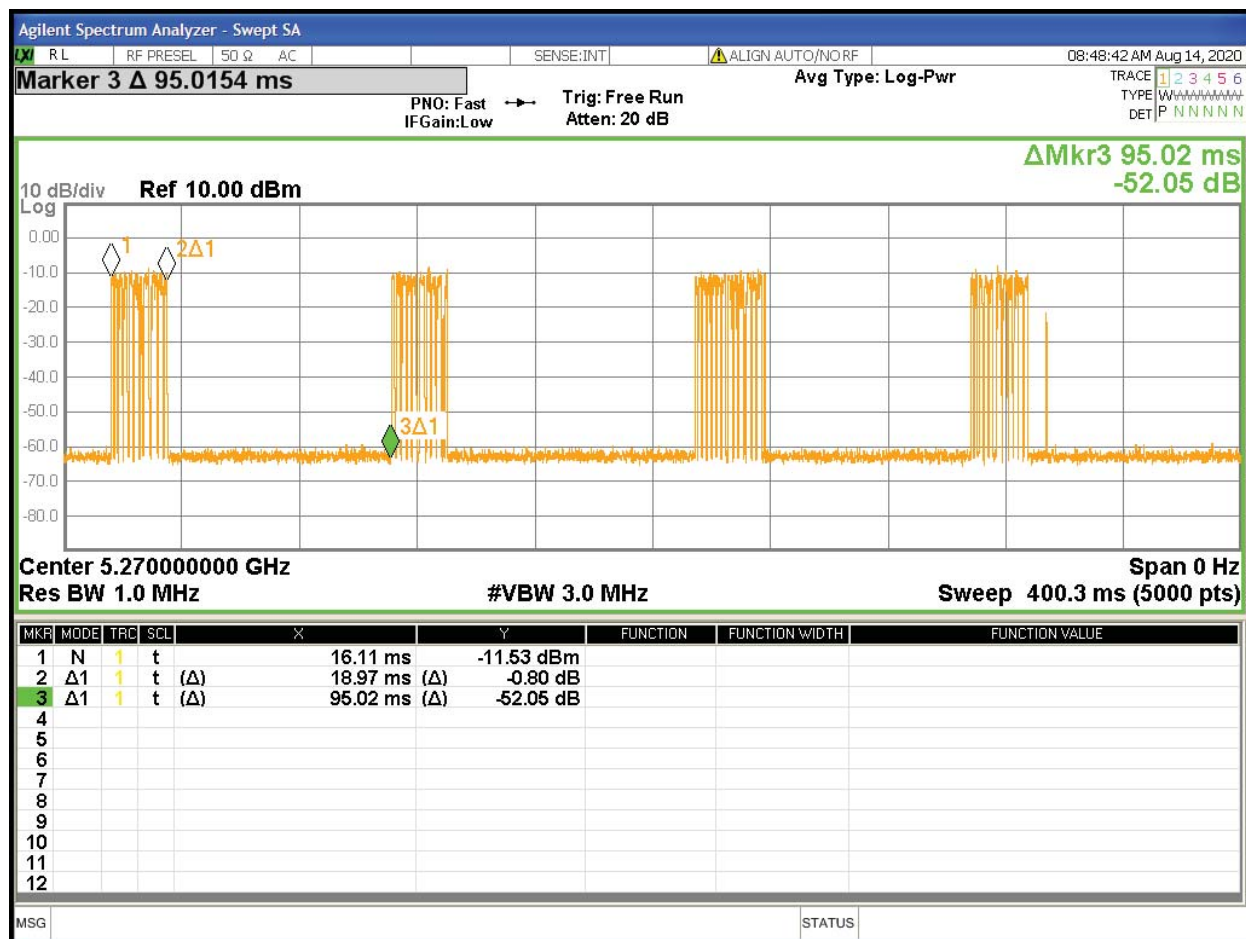
Figure 10: EUT Channel Loading at 5270 MHz. (40 MHz bandwidth)
