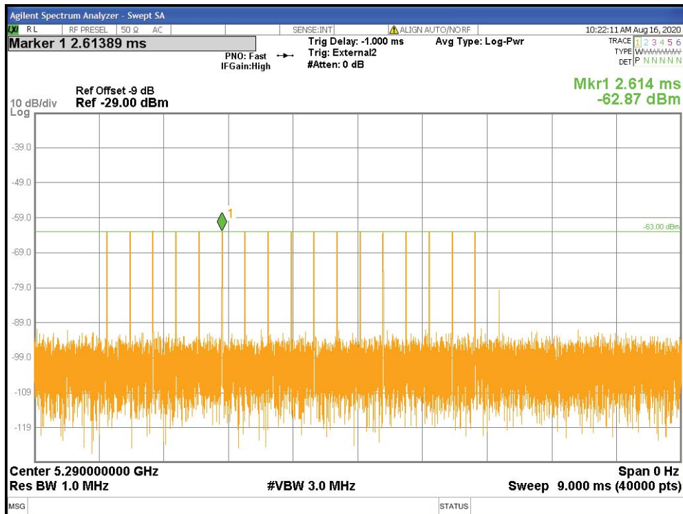
Figure 5: Radar Type 3 DFS Detection Threshold Level at 5290 MHz
