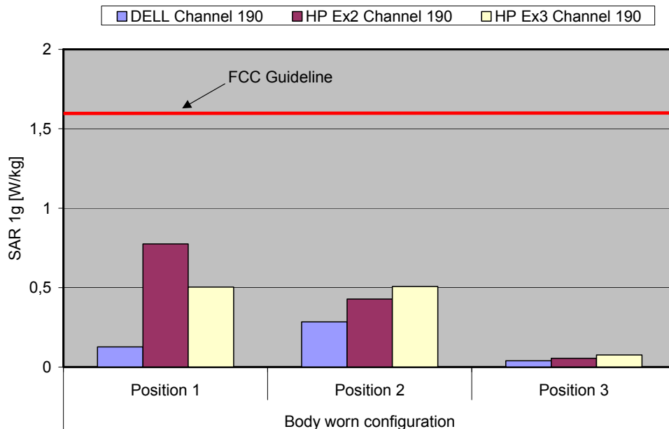
Fig. 8: The measured SAR values for the Option Globetrotter Fusion+ Card in combination with the three host products for GPRS 850 (Class 10) in comparison to the FCC exposure limit.
