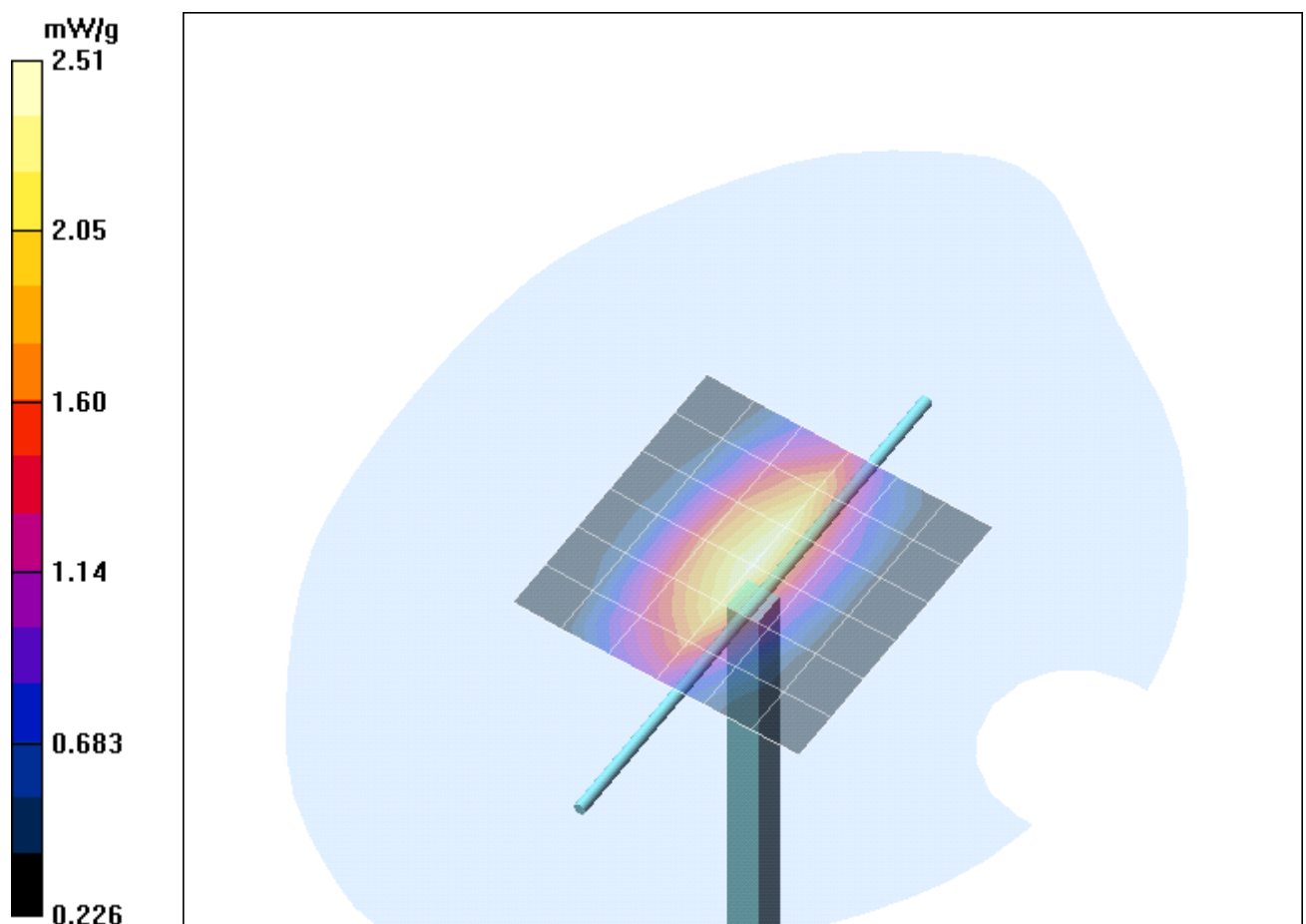
Fig. 10: Validation measurement 835MHz Body (September 19, 2005), coarse grid. Ambient Temperature: 21.1° C, Liquid Temperature: 20.4° C.
