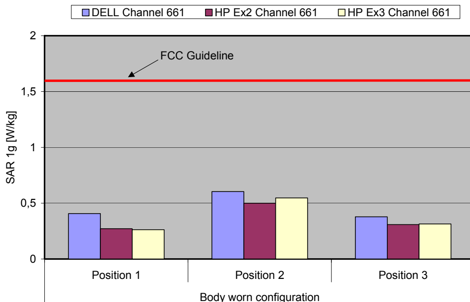
Fig. 9: The measured SAR values for the Option Globetrotter Fusion+ Card in combination with the three host products for GPRS 1900 (Class 10) in comparison to the FCC exposure limit.
