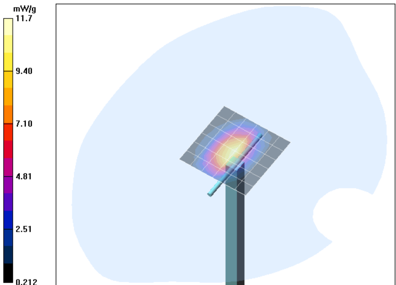
Fig. 11: Validation measurement 1900 MHz Body (September 20, 2005), coarse grid. Ambient Temperature: 21.6° C, Liquid Temperature: 20.8° C.
