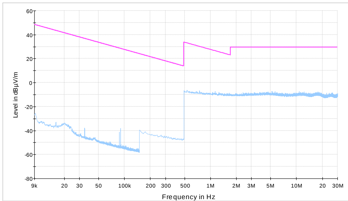
Figure 5: Channel 19 mid 9 kHz – 30 MHz
