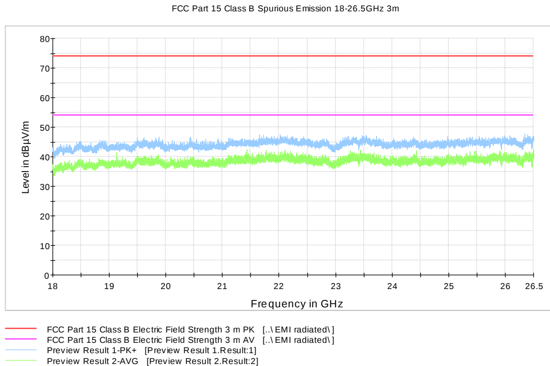
Figure 13: Channel 39 high 18 GHz – 26.5 GHz
