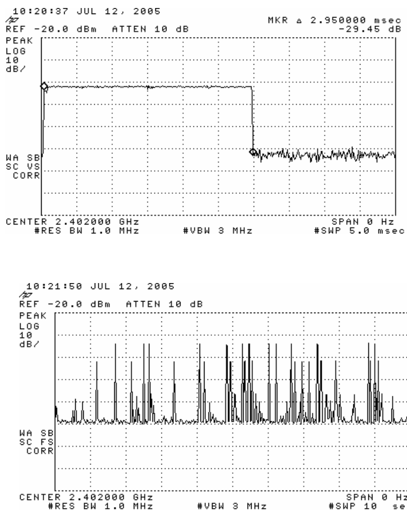
Figure 6.4 Single Channel Dwell Time. (only Low Channel shown)
