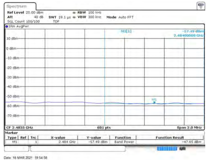
802.11ac-20 MHz HIGH CHANNEL, Reference level
