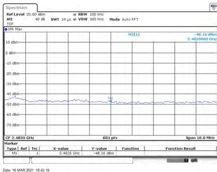
802.11b HIGH CHANNEL, Carrier level
