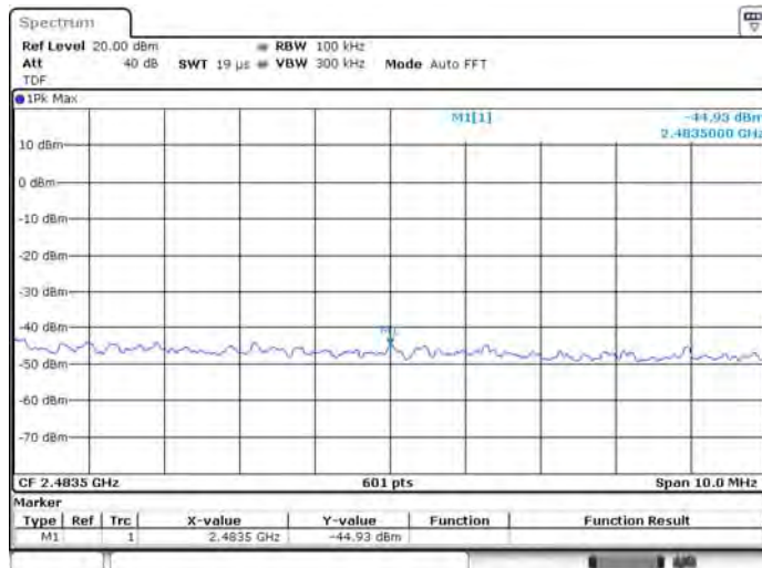
802.11ac-40 MHz HIGH CHANNEL, Carrier level
