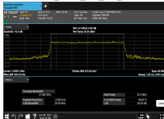
B2_N77(30M)_CP-OFDM_256 QAM_Outer_Full_Mid_CH
