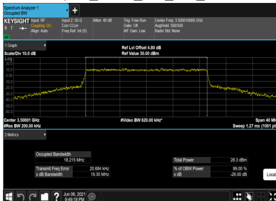
B2_N77(20M)_CP-OFDM_64 QAM_Outer_Full_Mid_CH
