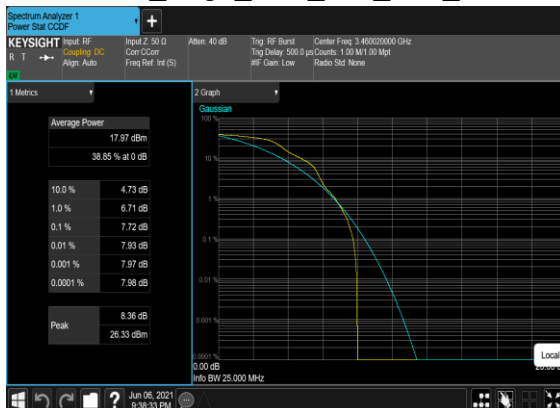
B2_N77(20M)_DFT-s-OFDM_PI_2- BPSK_Edge_1RB_Left_Low_CH
