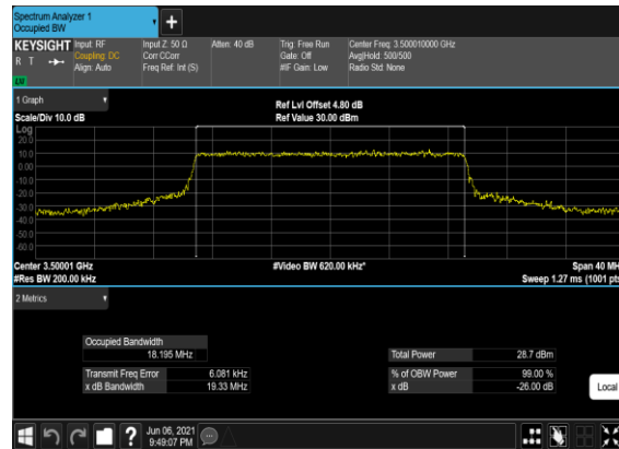
B2_N77(20M)_CP-OFDM_16 QAM_Outer_Full_Mid_CH
