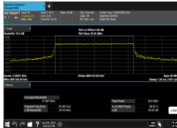
B2_N77(30M)_CP-OFDM_16 QAM_Outer_Full_Mid_CH
