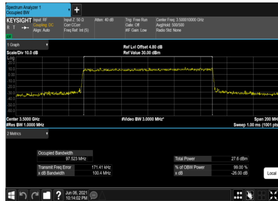
B2_N77(100M)_CP-OFDM_16 QAM_Outer_Full_Low_CH
