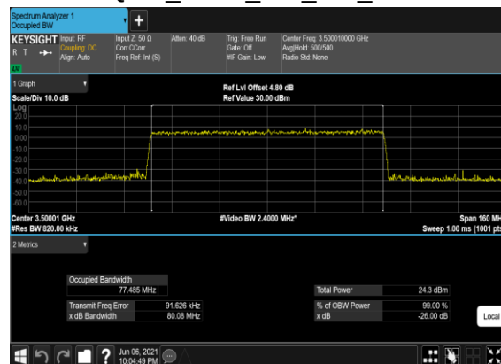
B2_N77(80M)_CP-OFDM_256 QAM_Outer_Full_Mid_CH
