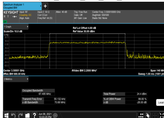
B2_N77(70M)_CP-OFDM_256 QAM_Outer_Full_Mid_CH
