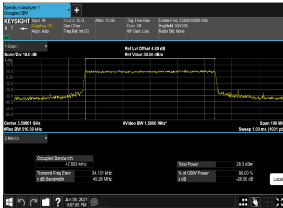
B2_N77(50M)_CP- OFDM_QPSK_Outer_Full_Mid_CH
