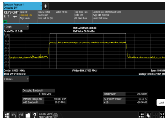
B2_N77(90M)_CP-OFDM_256 QAM_Outer_Full_Mid_CH
