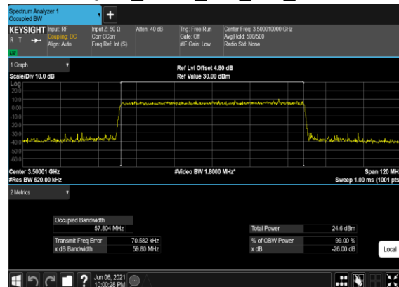
B2_N77(60M)_CP-OFDM_256 QAM_Outer_Full_Mid_CH
