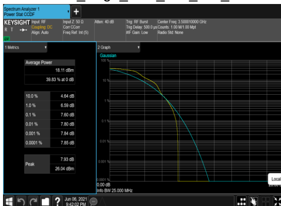
B2_N77(20M)_DFT-s-OFDM_PI_2- BPSK_Edge_1RB_Left_Mid_CH
