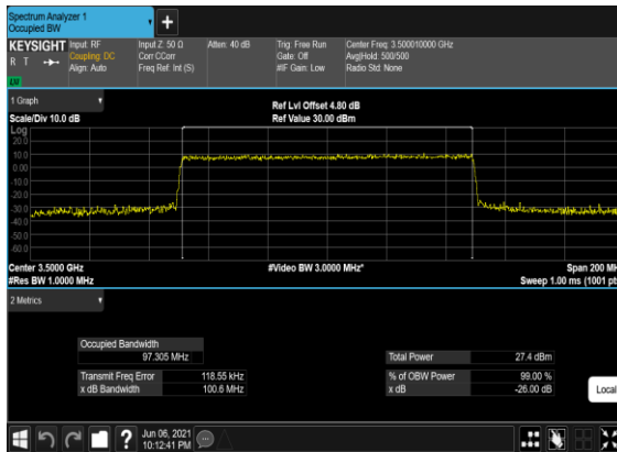
B2_N77(100M)_CP- OFDM_QPSK_Outer_Full_Low_CH
