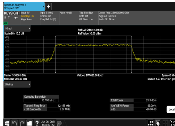
B2_N77(20M)_CP-OFDM_256 QAM_Outer_Full_Mid_CH
