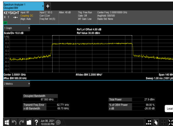
B2_N77(70M)_CP-OFDM_16 QAM_Outer_Full_Mid_CH
