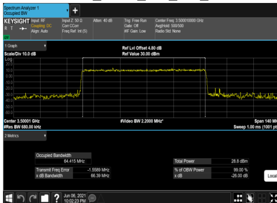
B2_N77(70M)_DFT-s-OFDM_PI_2- BPSK_Outer_Full_Mid_CH
