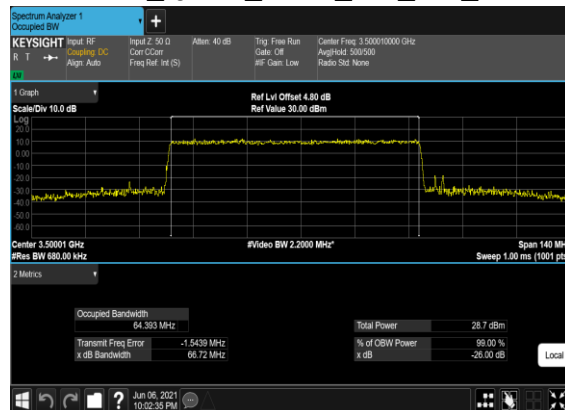
B2_N77(70M)_DFT-s- OFDM_QPSK_Outer_Full_Mid_CH
