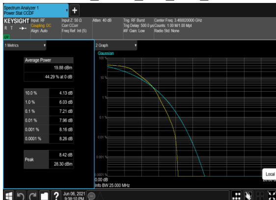
B2_N77(20M)_DFT-s-OFDM_PI_2- BPSK_Outer_Full_Low_CH
