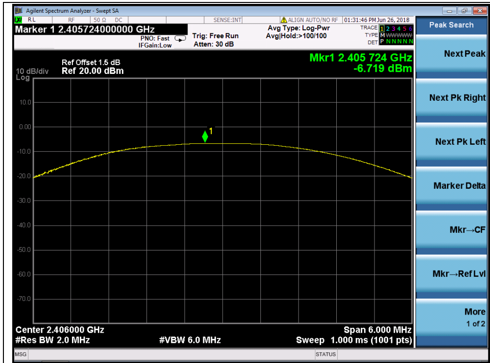
(Channel 1, 2406MHz)
