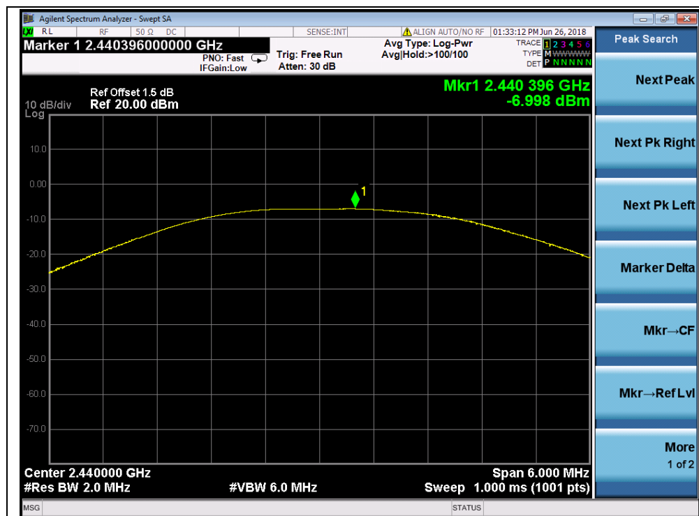
(Channel 3, 2440MHz)
