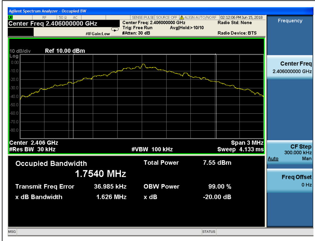
(Channel 1, 2406MHz)
