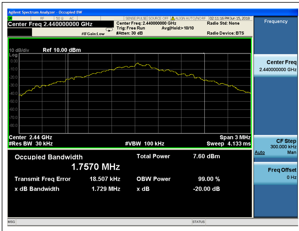
(Channel 3, 2440 MHz)
