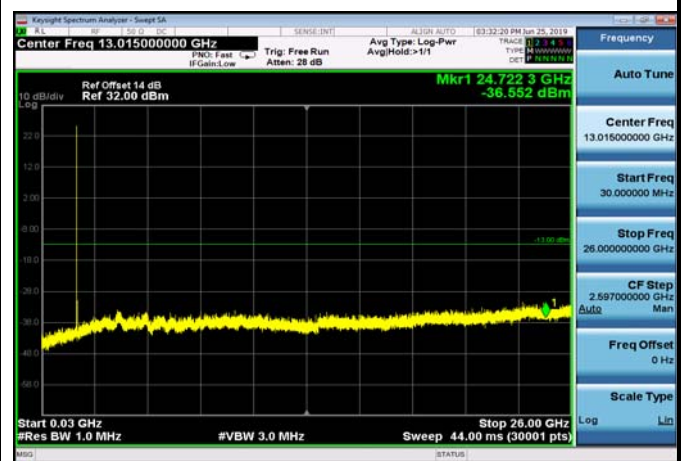
FDD04_HighRange_5MHz_30MHz~26GHz
