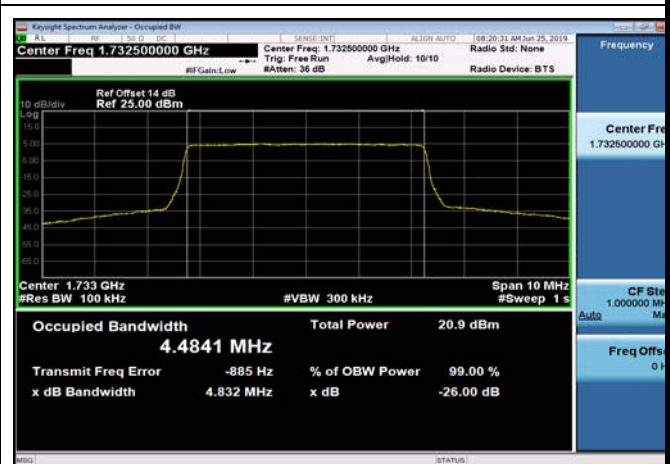
FDD04_MidRange_5MHz_1732.5MHz_QPSK
