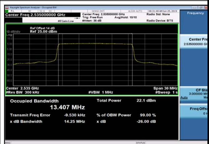
FDD07_MidRange_15MHz_2535MHz_QPSK
