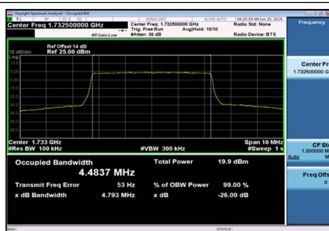
FDD04_MidRange_5MHz_1732.5MHz_Q16
