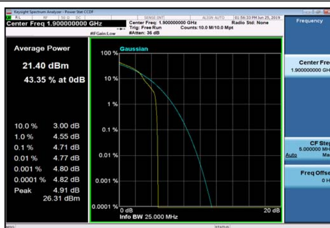
FDD02_HighRange_20MHz_1900_OneRB _high_Q16
