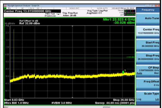
FDD05_HighRange_10MHz_30MHz~26GHz
