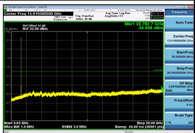
FDD04_MidRange_10MHz_30MHz~26GHz
