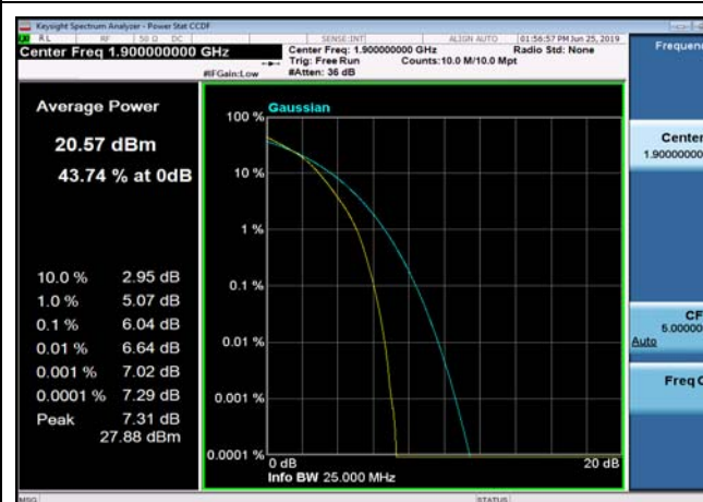
FDD02_HighRange_20MHz_1900_fullRB _Q16
