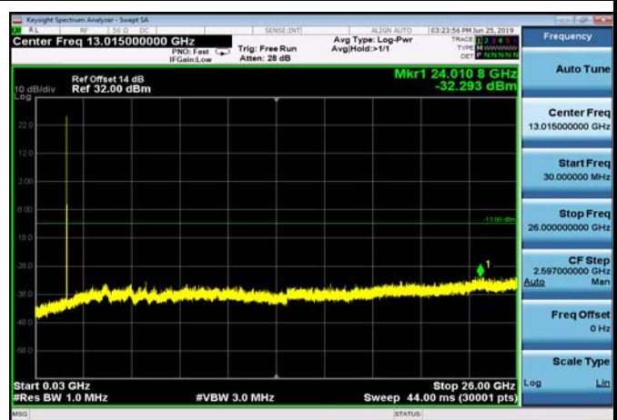
FDD04_LowRange_5MHz_30MHz~26GHz
