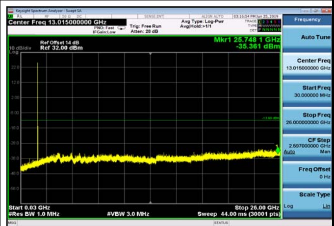
FDD04_HighRange_20MHz_30MHz~26GHz
