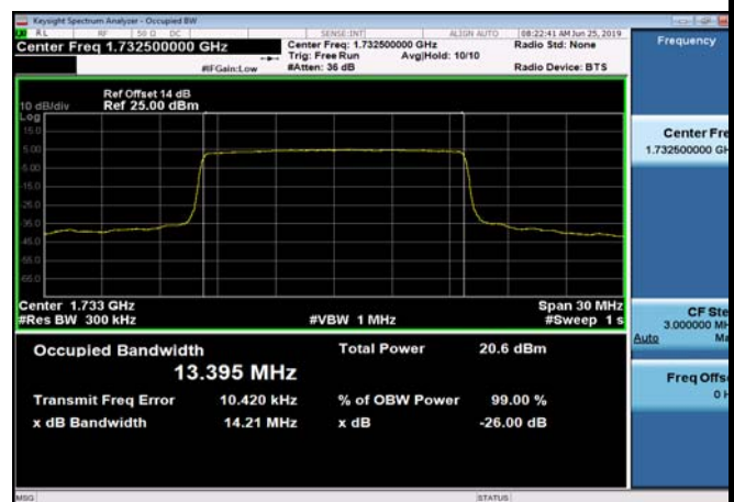
FDD04_MidRange_15MHz_1732.5MHz _QPSK
