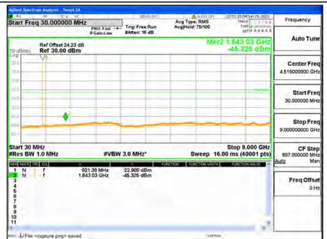
26 Part90 / 3MHz / High CH / QPSK
