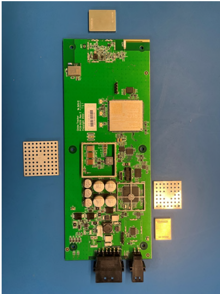
PCB Top – Shields removed
