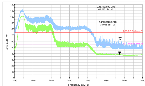
802.11ax HE40 26-Tone-CH9 Peak+ Average
