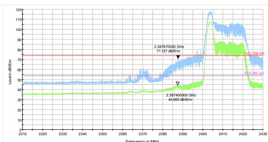
802.11ax HE20 26-Tone-CH1 Peak+ Average
