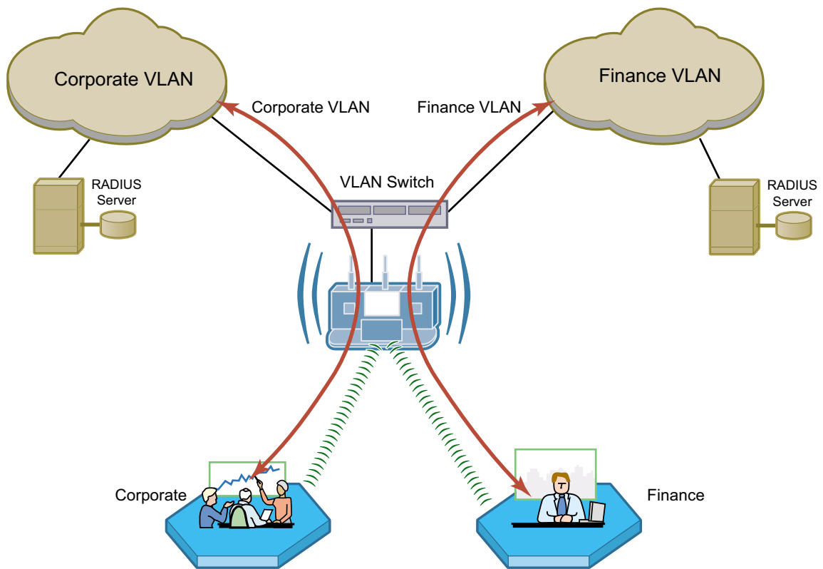
Figure 9: Example 3 Network
