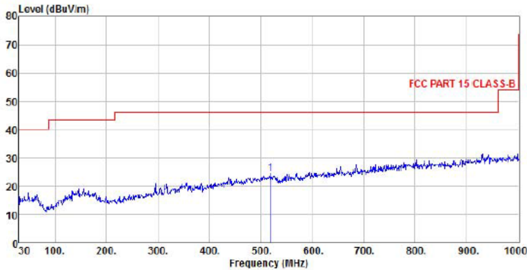
EGPRS1900 Normal Voltage Condition at Middle Channel
