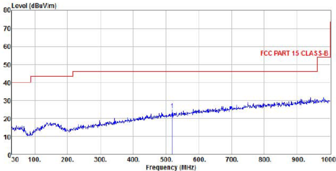
EGPRS850 Normal Voltage Condition at Middle Channel
