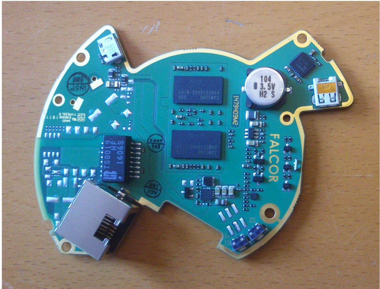
Main PCBA, upper side.
