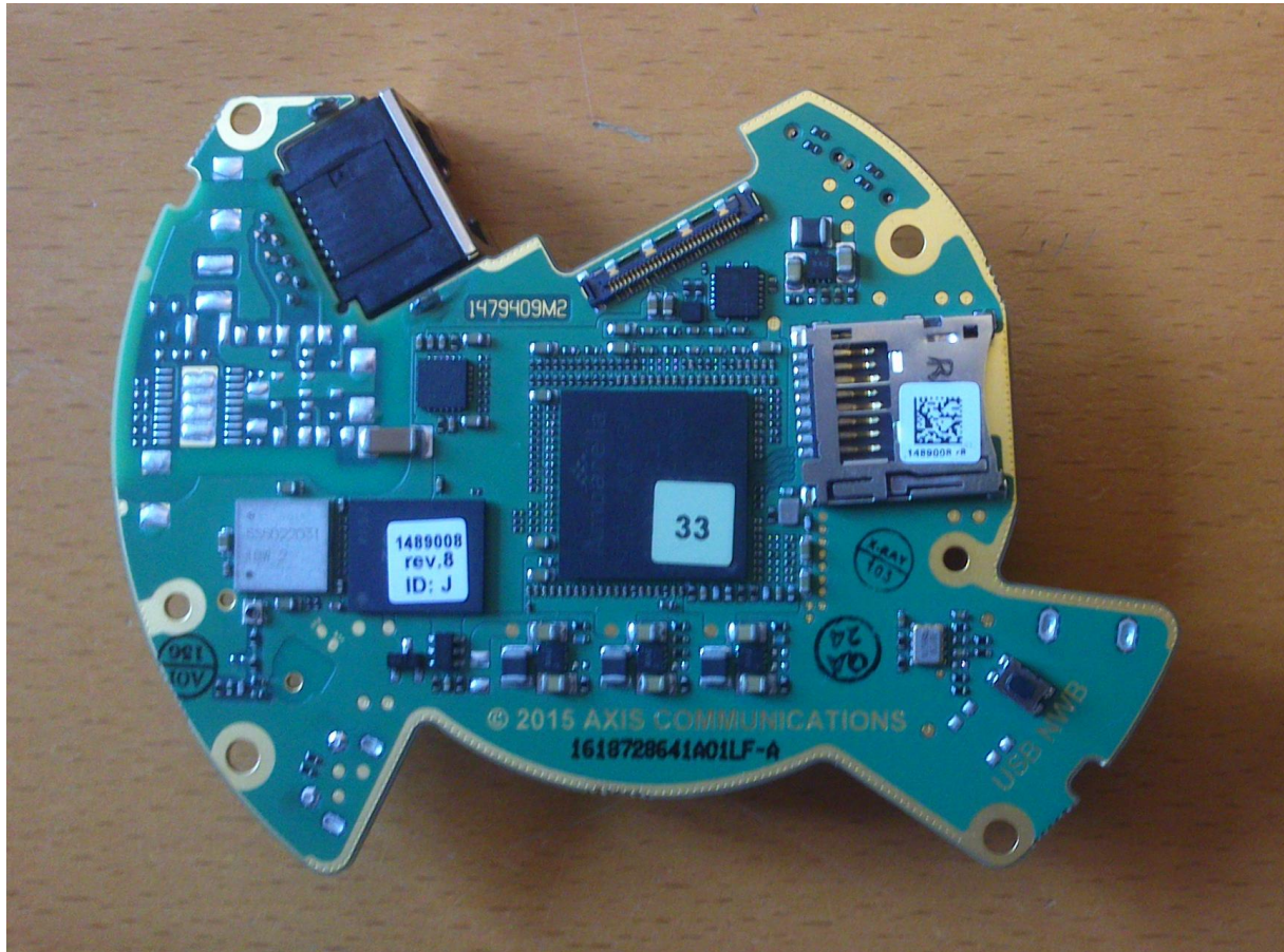
Main PCBA, lower side.
