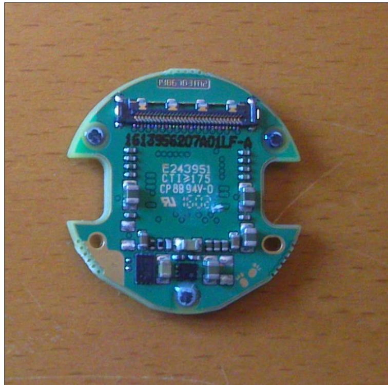
Daughter PCBA, lower side.
