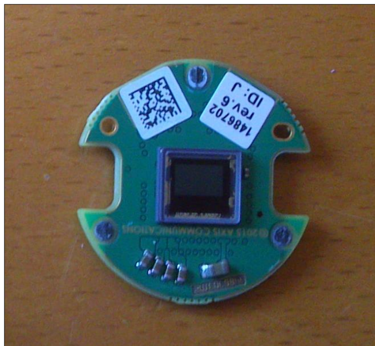
Daughter PCBA, upper side.
