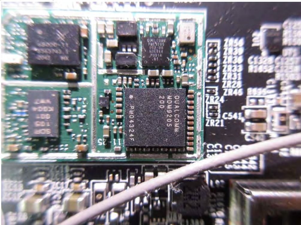
(18) EUT Photo (WWAN Module, FCC ID: NKRIMQ7)
