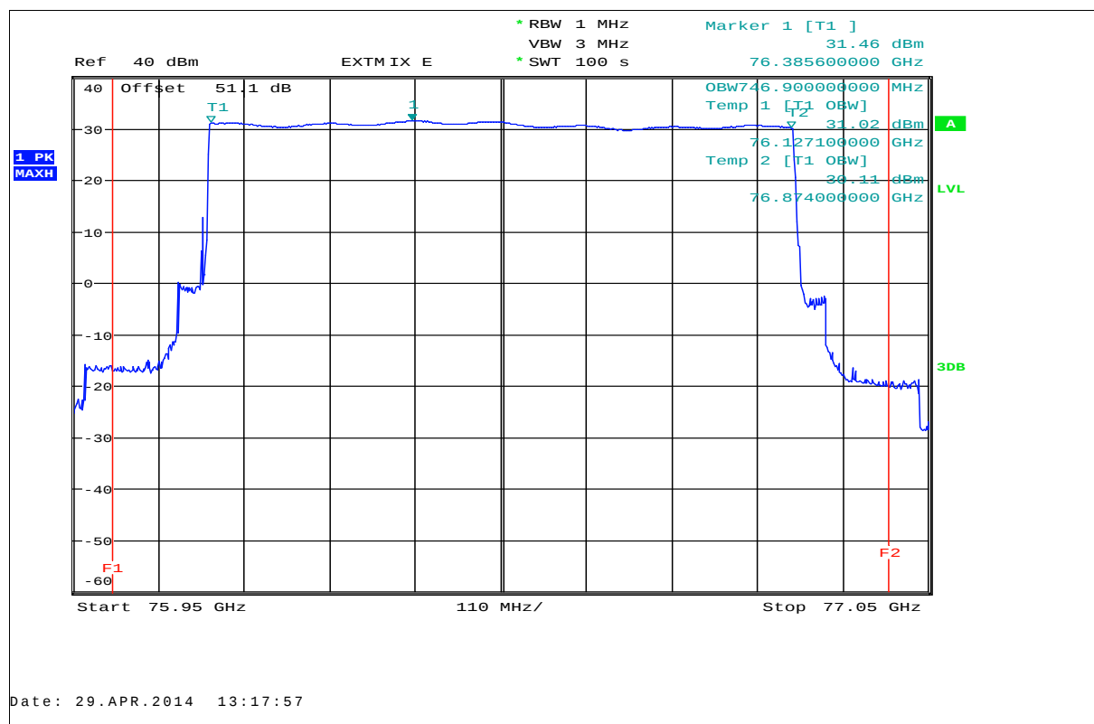
Plot 7: Occupied bandwidth (99%), T_{\text{nom}} / V_{\text{nom}}
