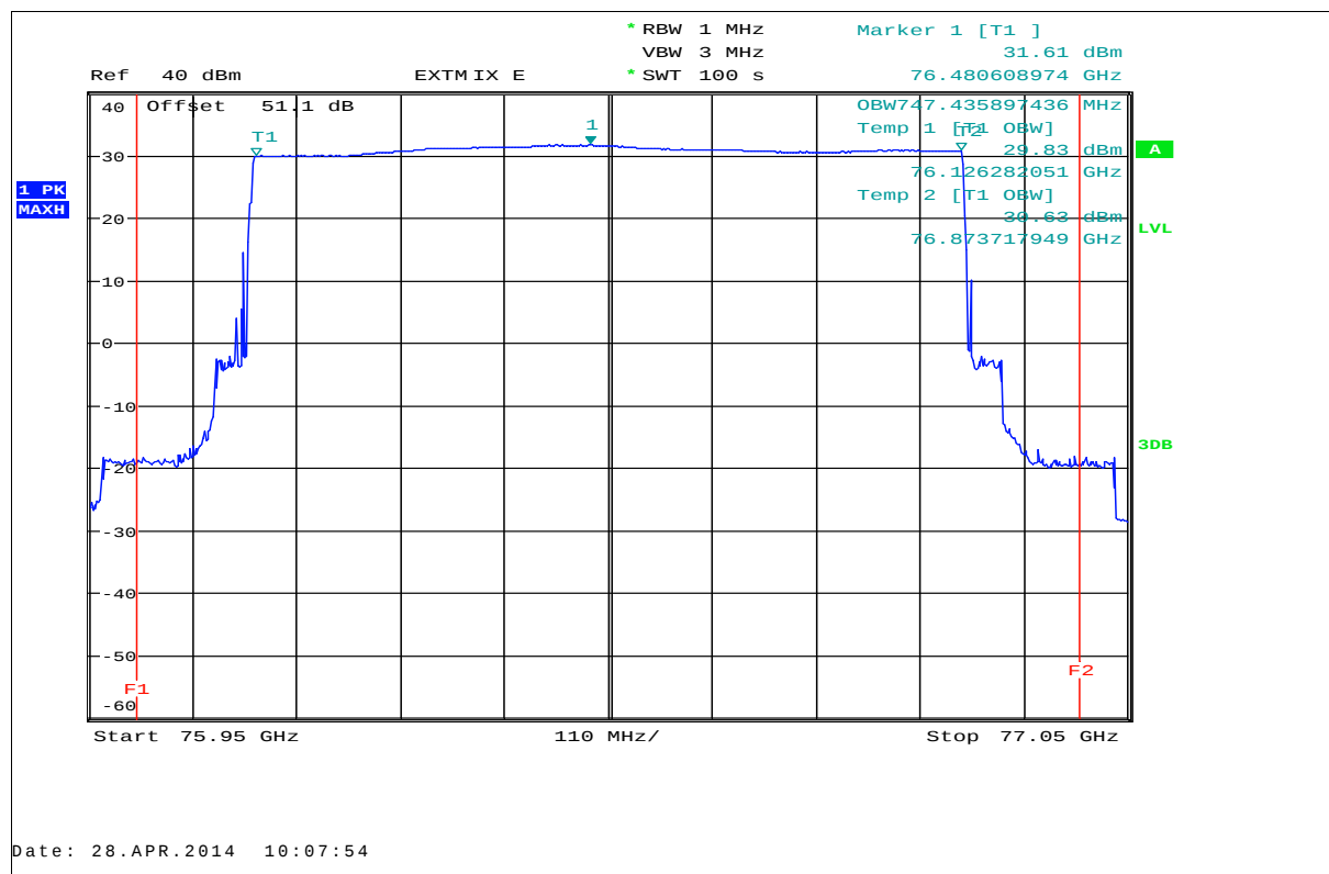
Plot 8: Occupied bandwidth (99%), T_{\text{min}} / V_{\text{min}} - V_{\text{max}}
