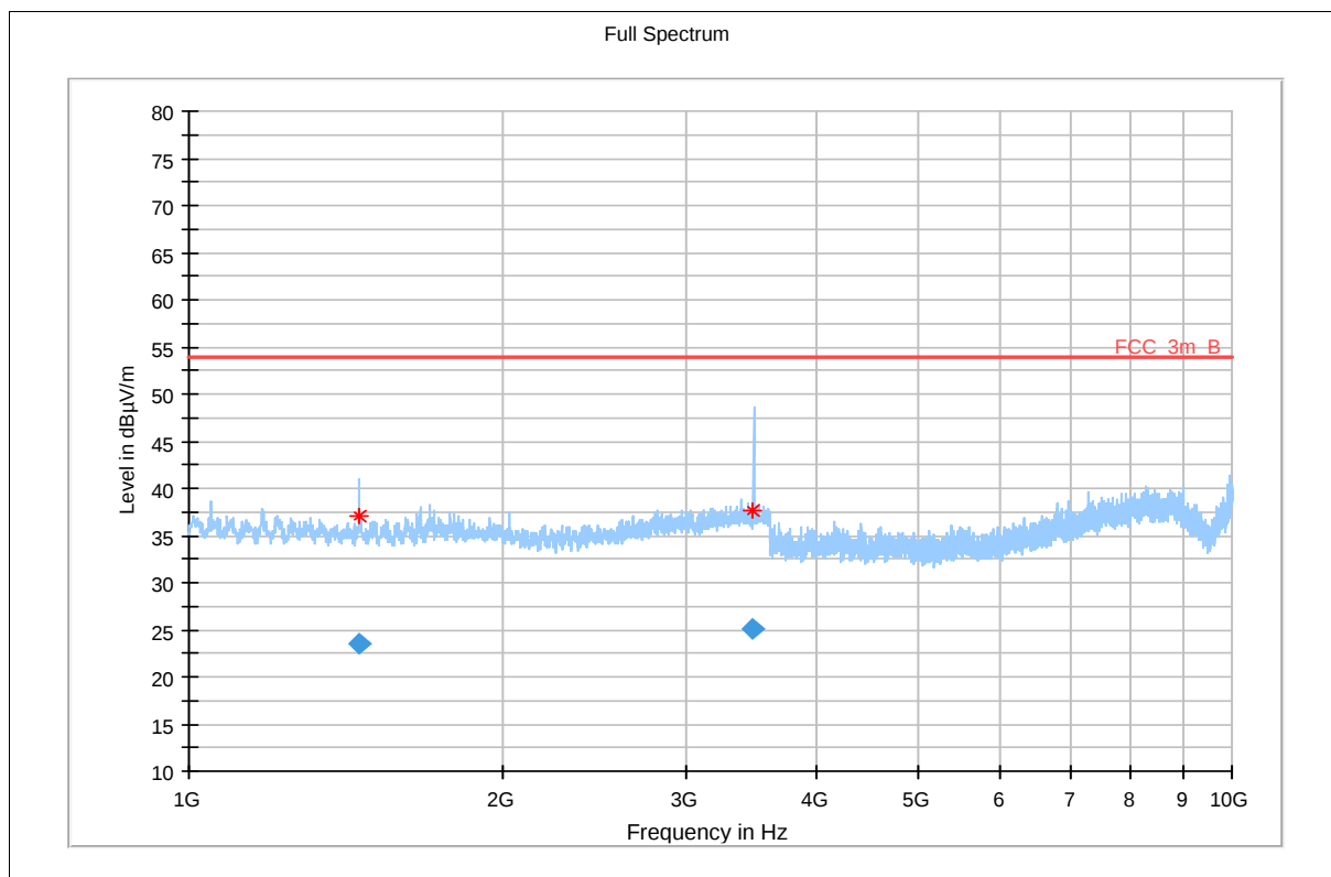
Plot 15: 1 GHz – 10 GHz, antenna horizontal and vertical, middle frequency
