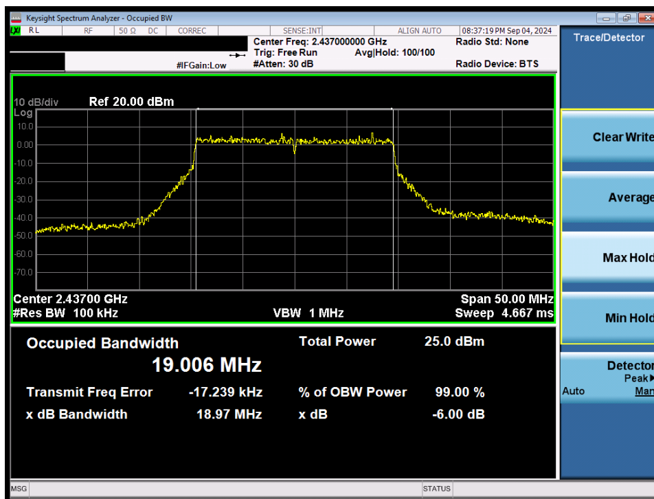
Plot 7-26. 6dB Bandwidth Plot (802.11ax/be (2.4GHz) – Ch. 6) MIMO ANT2
