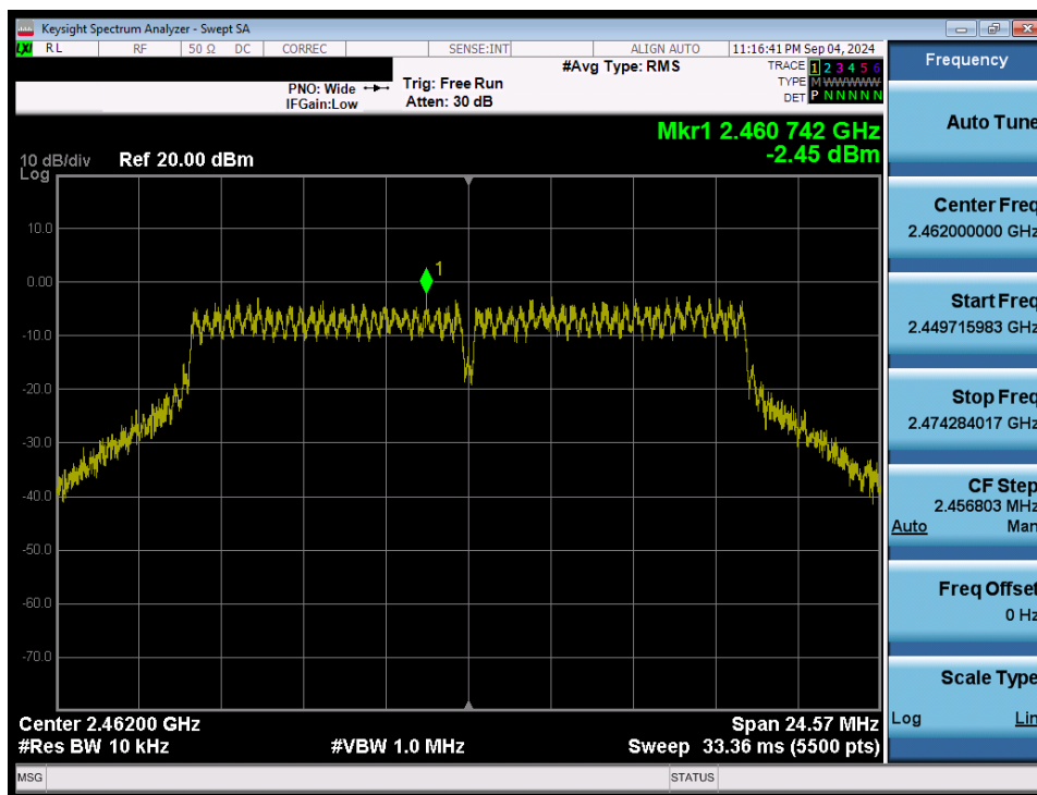
Plot 7-45. Power Spectral Density Plot (802.11g – Ch. 11) MIMO ANT2
