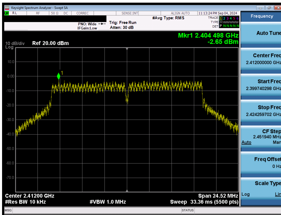
Plot 7-43. Power Spectral Density Plot (802.11g – Ch. 1) MIMO ANT2
