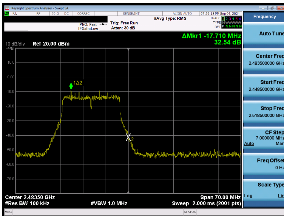
Plot 7-63. Band Edge Plot (802.11n/ac (2.4GHz) – Ch. 13) MIMO ANT1
