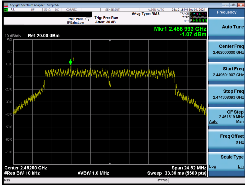
Plot 7-33. Power Spectral Density Plot (802.11g – Ch. 11) MIMO ANT1
