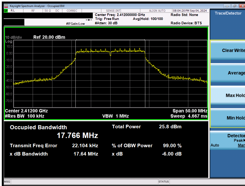
Plot 7-10. 6dB Bandwidth Plot (802.11n/ac (2.4GHz) – Ch. 1) MIMO ANT1
