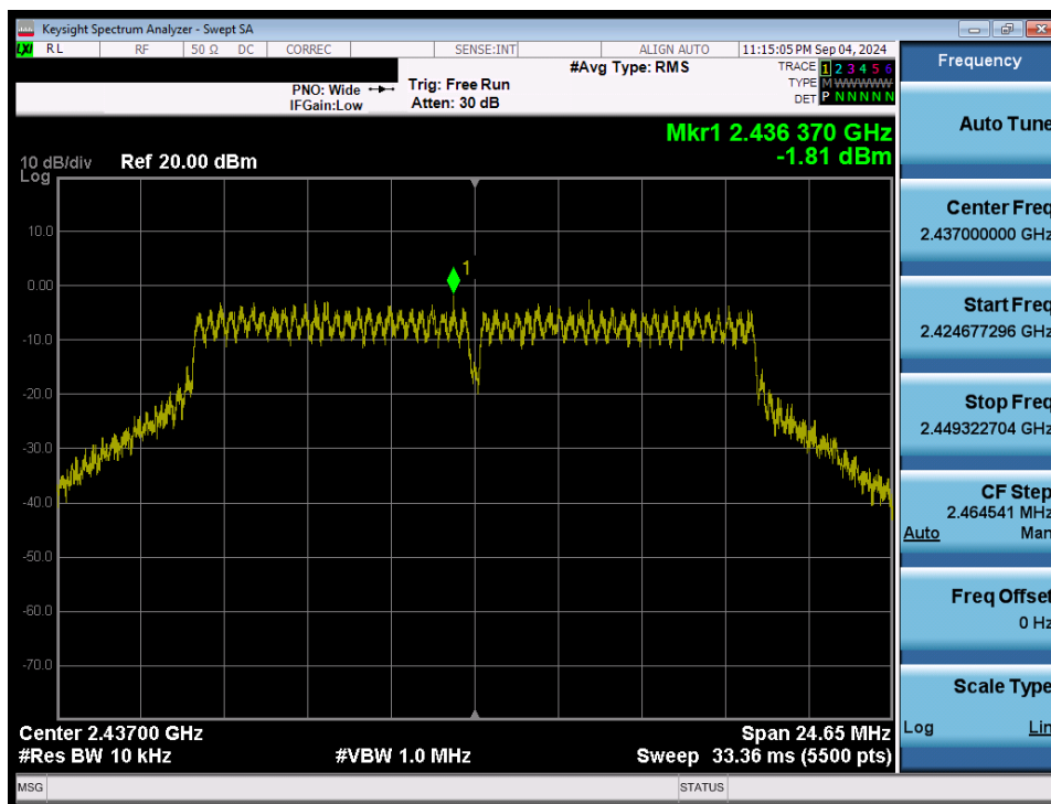
Plot 7-44. Power Spectral Density Plot (802.11g – Ch. 6) MIMO ANT2
