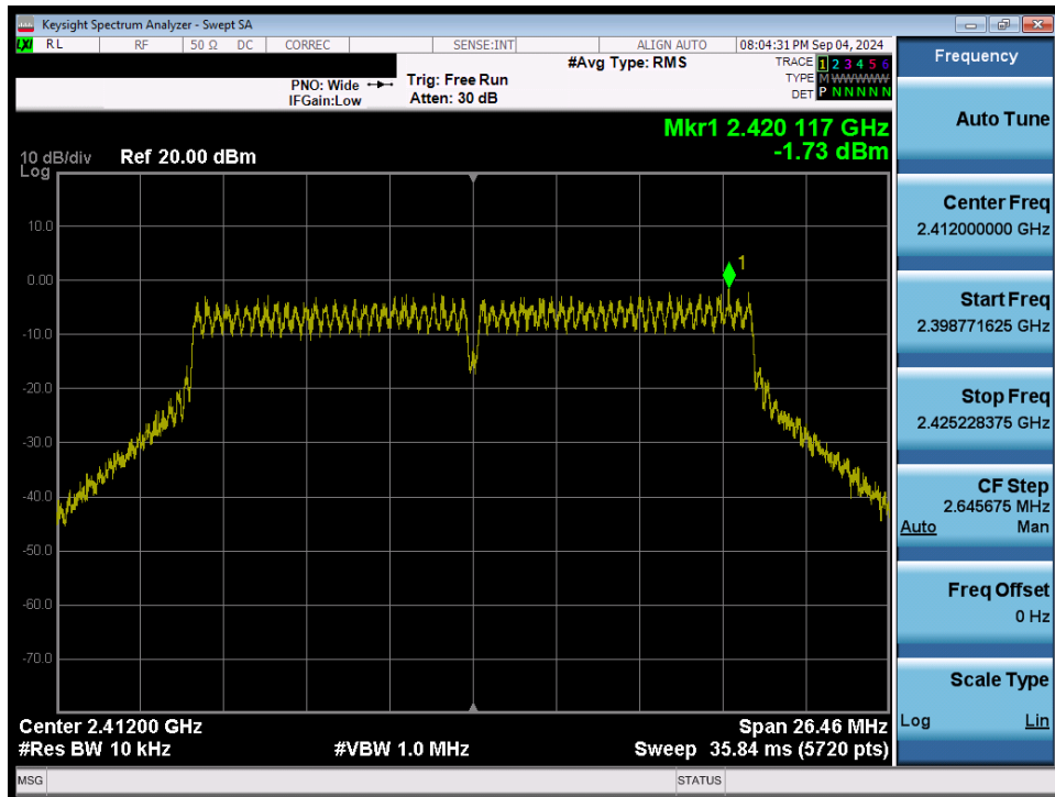
Plot 7-34. Power Spectral Density Plot (802.11n/ac (2.4GHz) – Ch. 1) MIMO ANT1
