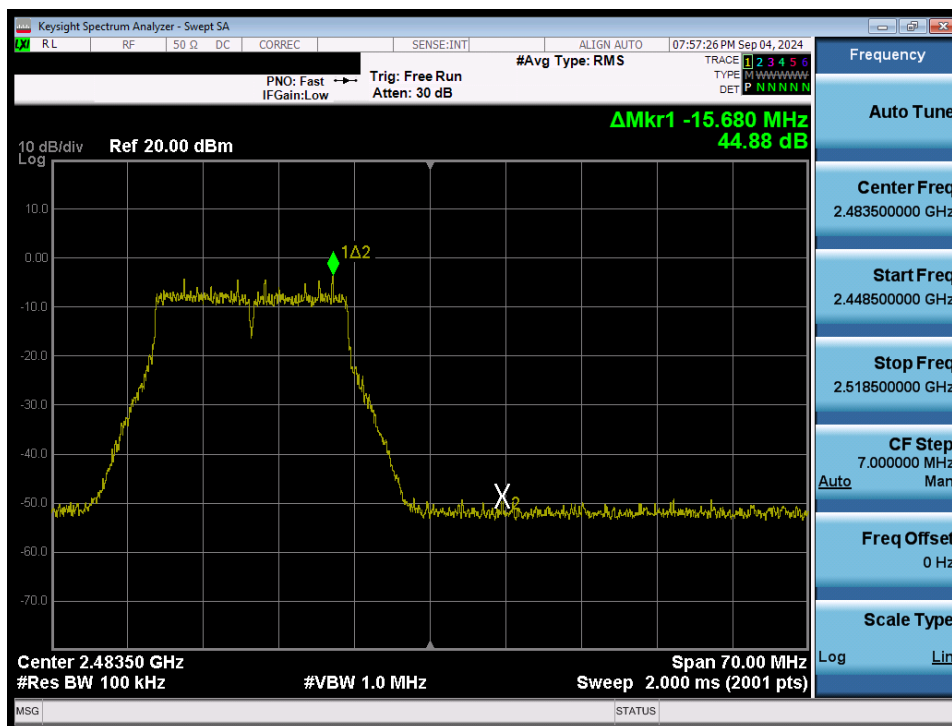
Plot 7-62. Band Edge Plot (802.11n/ac (2.4GHz) – Ch. 12) MIMO ANT1
