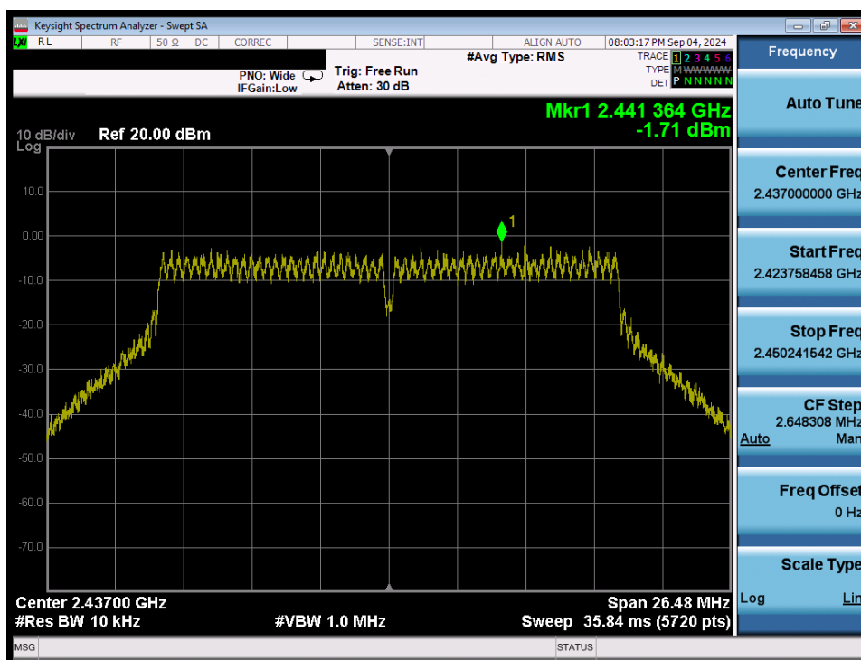
Plot 7-35. Power Spectral Density Plot (802.11n/ac (2.4GHz) – Ch. 6) MIMO ANT1
