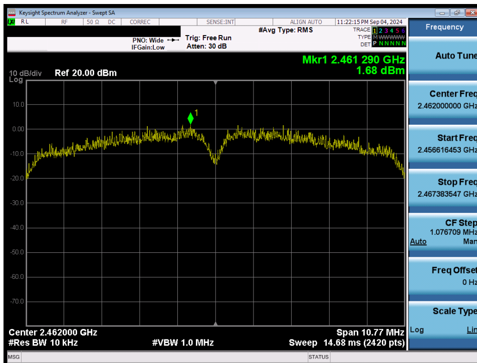
Plot 7-42. Power Spectral Density Plot (802.11b – Ch. 11) SISO ANT2
