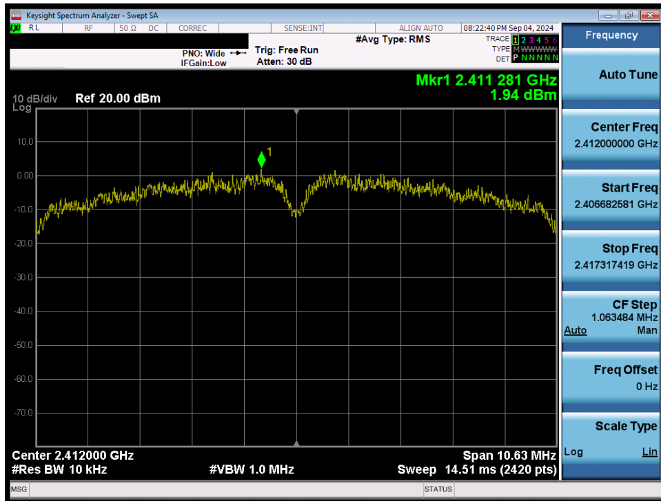
Plot 7-28. Power Spectral Density Plot (802.11b – Ch. 1) SISO ANT1
