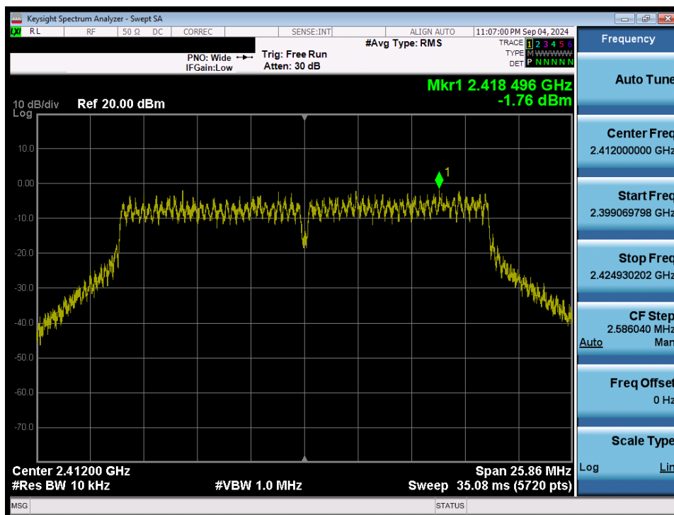
Plot 7-46. Power Spectral Density Plot (802.11n/ac (2.4GHz) – Ch. 1) MIMO ANT2
