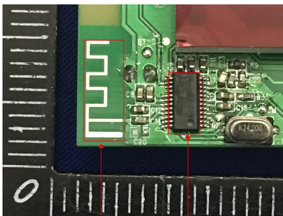
BT Antenna
