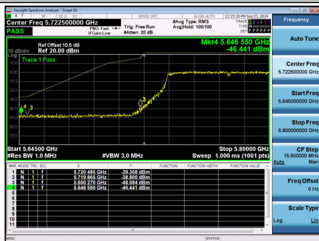
11AC80MIMO-Ant2-5775-PASS
