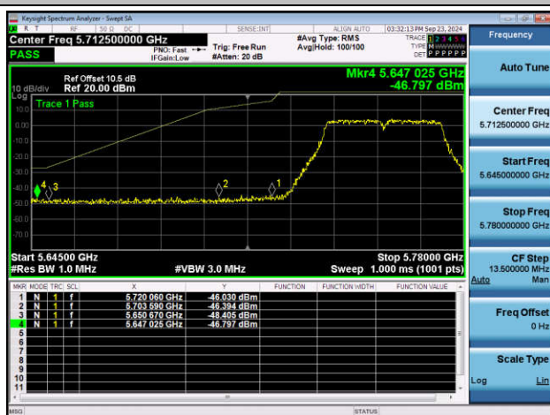
11AC40MIMO-Ant2-5755-PASS
