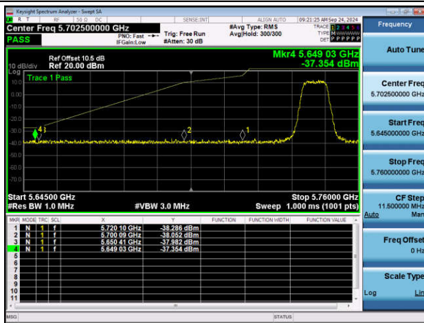
11A(10MHZ)-Ant1-5745-PASS
