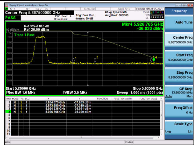
11A(10MHZ)-Ant1-5825-PASS
