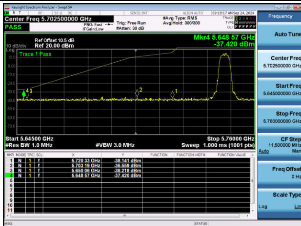
11A(5MHZ)-Ant2-5745.5-PASS
