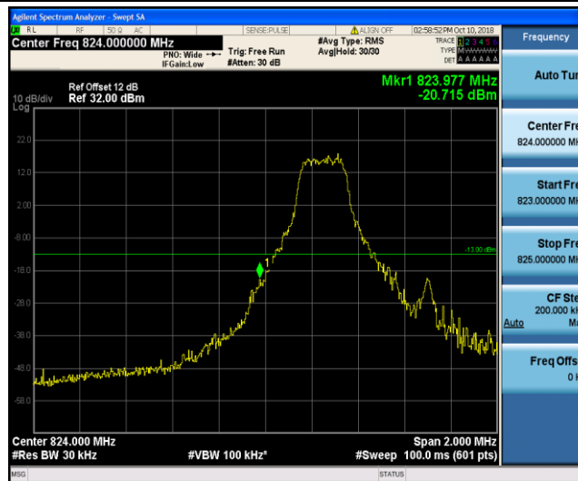
Band26_1.4MHz_16QAM_20407_1RB#0
