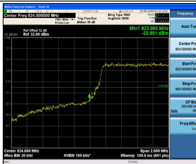
Band26_1.4MHz_16QAM_20407_6RB#0
