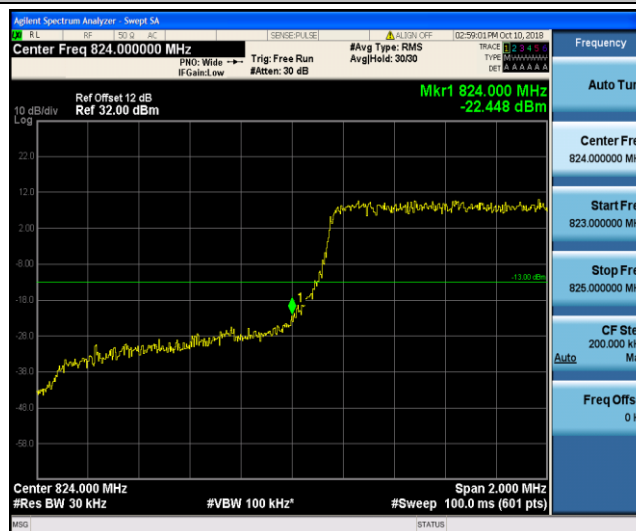
Band26_1.4MHz_QPSK_20407_6RB#0
