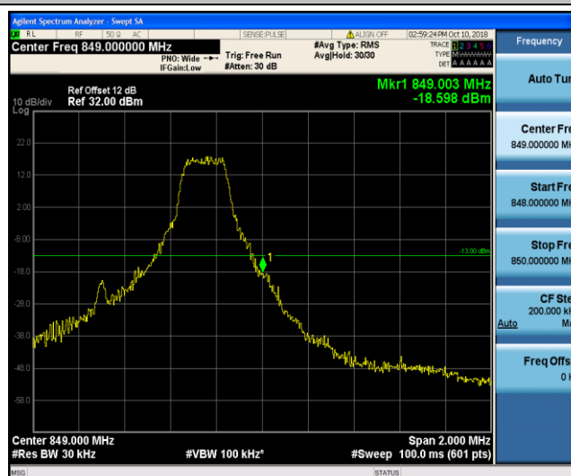
Band26_1.4MHz_QPSK_20643_1RB#5
