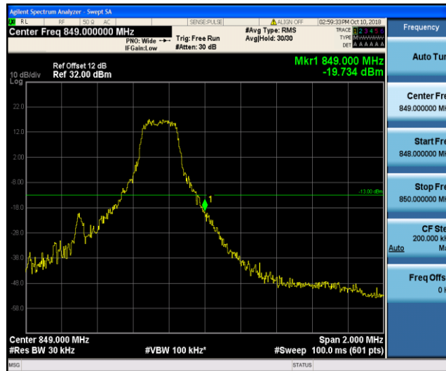
Band26_1.4MHz_16QAM_20643_1RB#5
