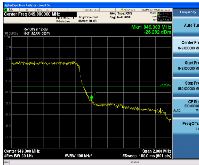
Band26_1.4MHz_QPSK_20643_6RB#0
