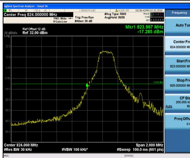
Band26_1.4MHz_QPSK_20407_1RB#0
