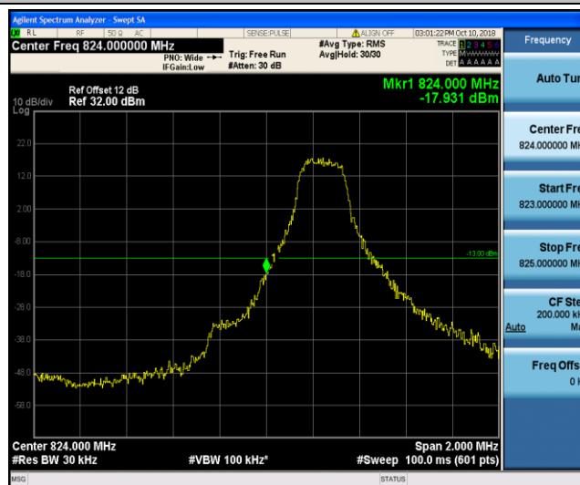
Band26_3MHz_QPSK_20415_1RB#0
