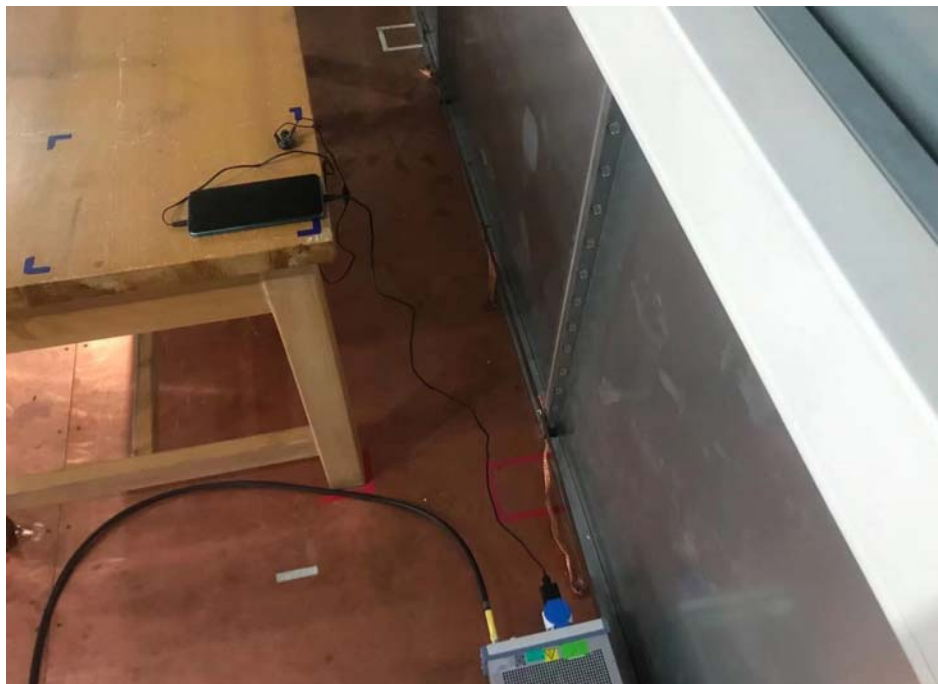
Conducted Emissions Test Setup (with charger)
