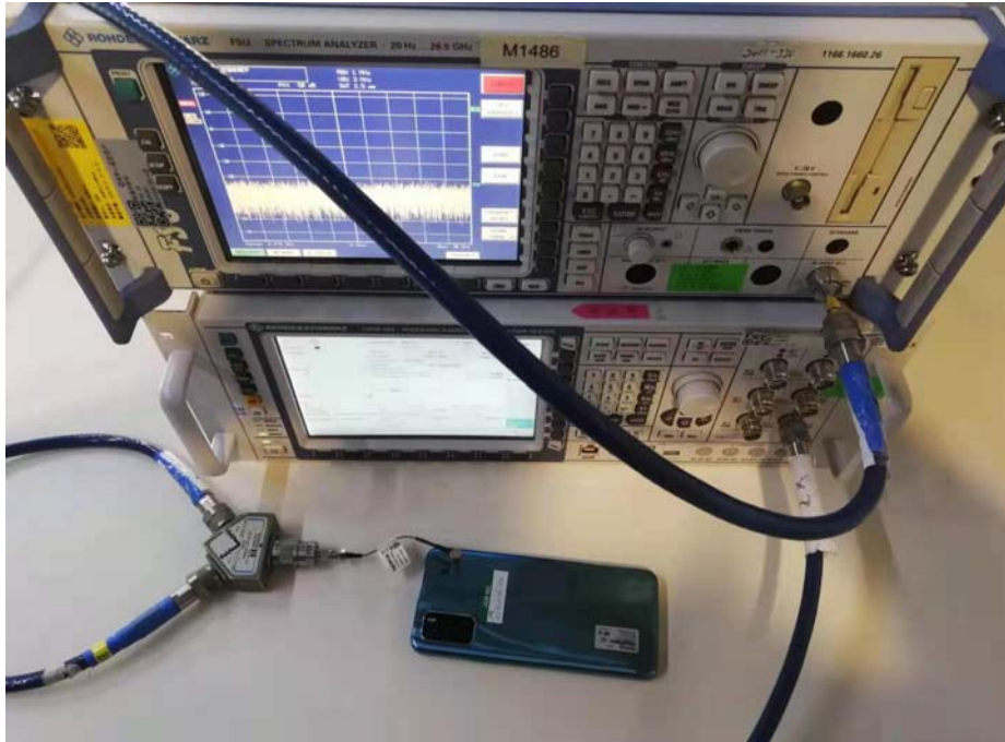
RF Conducted Test setup (GSM/WCDMA/LTE)
