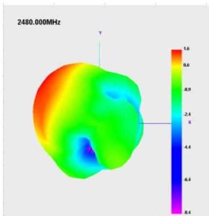
2.4G H plane
