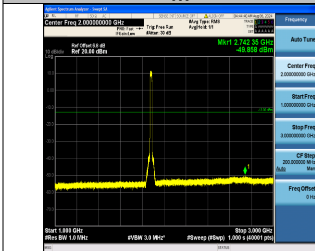
Band2_20MHz_QPSK_18900_100RB#0_1000~3000_1000~3000
