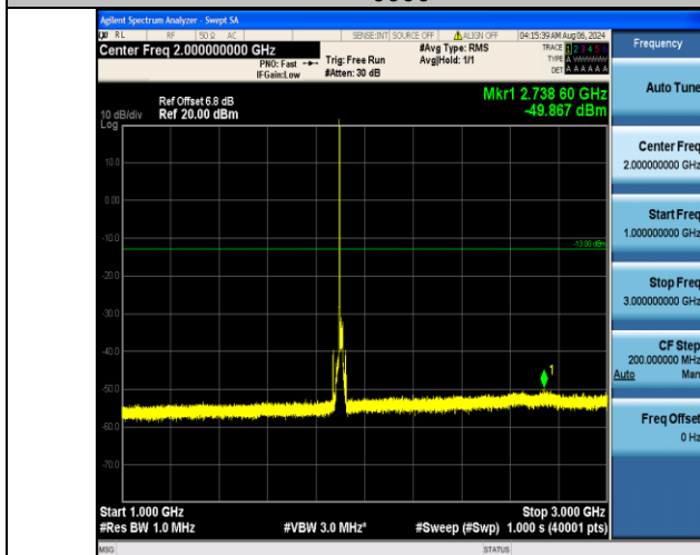
Band2_15MHz_16QAM_19125_1RB#0_1000~3000_1000~3000
