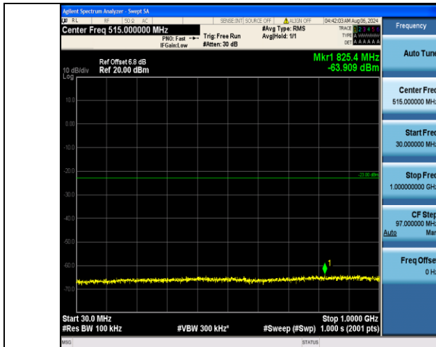
Band2_20MHz_16QAM_18700_1RB#99_30~1000_30~1000
