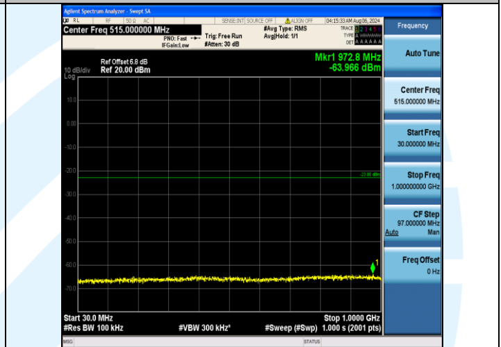
Band2_15MHz_16QAM_19125_1RB#0_30~1000_30~1000
