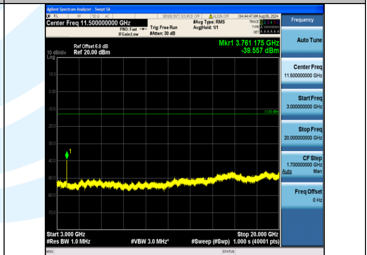
Band2_20MHz_QPSK_18900_100RB#0_3000~20000_3000~20000
