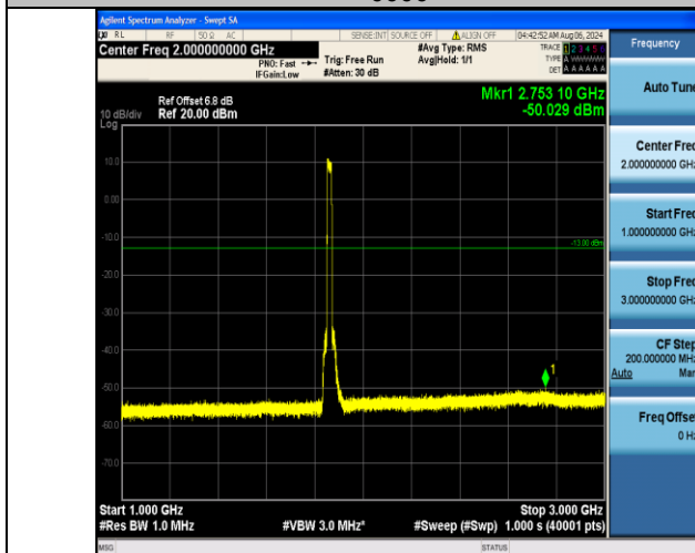
Band2_20MHz_16QAM_18700_100RB#0_1000~3000_1000~3000
