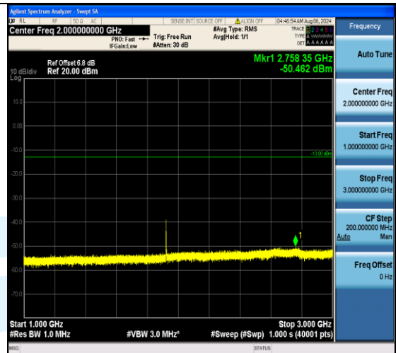
Band2_20MHz_QPSK_19100_100RB#0_1000~3000_1000~3000
