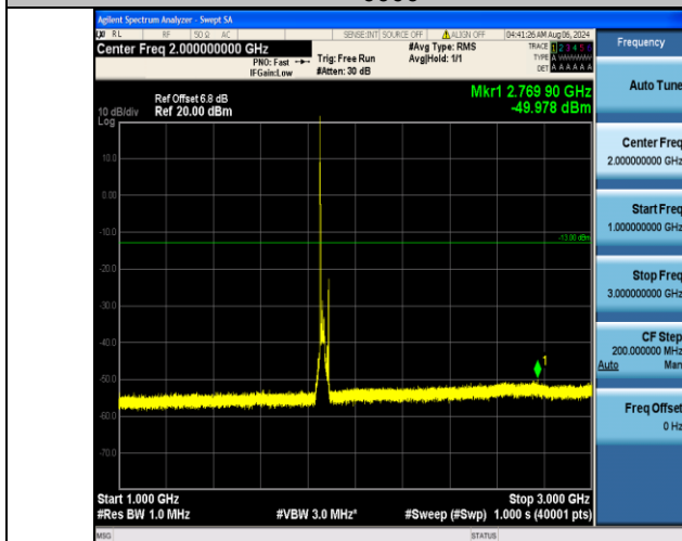
Band2_20MHz_16QAM_18700_1RB#0_1000~3000_1000~3000
