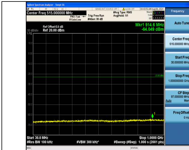
Band2_20MHz_QPSK_18900_1RB#99_30~1000_30~1000
