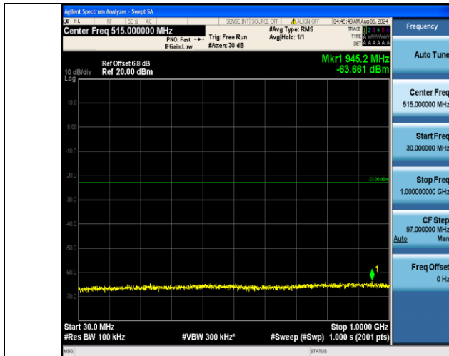
Band2_20MHz_QPSK_19100_100RB#0_30~1000_30~1000
