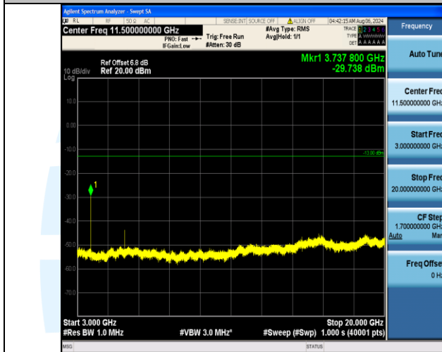
Band2_20MHz_16QAM_18700_1RB#99_3000~20000_3000~20000
