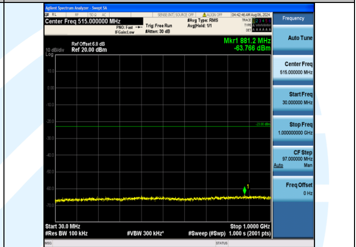
Band2_20MHz_16QAM_18700_100RB#0_30~1000_30~1000
