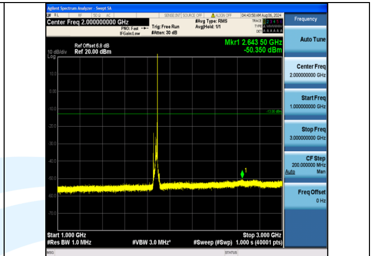
Band2_20MHz_QPSK_18900_1RB#99_1000~3000_1000~3000
