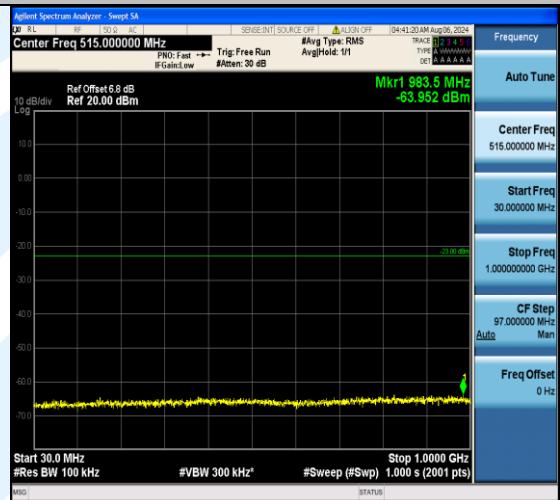
Band2_20MHz_16QAM_18700_1RB#0_30~1000_30~1000
