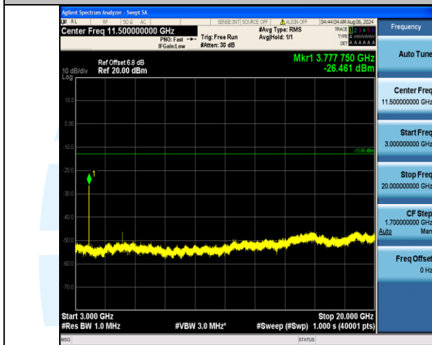
Band2_20MHz_QPSK_18900_1RB#99_3000~20000_3000~20000
