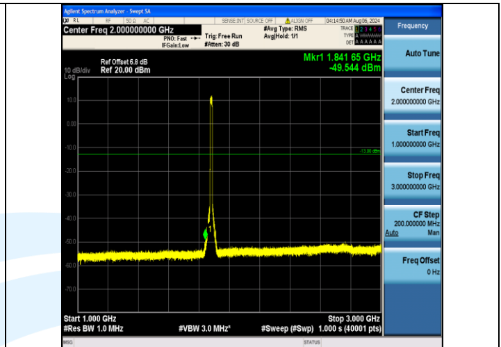
Band2_15MHz_16QAM_18900_75RB#0_1000~3000_1000~3000
