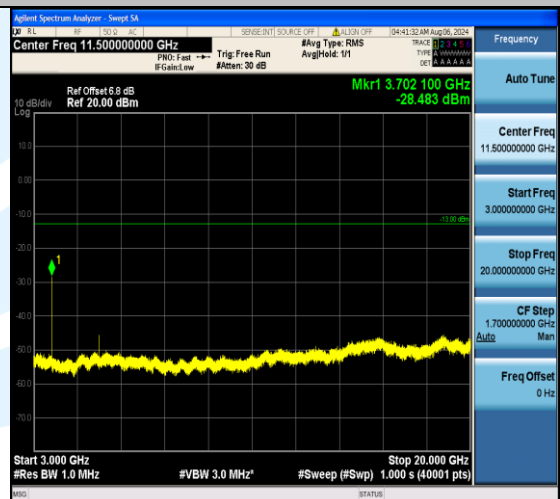
Band2_20MHz_16QAM_18700_1RB#0_3000~20000_3000~20000
