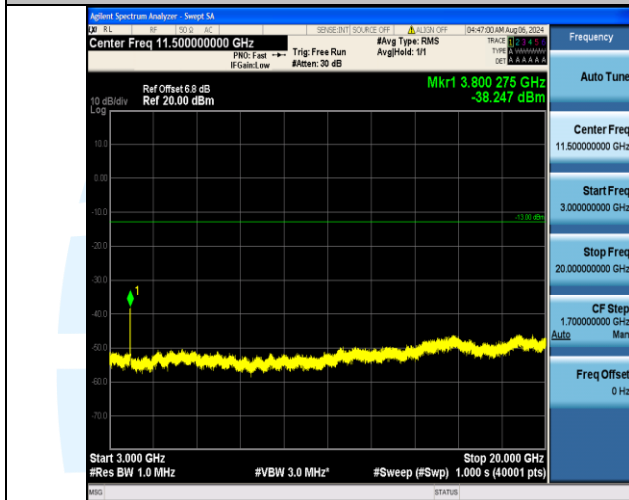
Band2_20MHz_QPSK_19100_100RB#0_3000~20000_3000~20000
