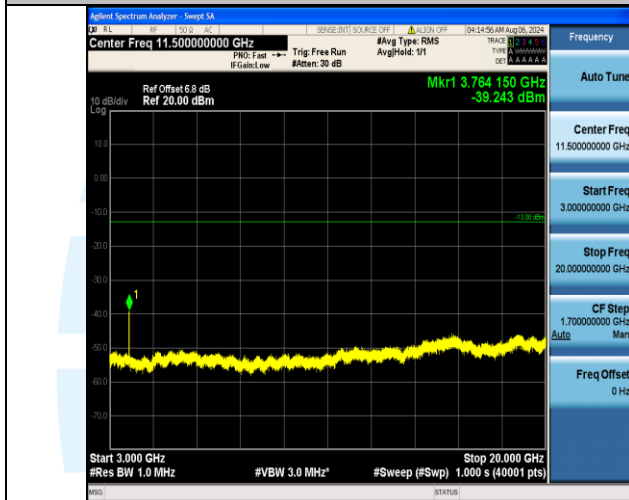
Band2_15MHz_16QAM_18900_75RB#0_3000~20000_3000~20000
