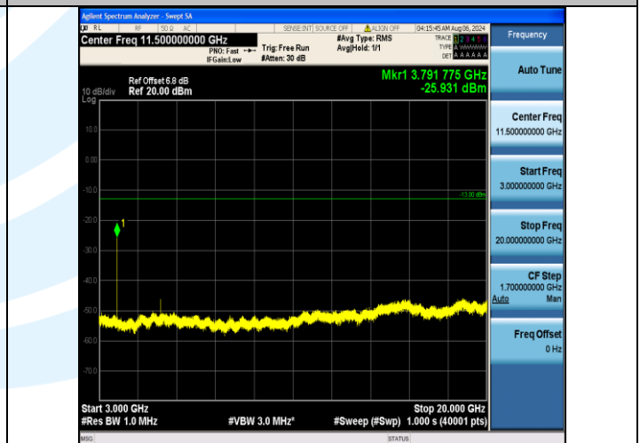
Band2_15MHz_16QAM_19125_1RB#0_3000~20000_3000~20000
