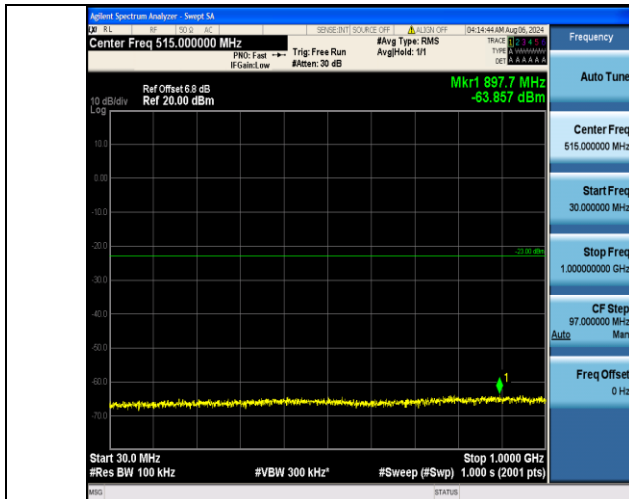
Band2_15MHz_16QAM_18900_75RB#0_30~1000_30~1000
