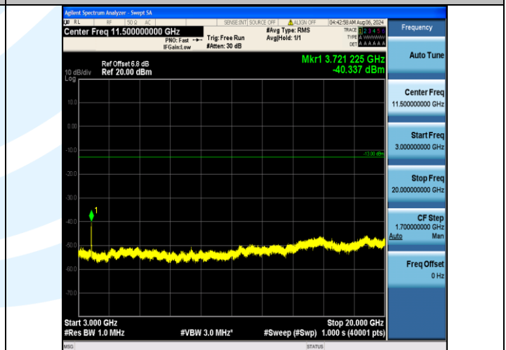
Band2_20MHz_16QAM_18700_100RB#0_3000~20000_3000~20000
