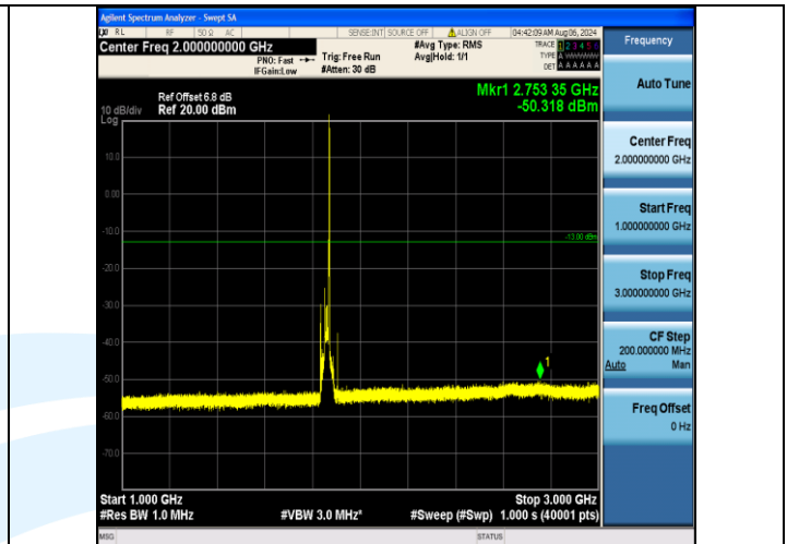
Band2_20MHz_16QAM_18700_1RB#99_1000~3000_1000~3000
