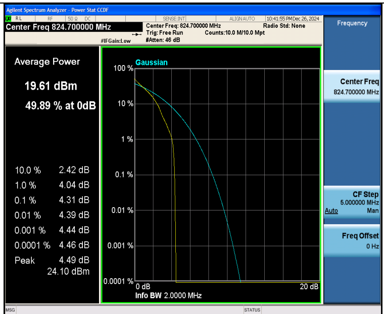
Band26(824-849)-1.4MHz-QPSK-26797-1RB#0-PASS
