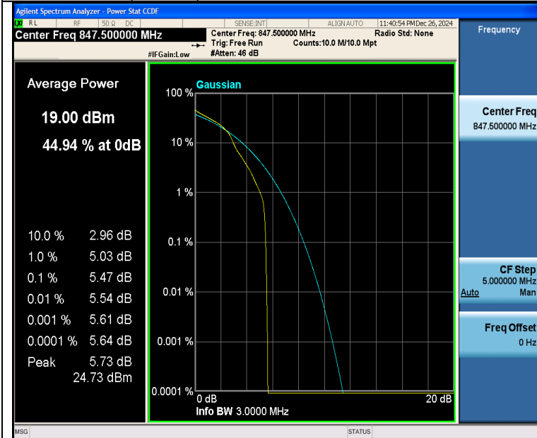
Band26(824-849)-3MHz-16QAM-27025-1RB#0-PASS
