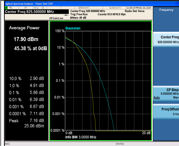
Band26(824-849)-3MHz-16QAM-26805-15RB#0-PASS
