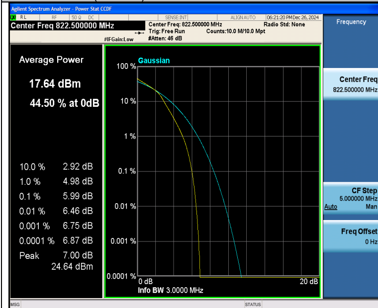
Band26(814-824)-3MHz-16QAM-26775-15RB#0-PASS
