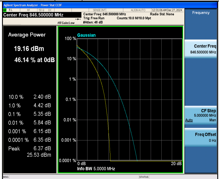
Band26(824-849)-5MHz-QPSK-27015-25RB#0-PASS
