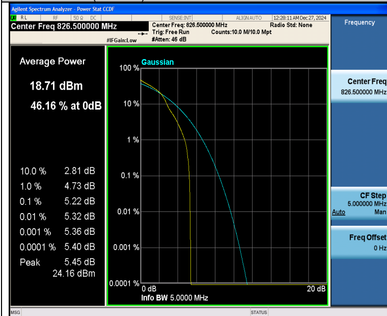
Band26(824-849)-5MHz-16QAM-26815-1RB#0-PASS
