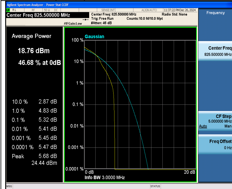
Band26(824-849)-3MHz-16QAM-26805-1RB#0-PASS
