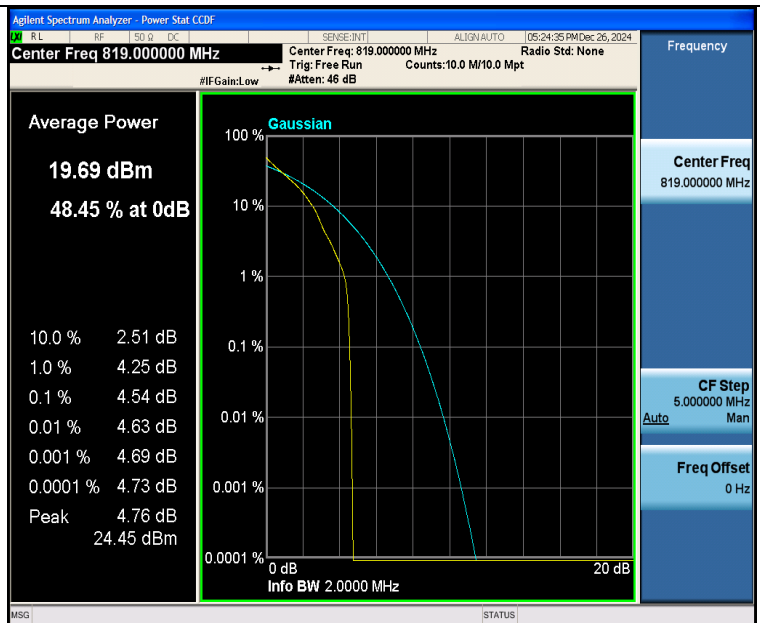
Band26(814-824)-1.4MHz-QPSK-26740-1RB#0-PASS
