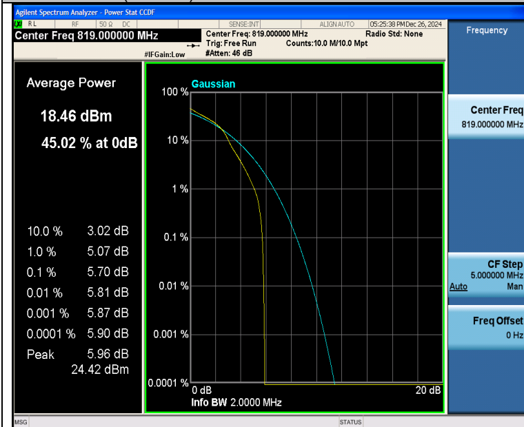
Band26(814-824)-1.4MHz-16QAM-26740-1RB#0-PASS
