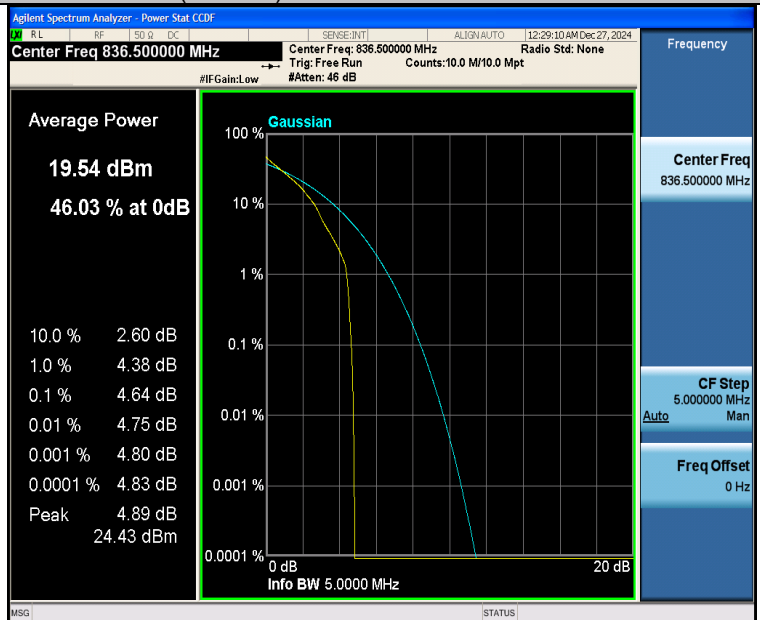
Band26(824-849)-5MHz-QPSK-26915-1RB#0-PASS
