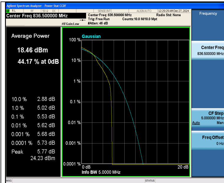
Band26(824-849)-5MHz-16QAM-26915-1RB#0-PASS
