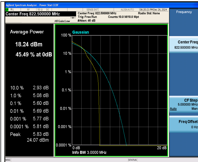
Band26(814-824)-3MHz-16QAM-26775-1RB#0-PASS
