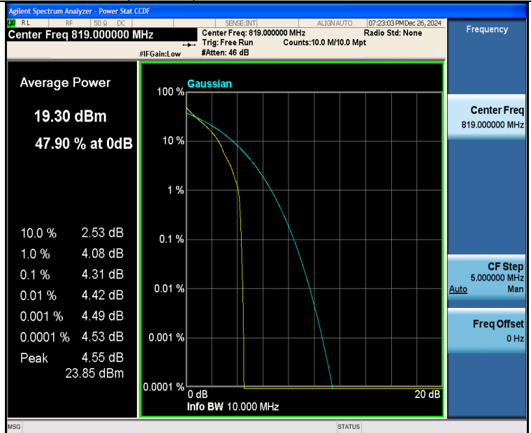
Band26(814-824)-10MHz-QPSK-26740-1RB#0-PASS
