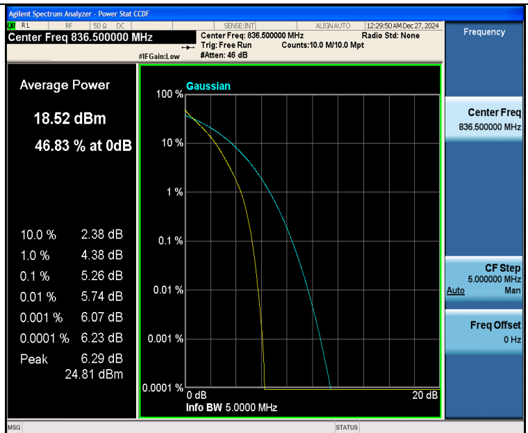
Band26(824-849)-5MHz-QPSK-26915-25RB#0-PASS
