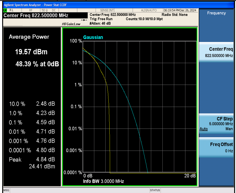
Band26(814-824)-3MHz-QPSK-26775-1RB#0-PASS
