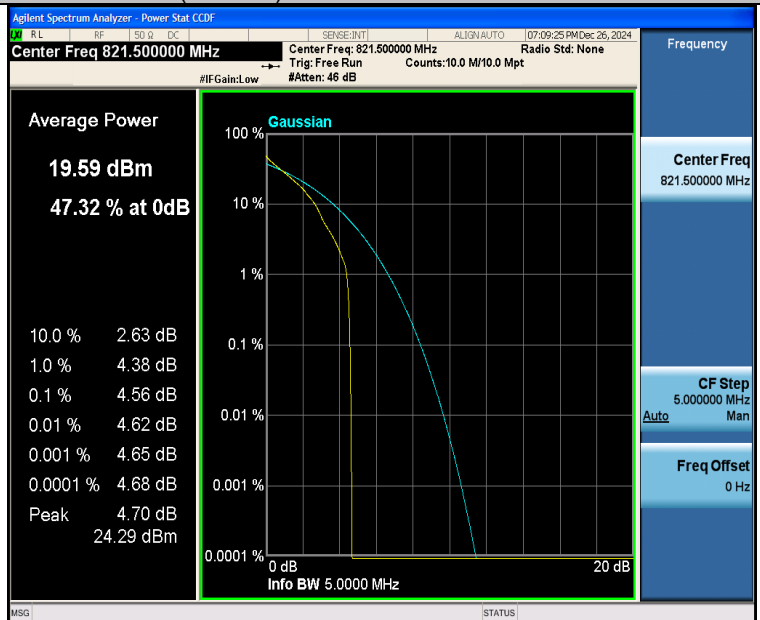
Band26(814-824)-5MHz-QPSK-26765-1RB#0-PASS
