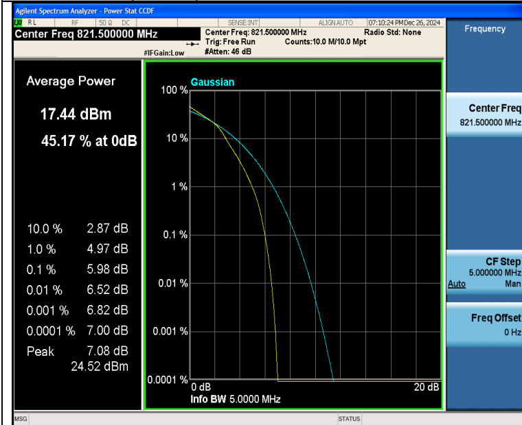
Band26(814-824)-5MHz-16QAM-26765-25RB#0-PASS
