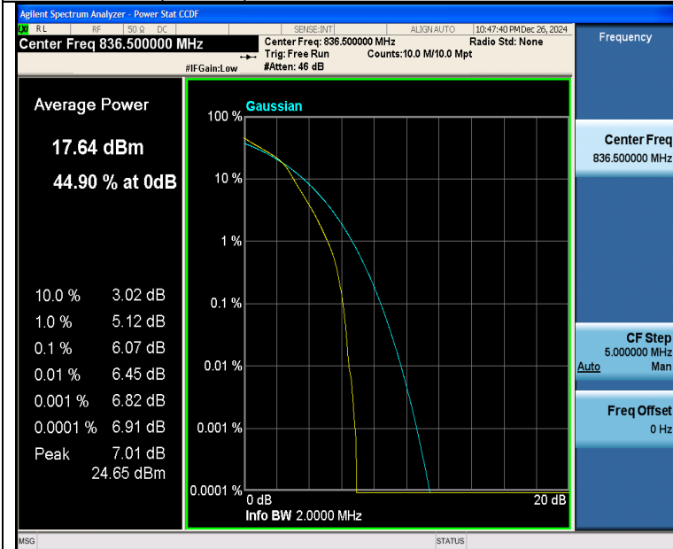
Band26(824-849)-1.4MHz-16QAM-26915-6RB#0-PASS
