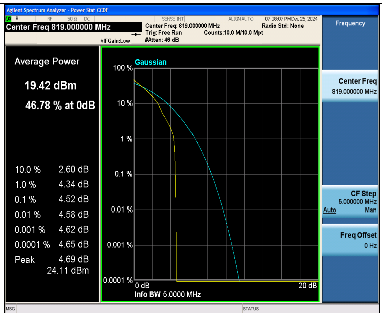
Band26(814-824)-5MHz-QPSK-26740-1RB#0-PASS
