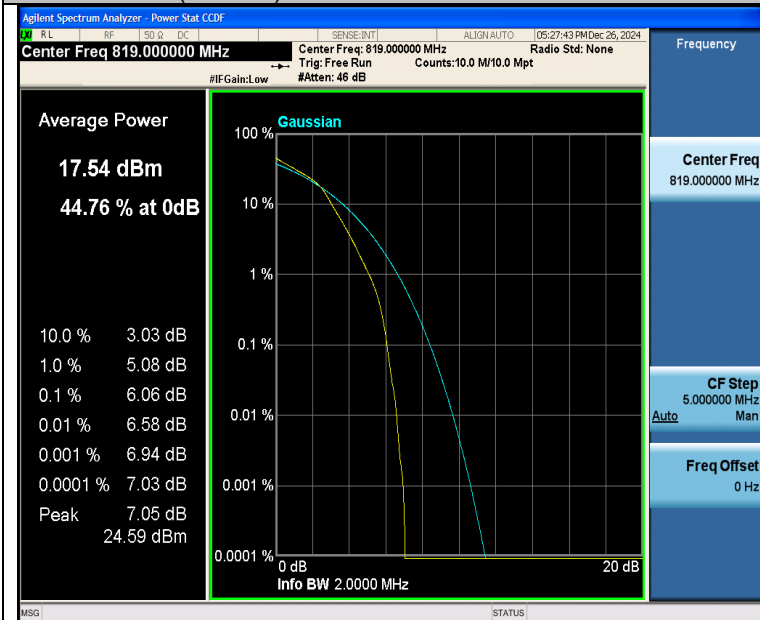
Band26(814-824)-1.4MHz-16QAM-26740-6RB#0-PASS
