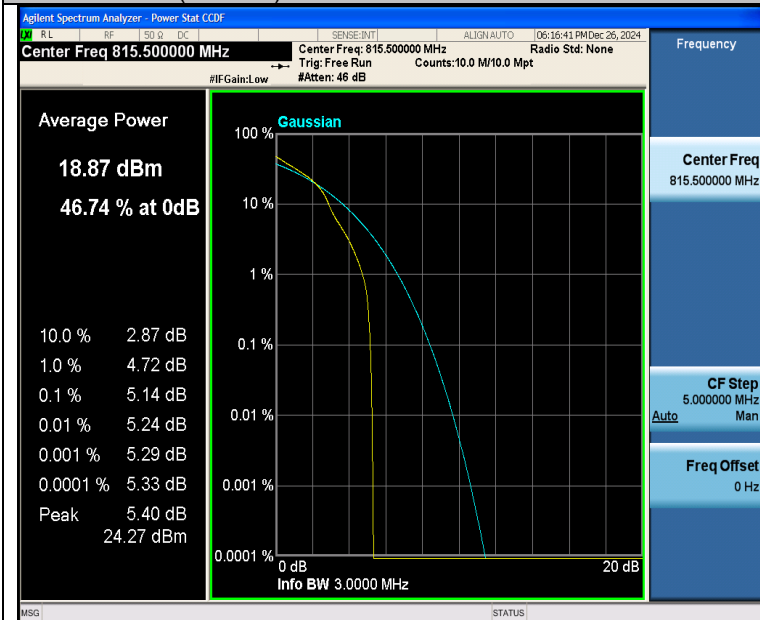
Band26(814-824)-3MHz-16QAM-26705-1RB#0-PASS
