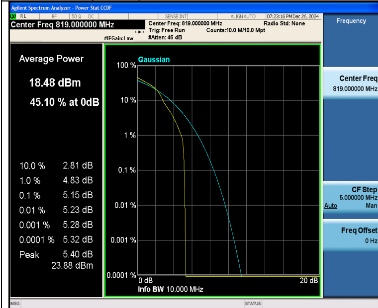
Band26(814-824)-10MHz-16QAM-26740-1RB#0-PASS
