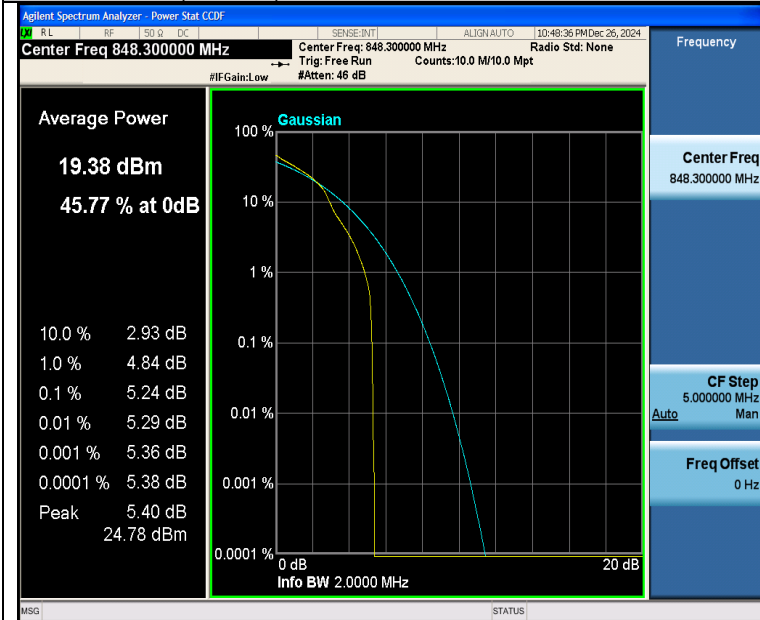
Band26(824-849)-1.4MHz-16QAM-27033-1RB#0-PASS
