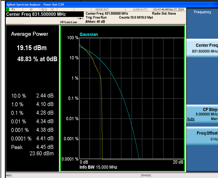
Band26(824-849)-15MHz-QPSK-26865-1RB#0-PASS
