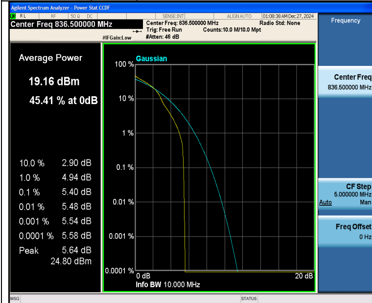
Band26(824-849)-10MHz-16QAM-26915-1RB#0-PASS
