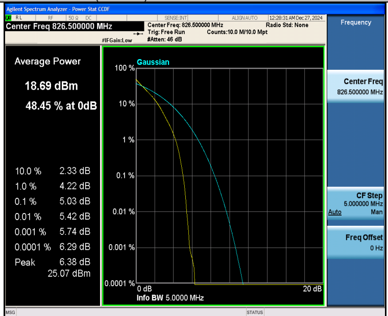
Band26(824-849)-5MHz-QPSK-26815-25RB#0-PASS
