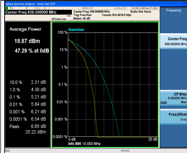
Band26(824-849)-10MHz-QPSK-26915-50RB#0-PASS
