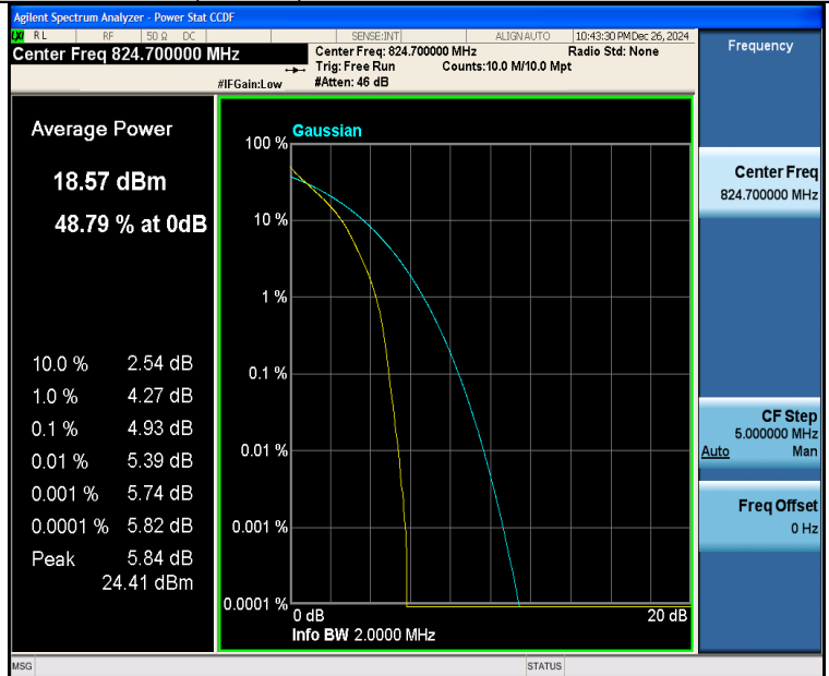
Band26(824-849)-1.4MHz-QPSK-26797-6RB#0-PASS
