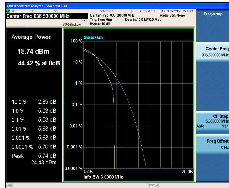
Band26(824-849)-3MHz-16QAM-26915-1RB#0-PASS
