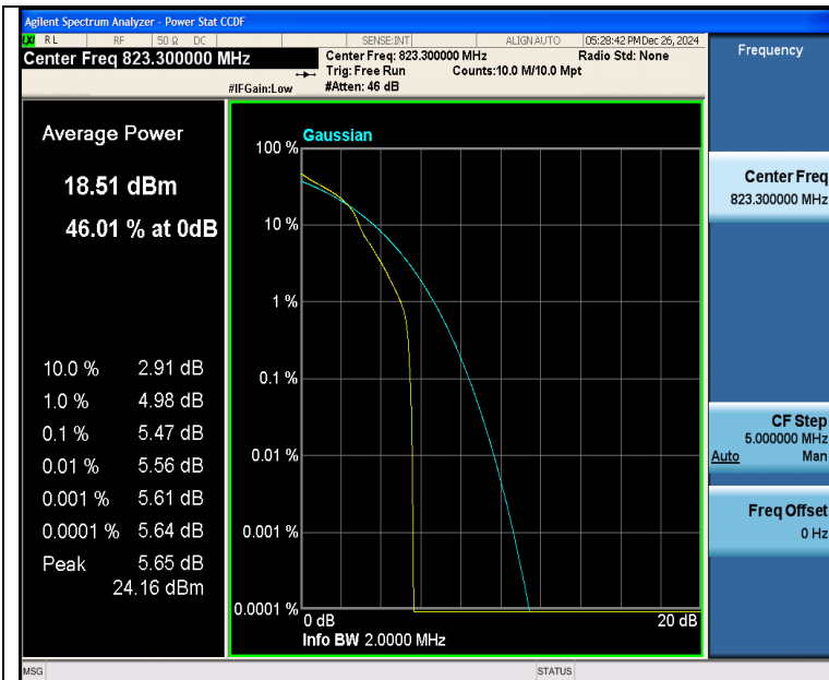
Band26(814-824)-1.4MHz-16QAM-26783-1RB#0-PASS
