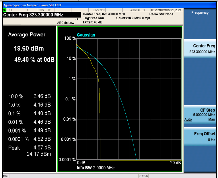
Band26(814-824)-1.4MHz-QPSK-26783-1RB#0-PASS
