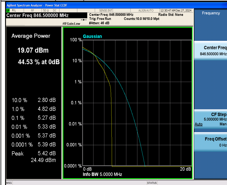
Band26(824-849)-5MHz-16QAM-27015-1RB#0-PASS
