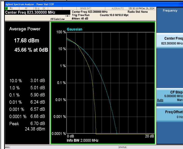
Band26(814-824)-1.4MHz-16QAM-26783-6RB#0-PASS
