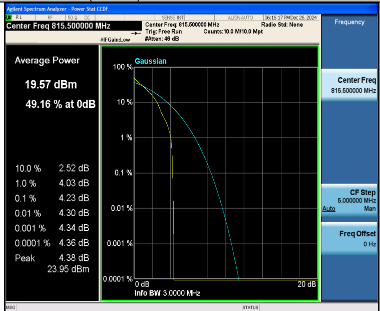
Band26(814-824)-3MHz-QPSK-26705-1RB#0-PASS
