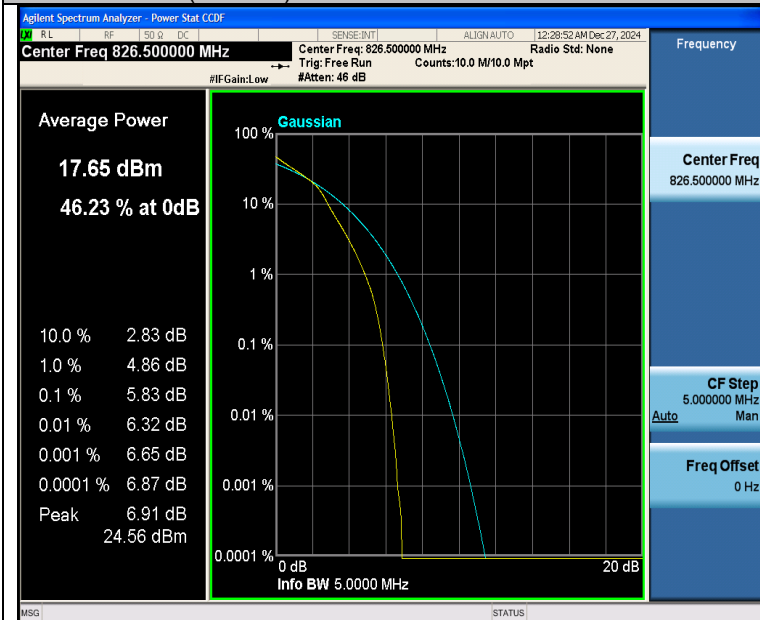
Band26(824-849)-5MHz-16QAM-26815-25RB#0-PASS
