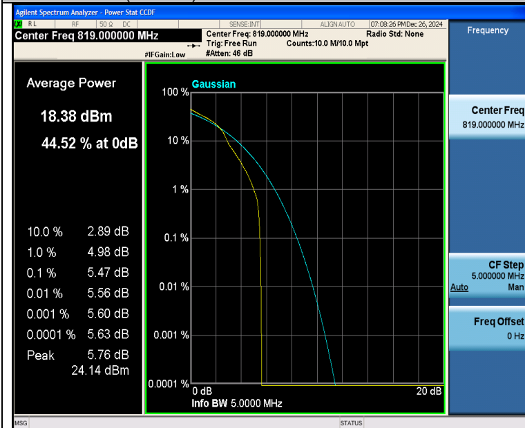
Band26(814-824)-5MHz-16QAM-26740-1RB#0-PASS
