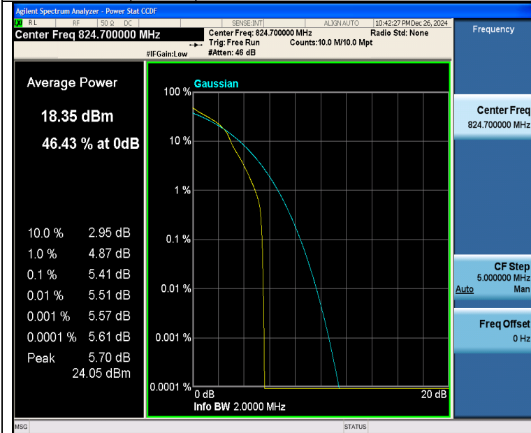
Band26(824-849)-1.4MHz-16QAM-26797-1RB#0-PASS
