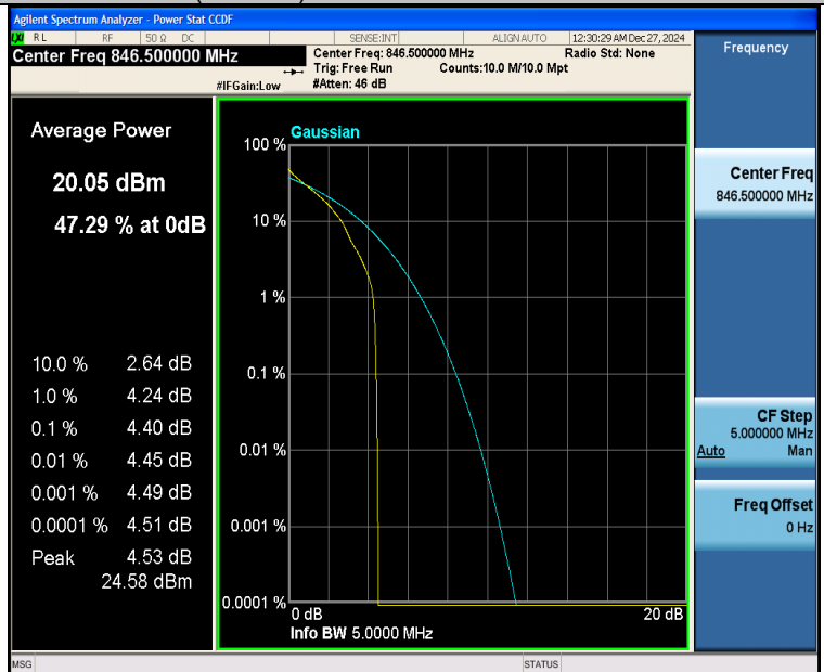
Band26(824-849)-5MHz-QPSK-27015-1RB#0-PASS
