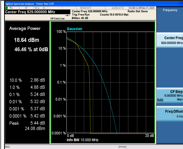
Band26(824-849)-10MHz-16QAM-26840-1RB#0-PASS
