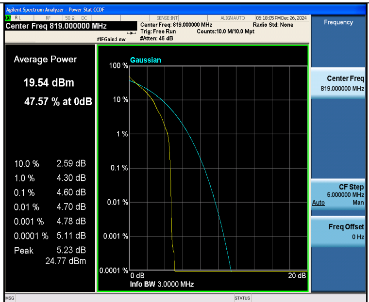
Band26(814-824)-3MHz-QPSK-26740-1RB#0-PASS
