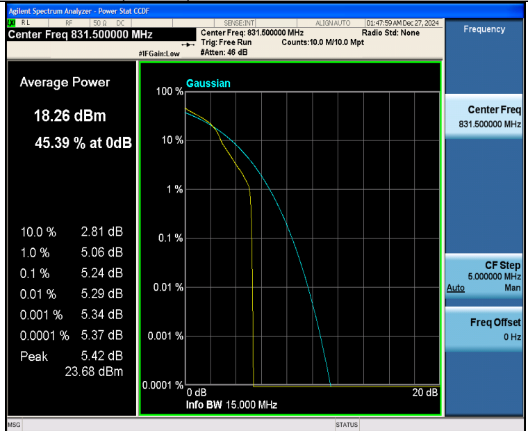
Band26(824-849)-15MHz-16QAM-26865-1RB#0-PASS
