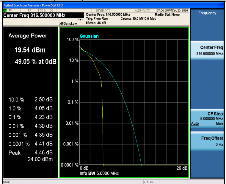
Band26(814-824)-5MHz-QPSK-26715-1RB#0-PASS
