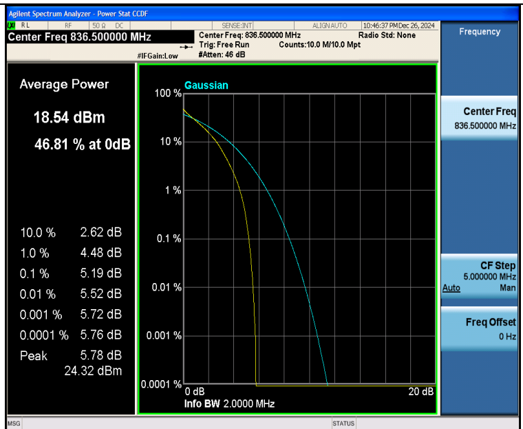
Band26(824-849)-1.4MHz-QPSK-26915-6RB#0-PASS
