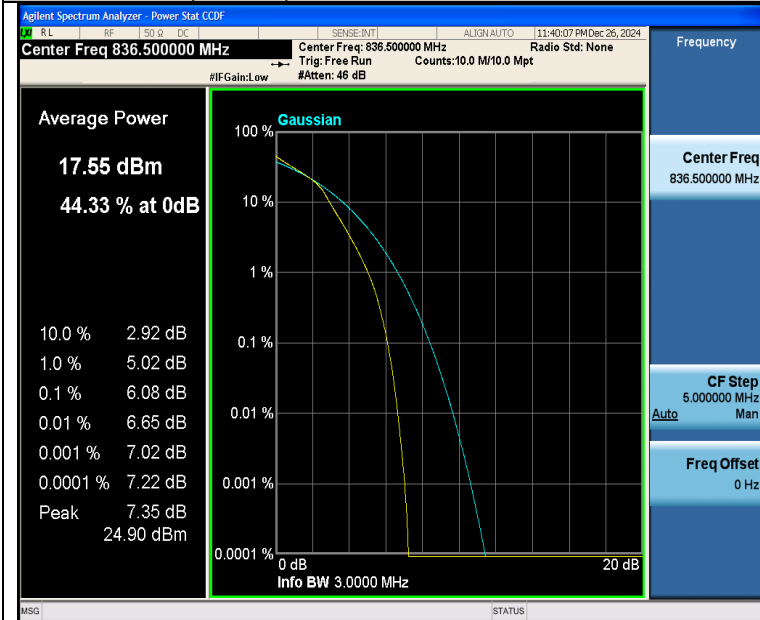
Band26(824-849)-3MHz-16QAM-26915-15RB#0-PASS
