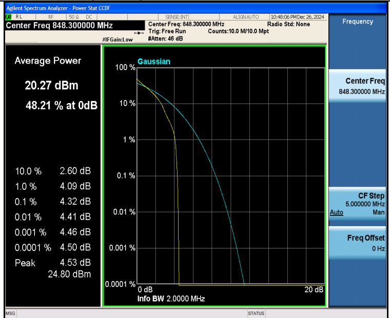
Band26(824-849)-1.4MHz-QPSK-27033-1RB#0-PASS
