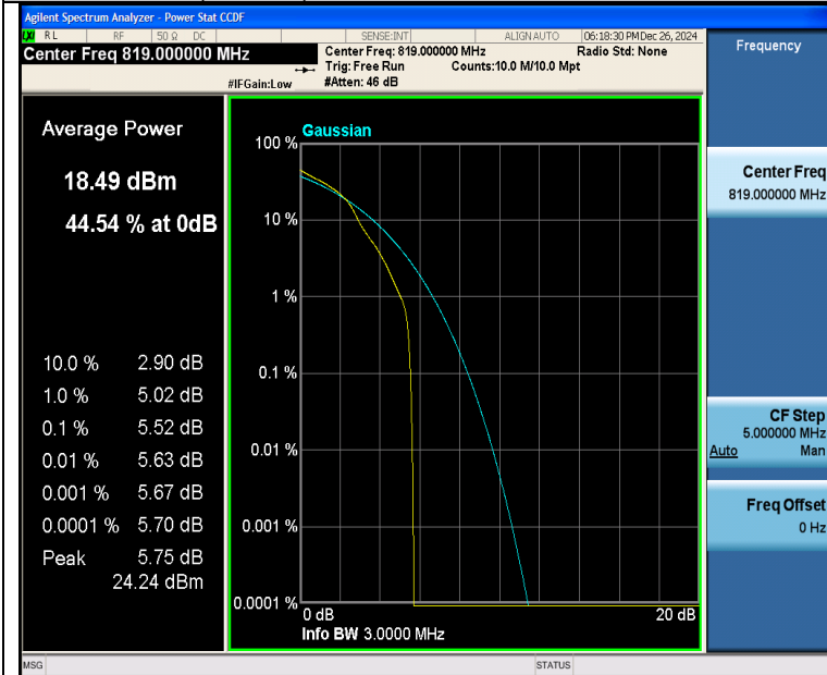
Band26(814-824)-3MHz-16QAM-26740-1RB#0-PASS
