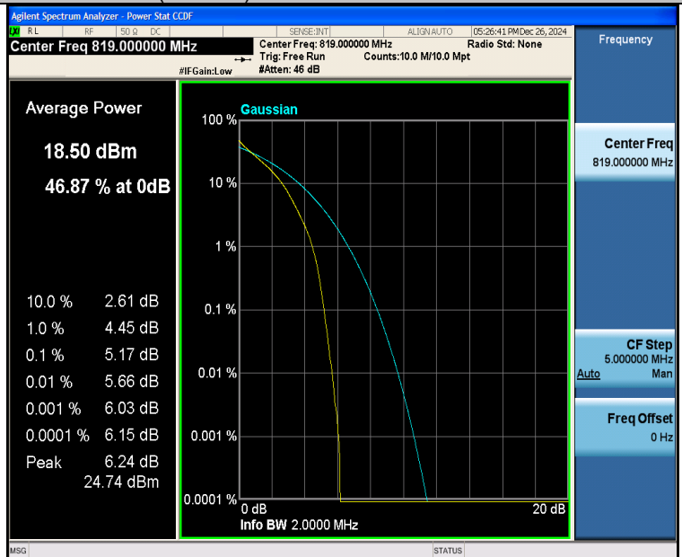
Band26(814-824)-1.4MHz-QPSK-26740-6RB#0-PASS
