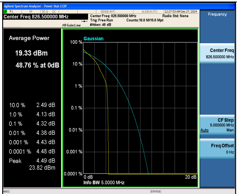
Band26(824-849)-5MHz-QPSK-26815-1RB#0-PASS
