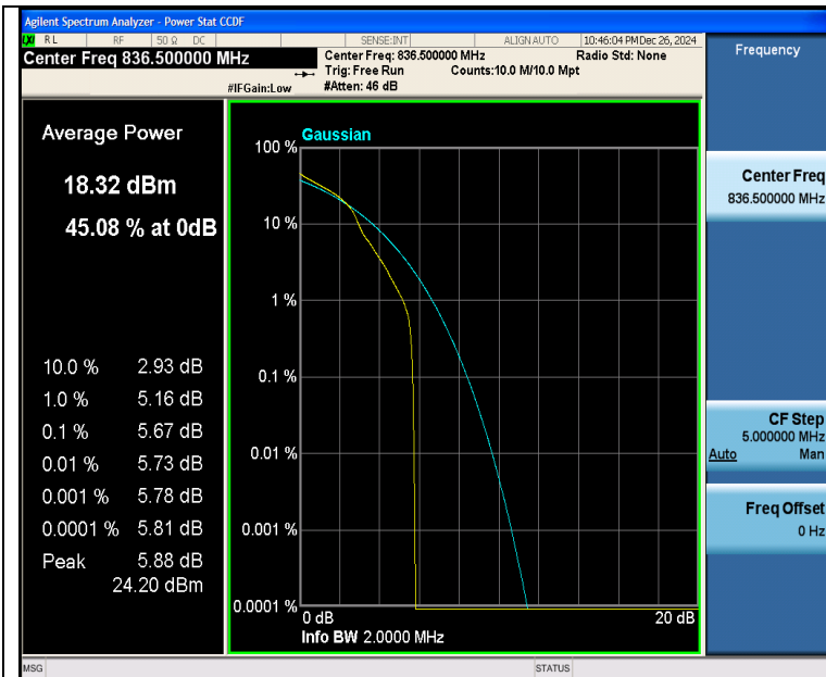
Band26(824-849)-1.4MHz-16QAM-26915-1RB#0-PASS
