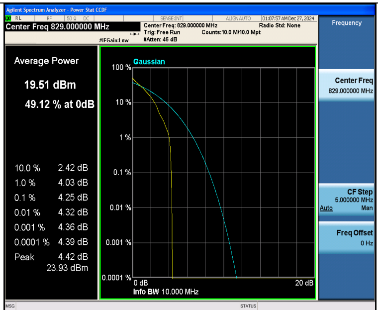
Band26(824-849)-10MHz-QPSK-26840-1RB#0-PASS
