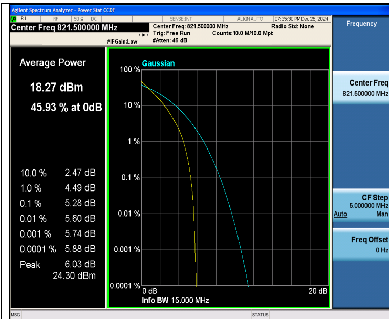
Band26(814-824)-15MHz-QPSK-26765-75RB#0-PASS
