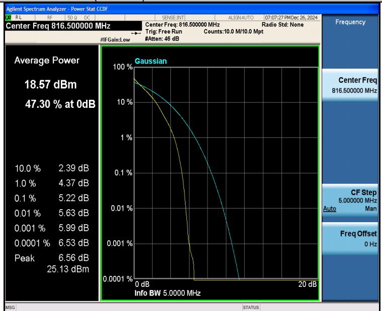
Band26(814-824)-5MHz-QPSK-26715-25RB#0-PASS
