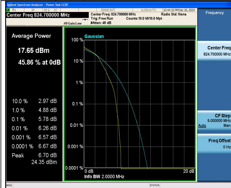
Band26(824-849)-1.4MHz-16QAM-26797-6RB#0-PASS
