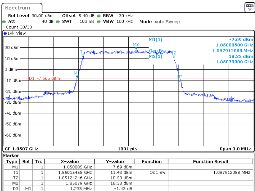
Band25-1.4MHz-QPSK-26047-6RB#0-1.088
