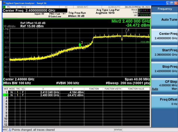
Test Mode:802.11g 2412MHz Chain1
