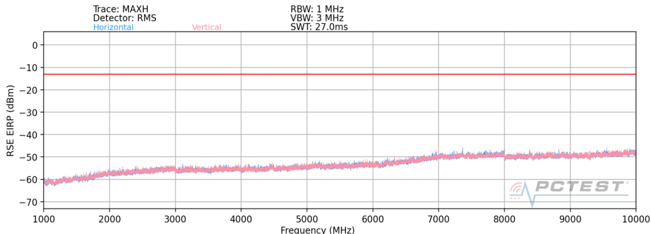
Plot 7-36. Radiated Spurious Plot (LTE Band 8- 15kHz SCS)
