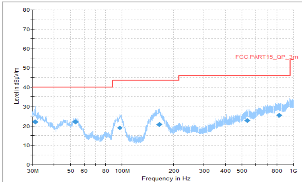
Figure A.1.25. Radiated Emission (GSM receiver 850MHz, 30MHz to 1GHz) Final_Results
