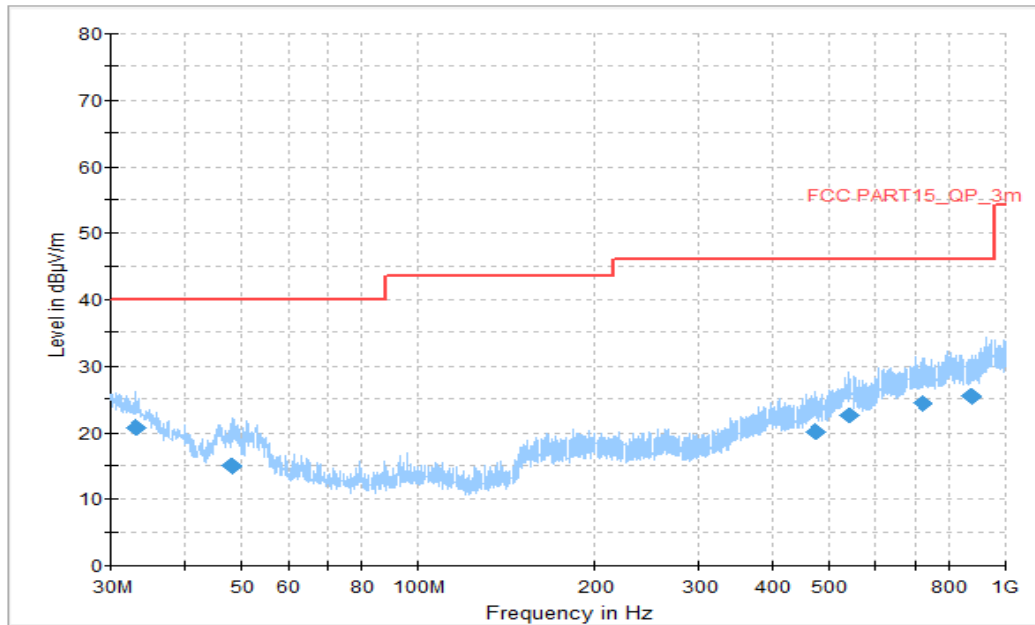
Figure A.1.23. Radiated Emission (GSM receiver 850MHz, 30MHz to 1GHz) Final_Results
