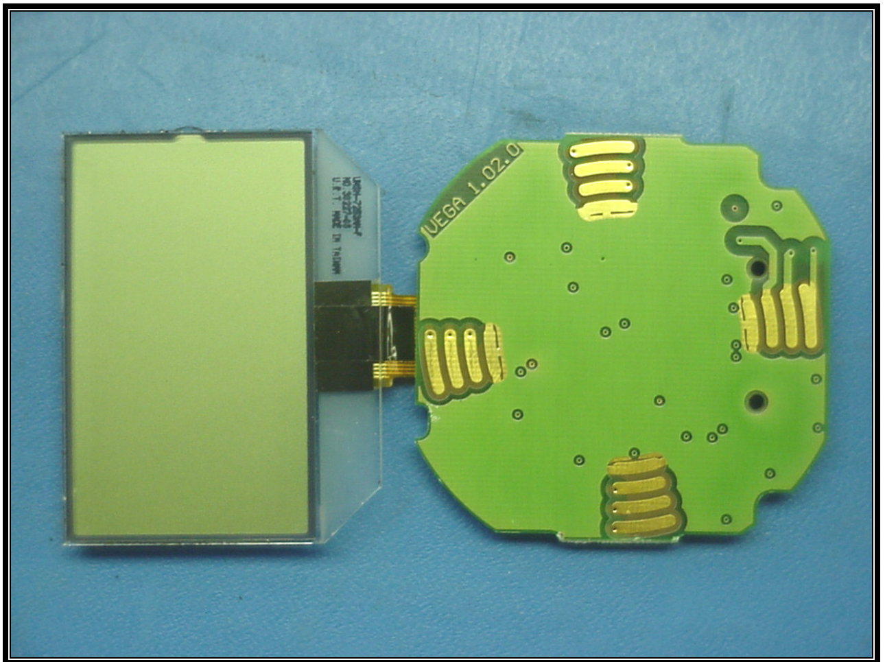
PHOTOGRAPH 21: EUT LCD DISPLAY – PCB BOTTOM VIEW
