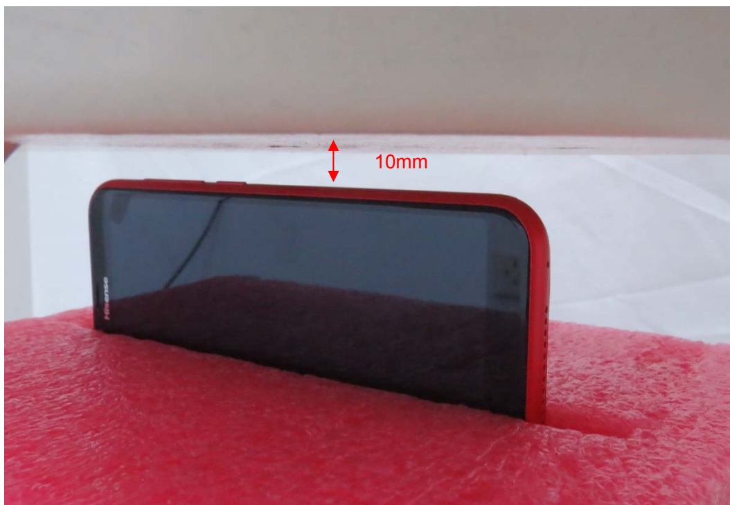
Picture 12: Right Side, the distance from handset to the bottom of the Phantom is 10mm
