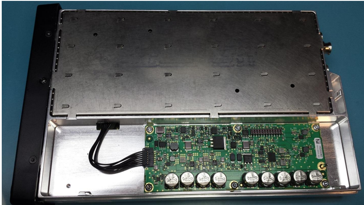
Figure 6 - Power and transmit cavity with TX cover on
