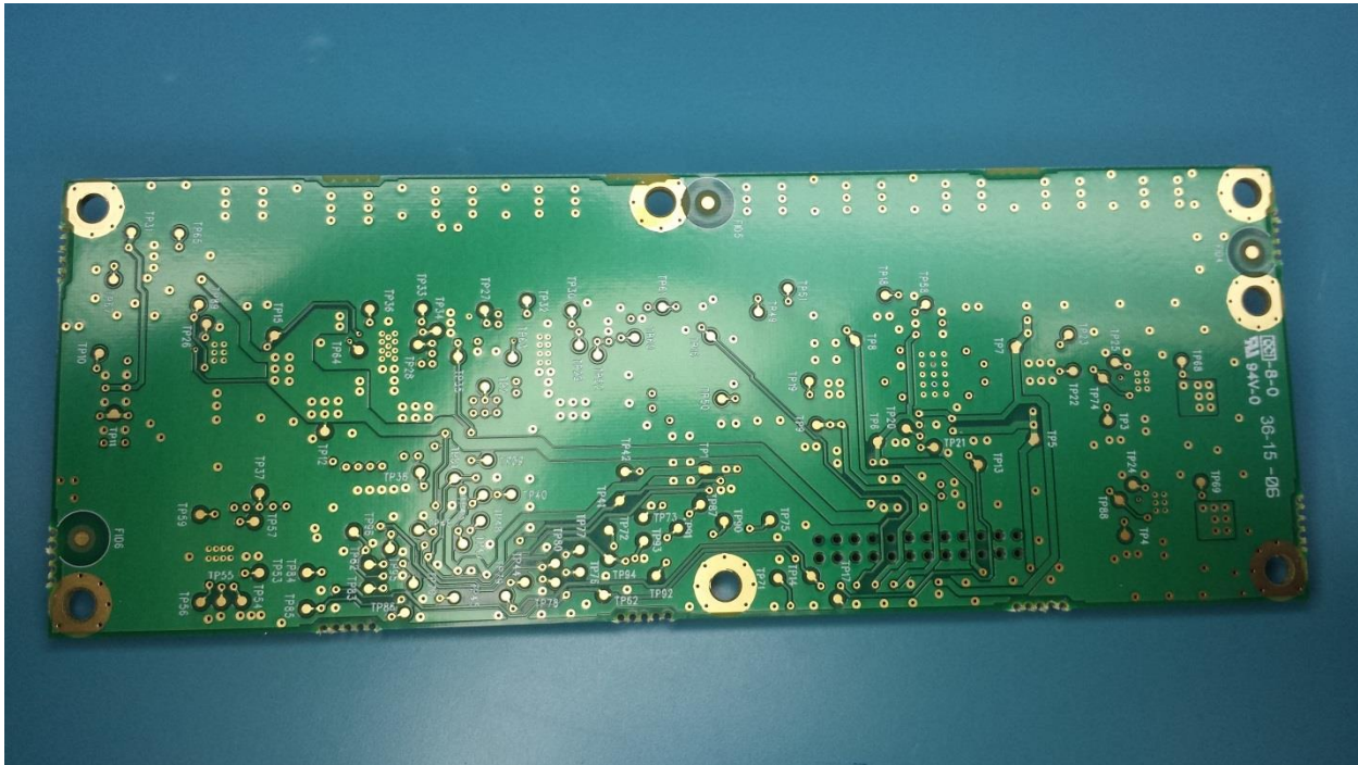
Figure 7 - Power board bottom
