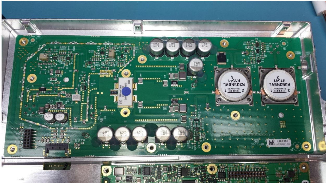
Figure 10 - Transmit board top
