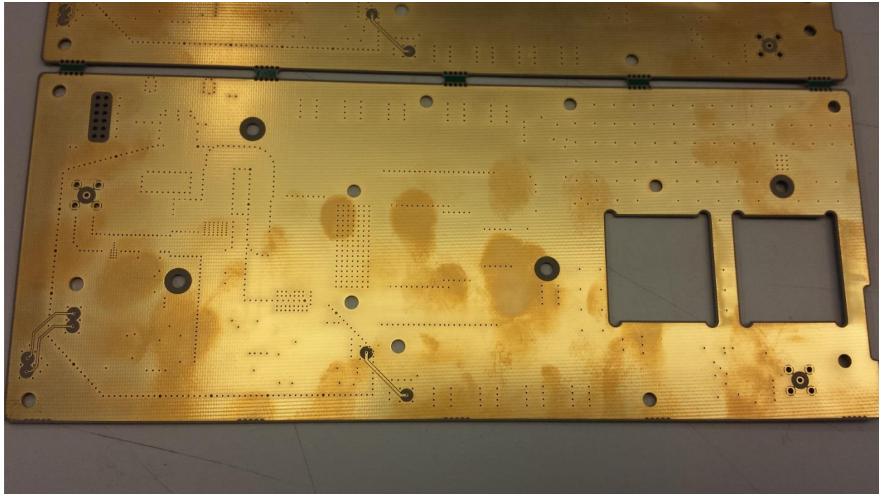
Figure 9 - Power board bottom Transmitter
