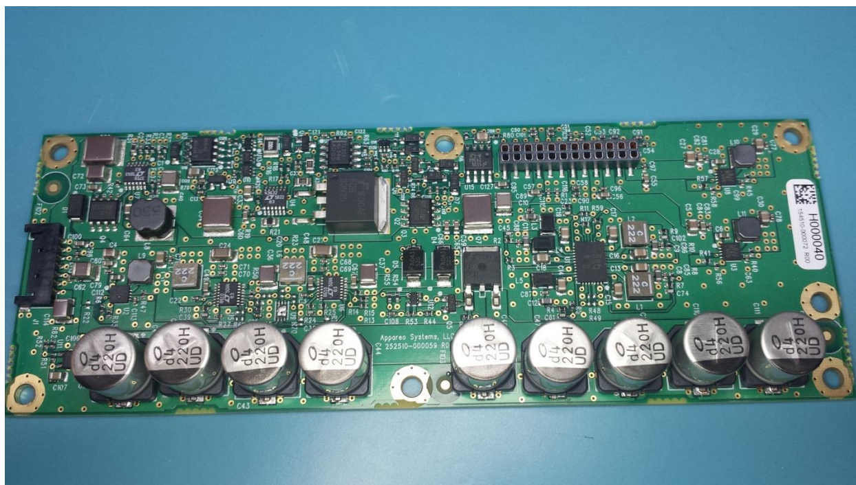
Figure 8 - Power board top
