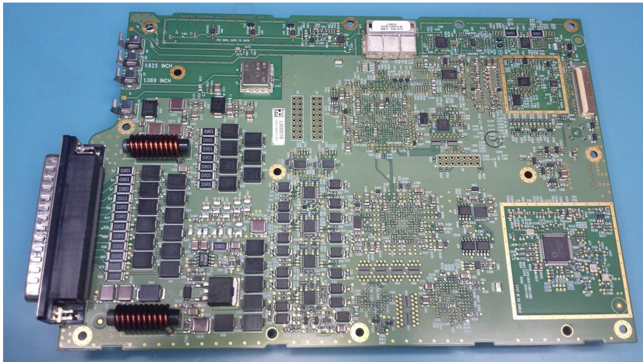
Figure 2 - Main board - top
