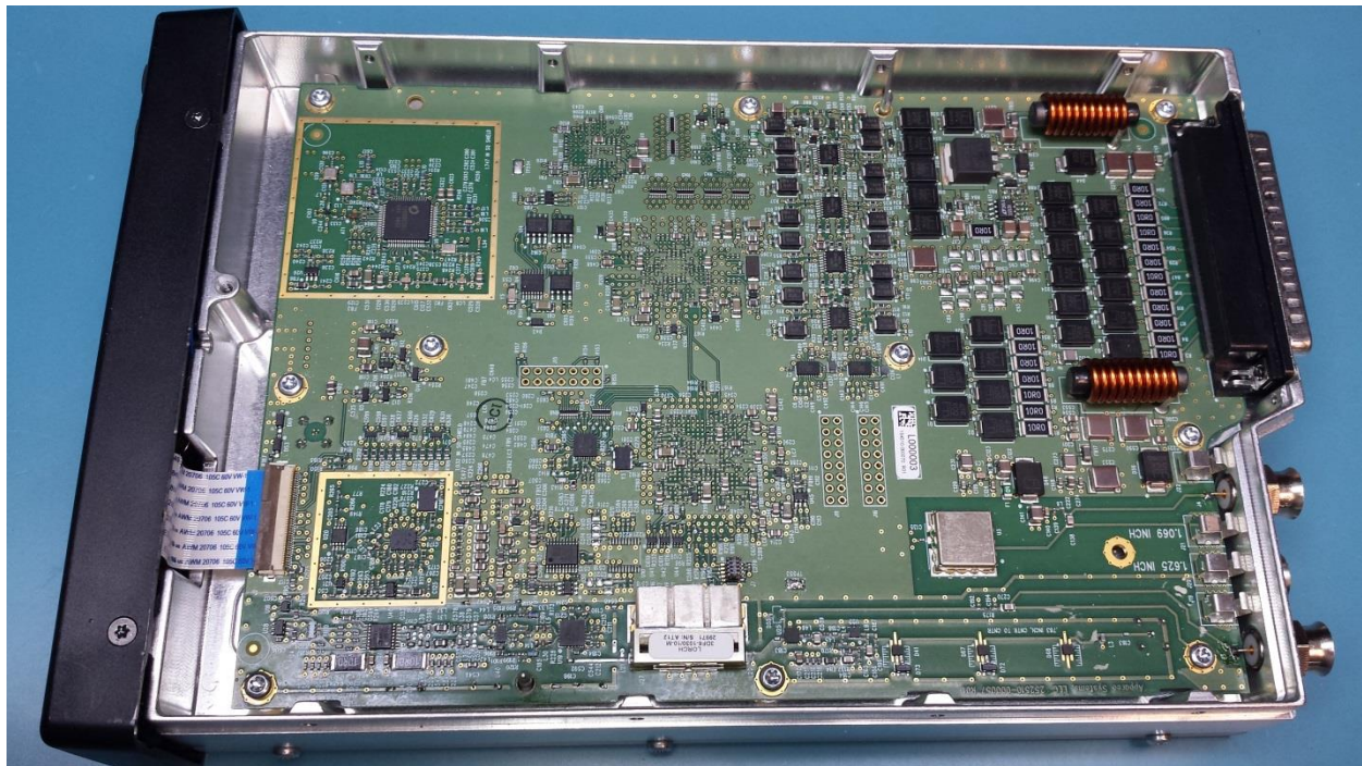
Figure 3 - Main board cavity
