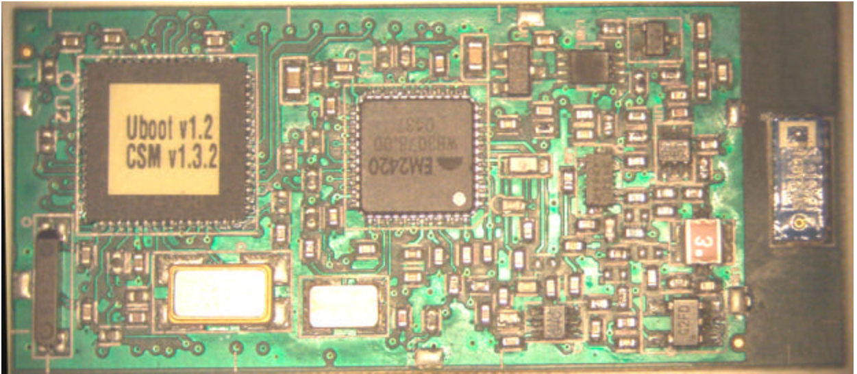
Photo 3. Internal Top View, of EUT
