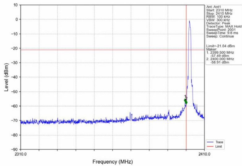
\pi/4 -DQPSK No-hopping Band edge-left side
