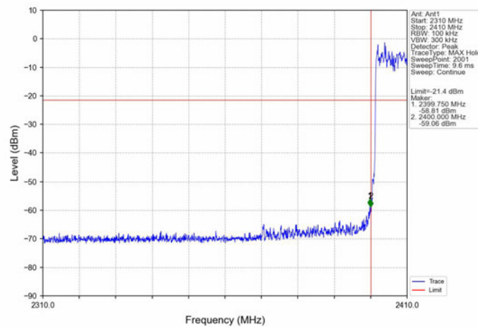
\pi/4 -DQPSK Hopping Band edge-left side
