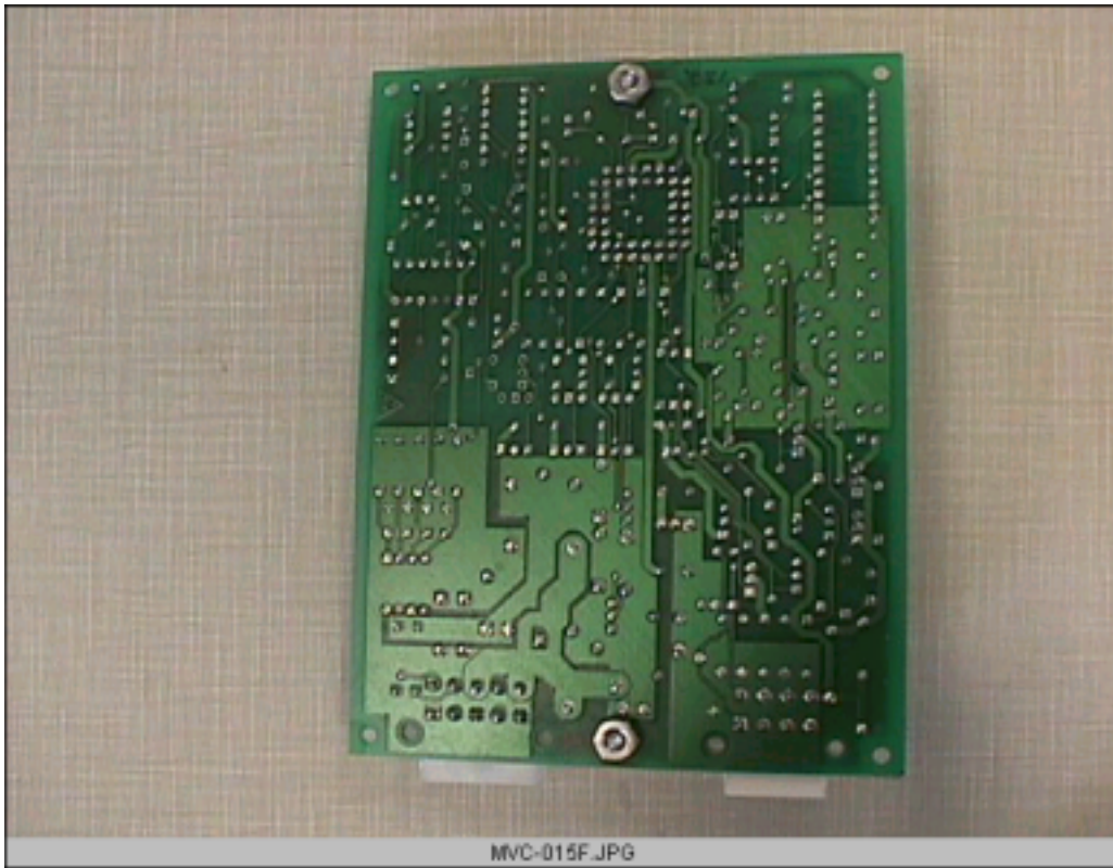
Strattec - Access PCB, Foil Side
