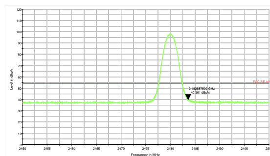
3DH5-Channel 78: Average
