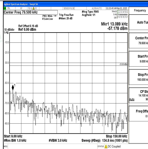
Band13_10MHz_16QAM_23230_1RB#0_0.009~0.15_0.009~0.15
