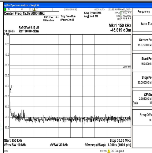
Band13_10MHz_16QAM_23230_1RB#0_0.15~30_0.15~30
