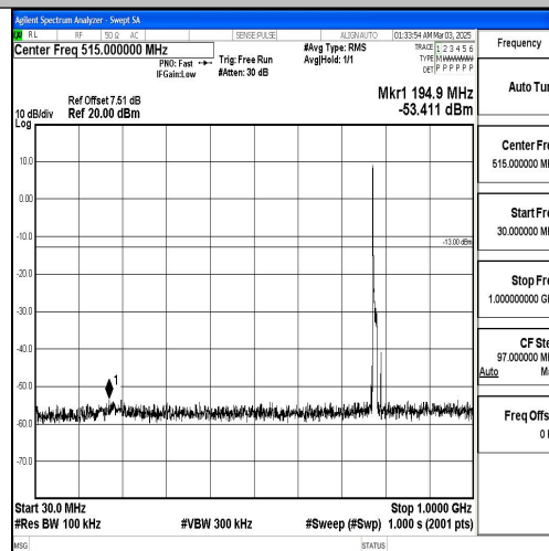
Band13_10MHz_16QAM_23230_1RB#0_30~1000_30~1000
