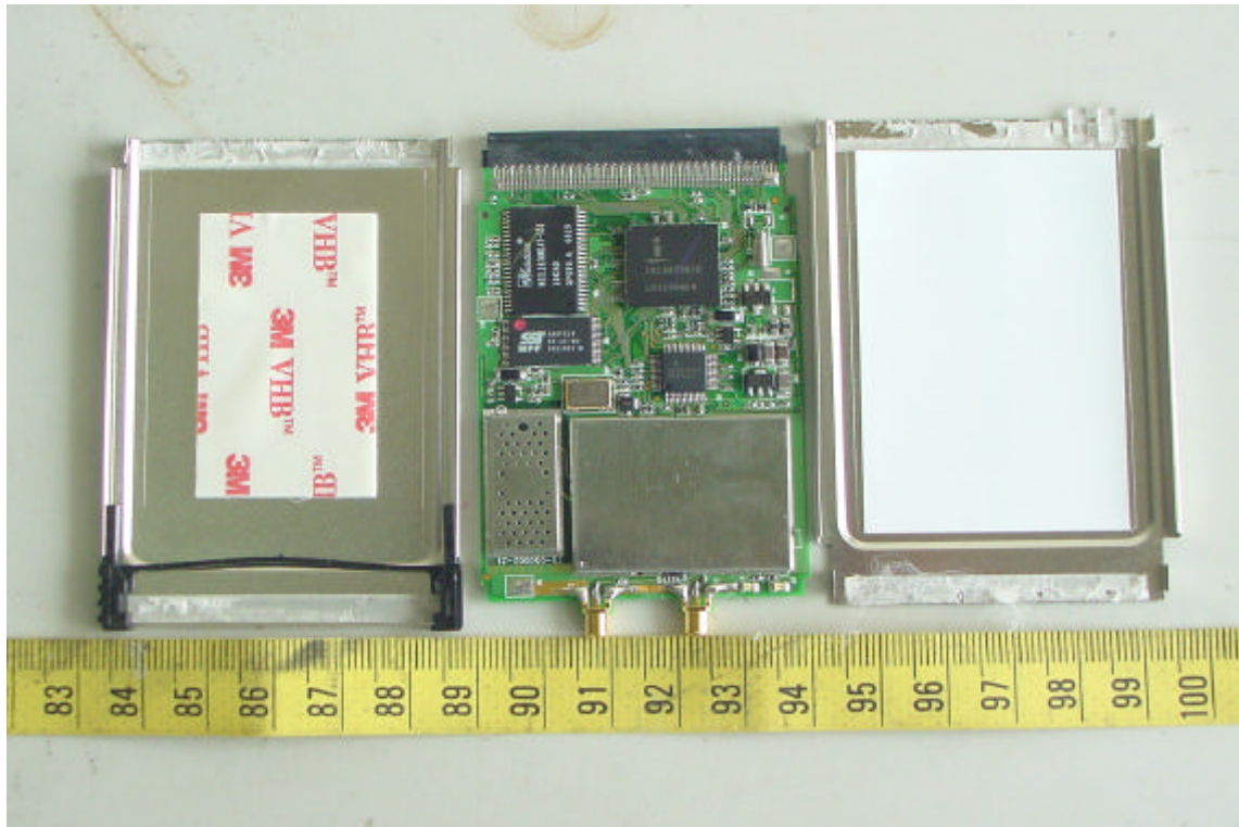
Internal View of Wireless LAN Card
