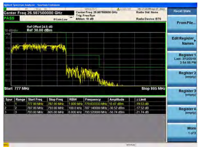
Band13 / 10MHz / High CH / QPSK / FULL RB
