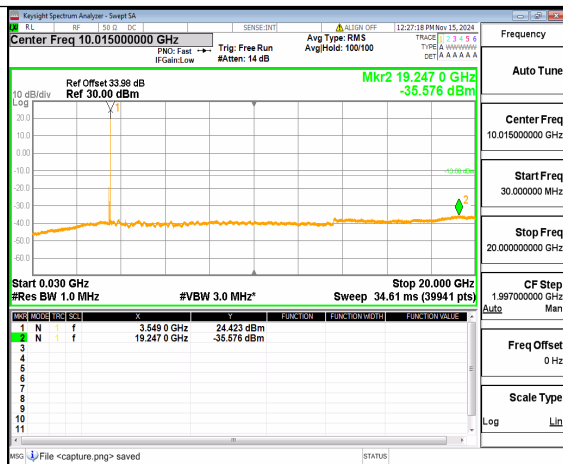
n77(3450-3550MHz) (30MHz-20GHz) 60M DFT-s-OFDM QPSK Inner 1RB Right High
