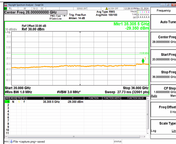
n77(3450-3550MHz) (20GHz-36GHz) 60M DFT-s-OFDM QPSK Inner 1RB Right High
